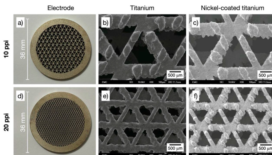
Figure 5. Photographs and SEM images of 3D-printed porous electrodes with triangular open-cell architecture. SEM magnification 30 \times . a) Ti/Ni electrode with porosity grade 10 ppi: b) bare titanium alloy, c) nickel-coated. d) Ti/Ni electrode with porosity grade 20 ppi: e) bare titanium alloy, f) nickel-coated.
