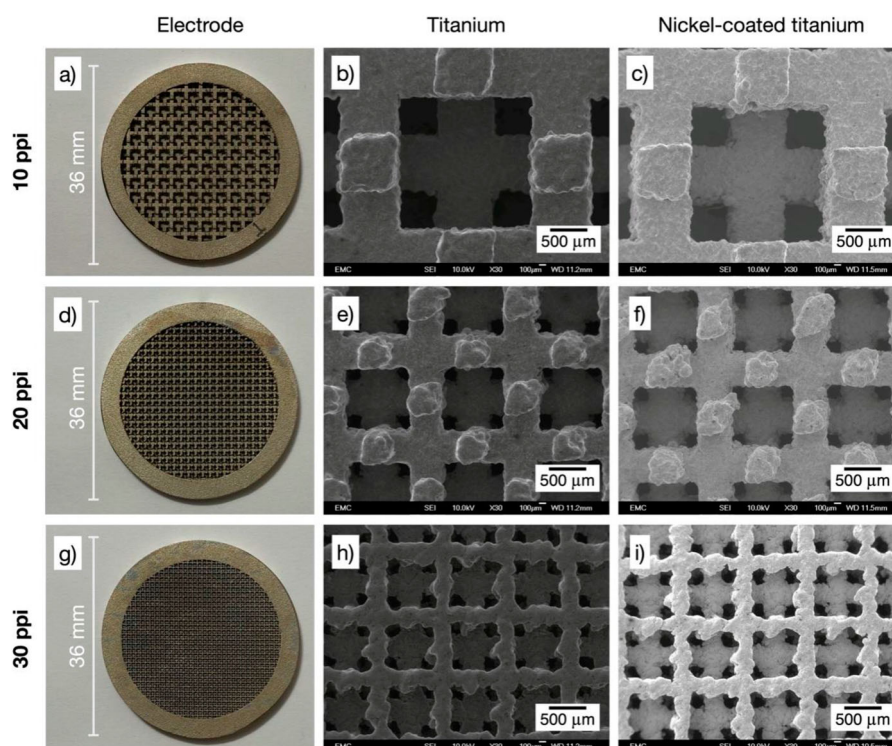
Figure 3. Photographs and SEM images of 3D-printed porous electrodes with rectangular open-cell architecture. SEM magnification 30 \times . a) Ti/Ni electrode with porosity grade 10 ppi: b) bare titanium alloy, c) nickel-coated. d) Ti/Ni electrode with porosity grade 20 ppi: e) bare titanium alloy, f) nickel-coated. g) Ti/Ni electrode with porosity grade 30 ppi: h) bare titanium alloy, i) nickel-coated.
