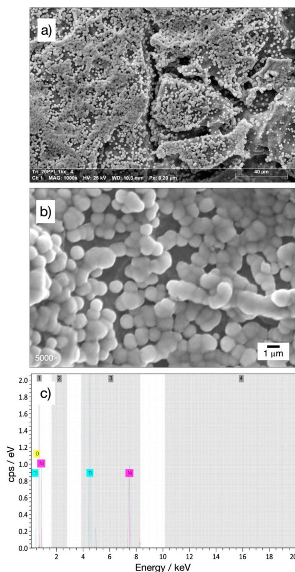
Figure 7. High magnification SEM images and EDS of the nickel coating on the 3D-printed porous electrode with triangular 20 ppi architecture at a mid-point in the porous region. a) 1000 \times image, and c) corresponding EDS spectra. b) Coating microstructure at 5000 \times magnification.
