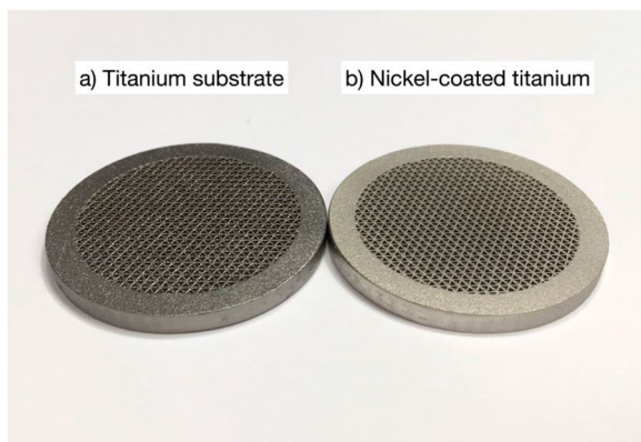
Figure 2. Photographs of the 3D-printed porous electrodes with triangular 20 ppi architecture before and after the coating procedure. a) 3D-printed titanium alloy substrate. b) After nickel electrodeposition.
