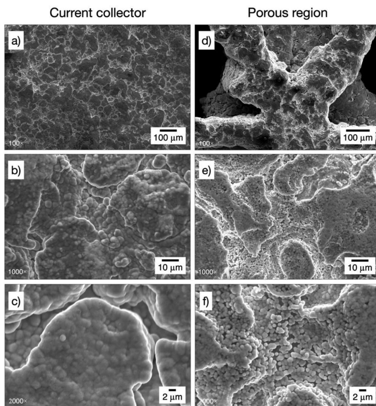
Figure 6. SEM images of the nickel coating on the 3D-printed porous electrode with triangular 20 ppi architecture at different locations and magnifications. At a mid-point in the current collector: a) 100\times , b) 1000\times , c) 2000\times . At a point near the centre of the porous structure of the electrode: d) 100\times , e) 1000\times , f) 2000\times .
