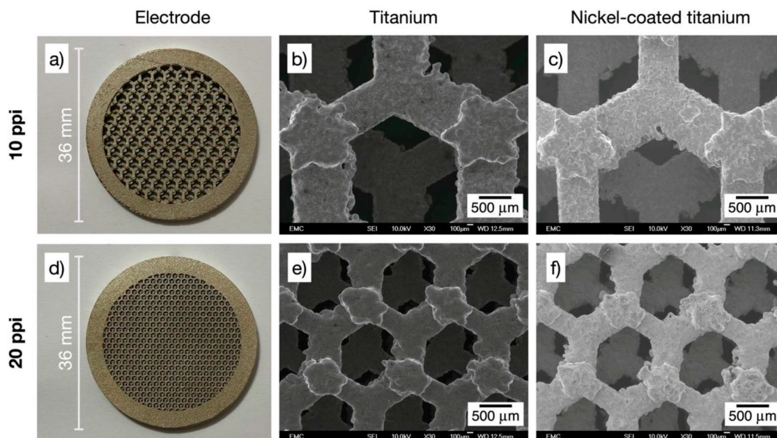
Figure 4. Photographs and SEM images of 3D-printed porous electrodes with hexagonal open-cell architecture. SEM magnification 30 \times . a) Ti/Ni electrode with porosity grade 10 ppi: b) bare titanium alloy, c) nickel-coated. d) Ti/Ni electrode with porosity grade 20 ppi: e) bare titanium alloy, f) nickel-coated.
