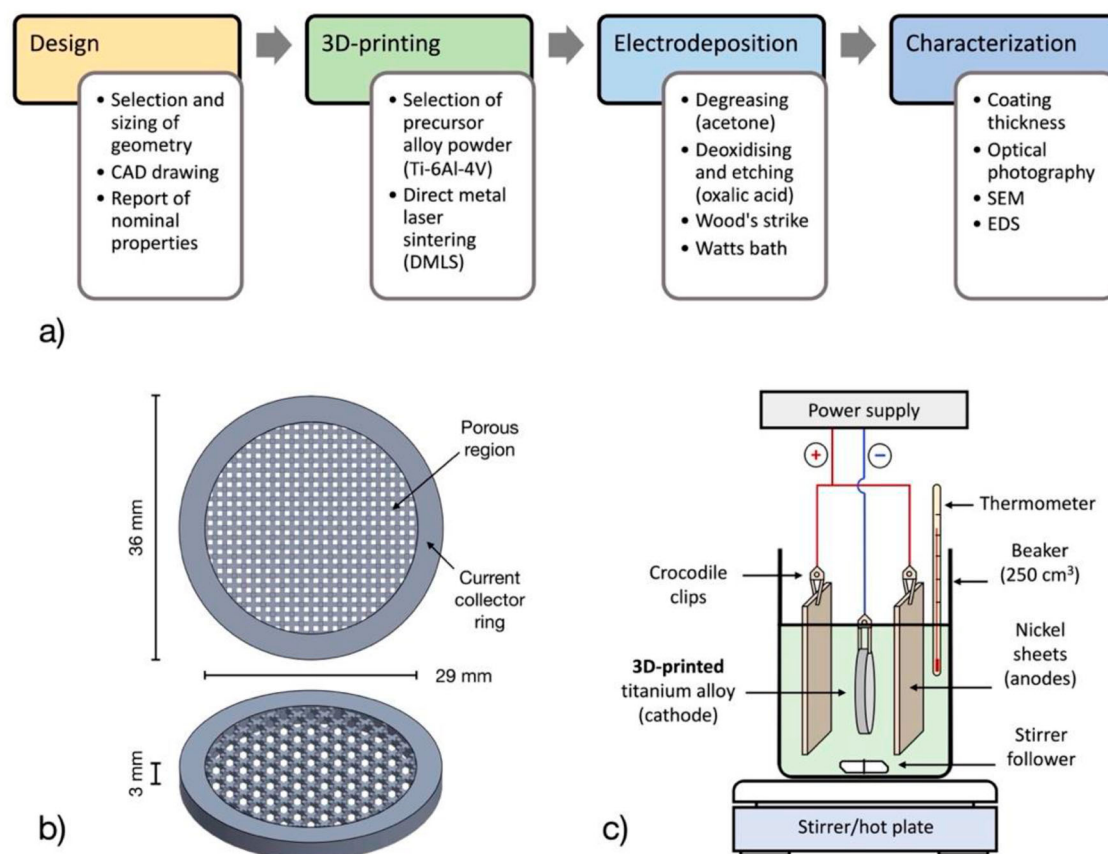
Figure 1. 3D-printed, Ti/Ni porous electrodes for electrochemical flow reactors. a) Design and coating process. b) Configuration of the 3D-printed titanium substrates, front view and perspective (10 ppi rectangular porous architecture as example). c) Experimental arrangement for the electrodeposition of electrocatalytic nickel on titanium substrates.
