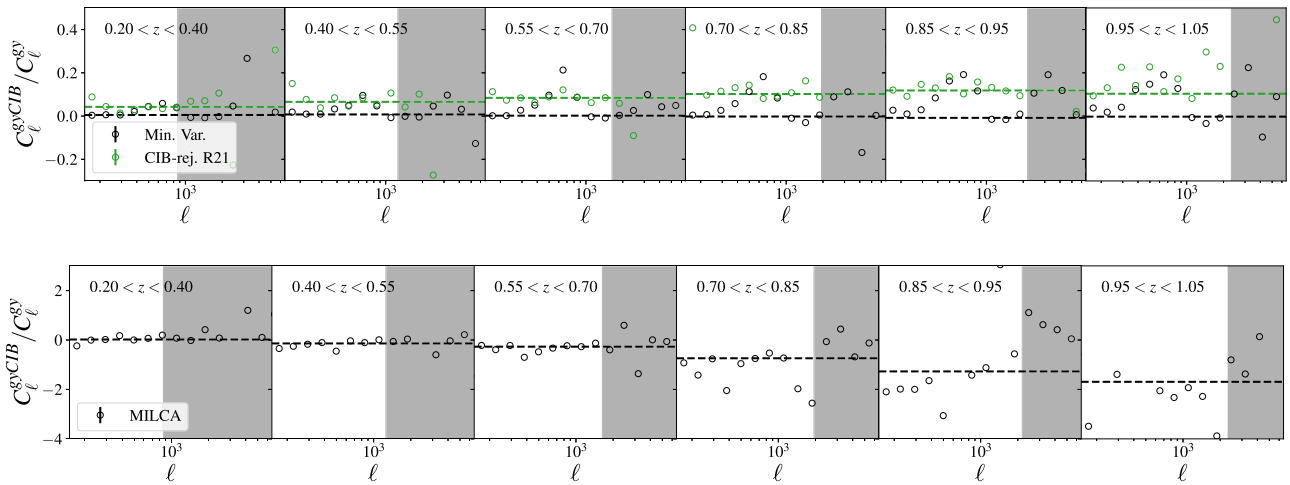
Figure 5. Top panel: Relative CIB leakage in the SPT-SZ + Planck maps, C_{\ell}^{gyCIB}/C_{\ell}^{gy} . The dashed line represents the median ratio within the considered scale cuts. Bottom panel: CIB leakage for MILCA y-map. For the last 2 redshift bins the CIB signal is dominant.
