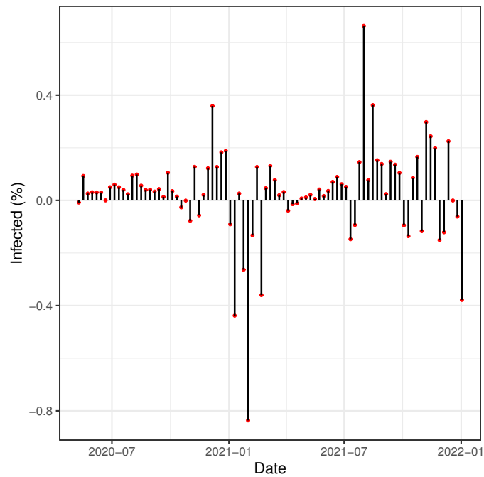
Figure 5: Prediction Error
