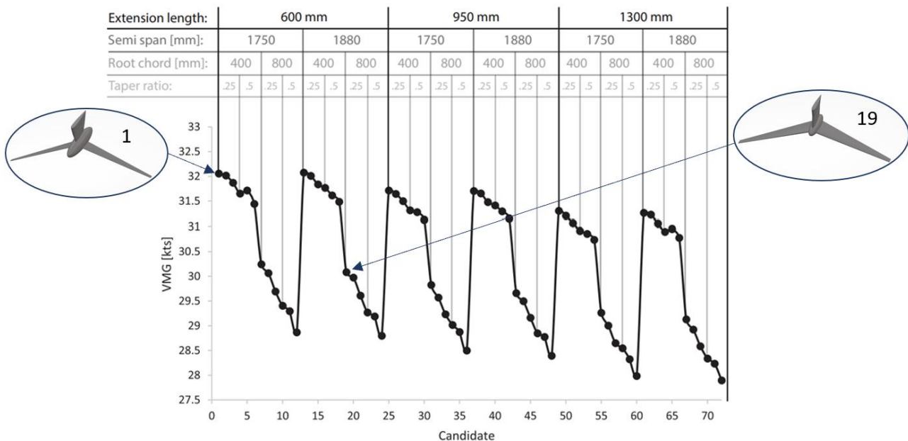
Figure 10. Foil performance in 11 kts downwind at TWA = 140°
