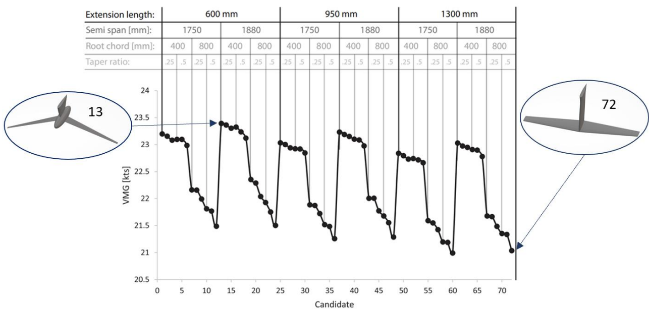
Figure 9. Foil performance in 11 kts upwind at TWA = 47.5°
