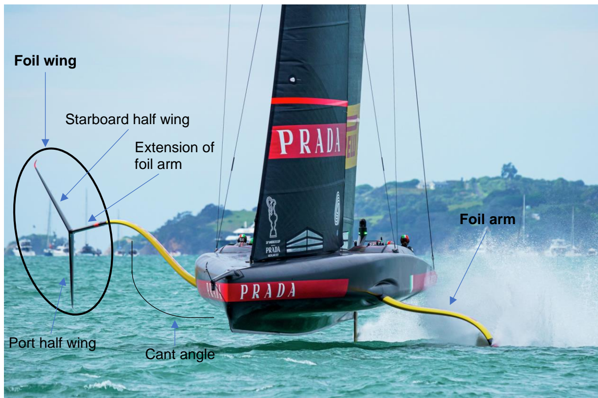
Figure 1. AC75 Luna Rossa based on Gattini (2020)
