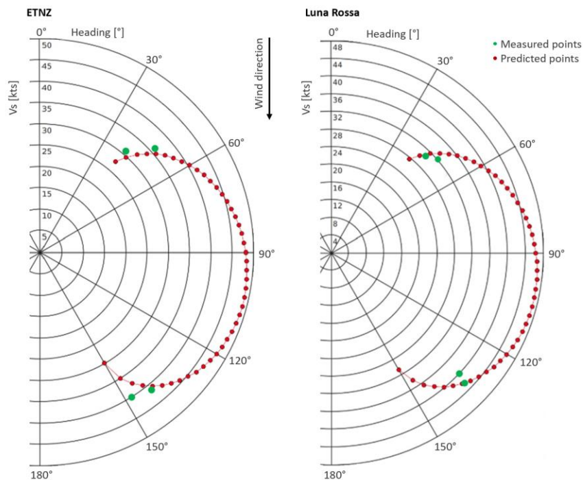
Figure 8. Velocity polars in knots of the two foil designs in 11 kts TWS (ETNZ left, Luna Rossa right)
