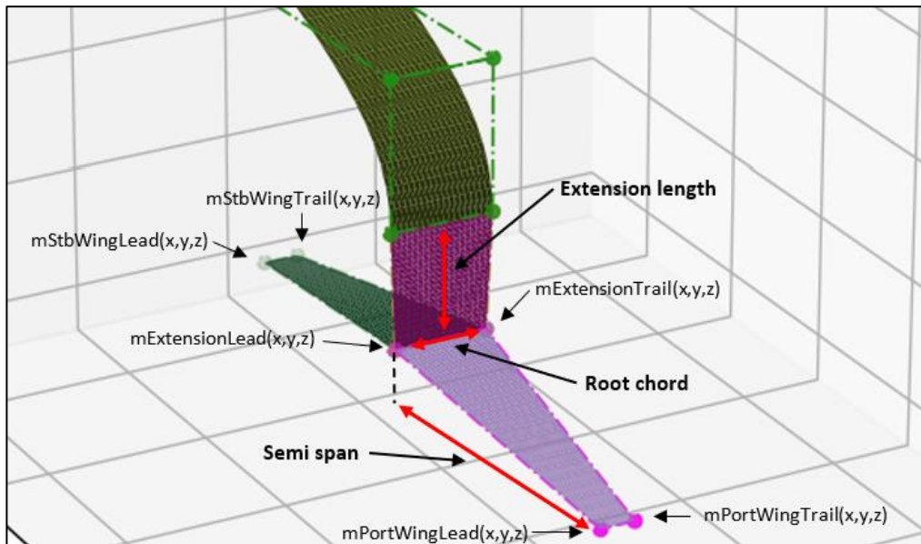
Figure 7. Simple parametric model of the AC75 hydrofoil showing the control points employed to define the hydrofoil geometry
