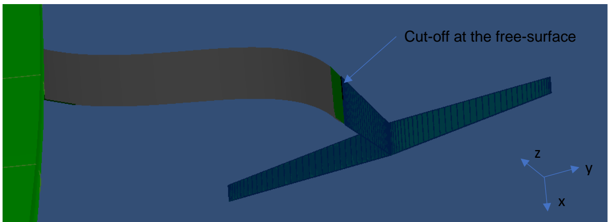
Figure 4. AC75 foil discretised with 40 stations per foil part and cut-off at the free-surface
