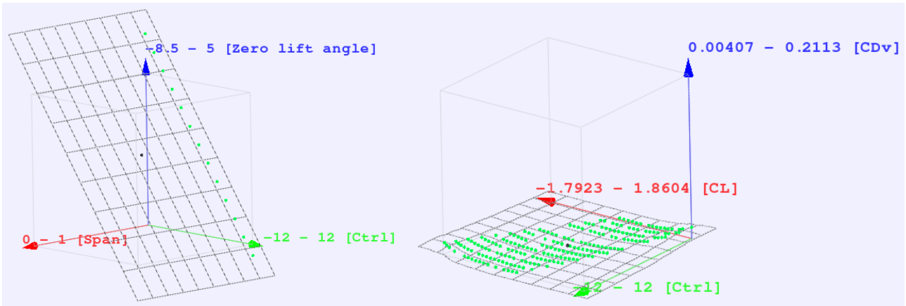
Figure 5. Response surfaces for the Eppler 874 section, zero-lift-angle (left), sectional profile drag C_{Dv} (right) at Re = 3e+07 and Span = 0 ; Ctrl corresponds to flap angle
