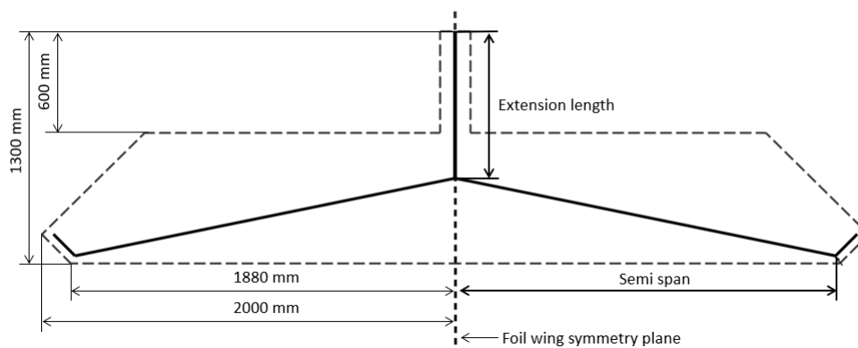
Figure 2. Foil Box
