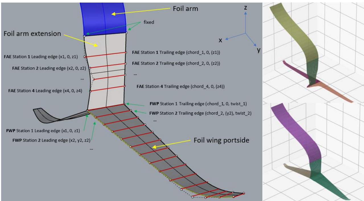
Figure 6. NURBS-based parametric model of the AC75 foil using 86 design
