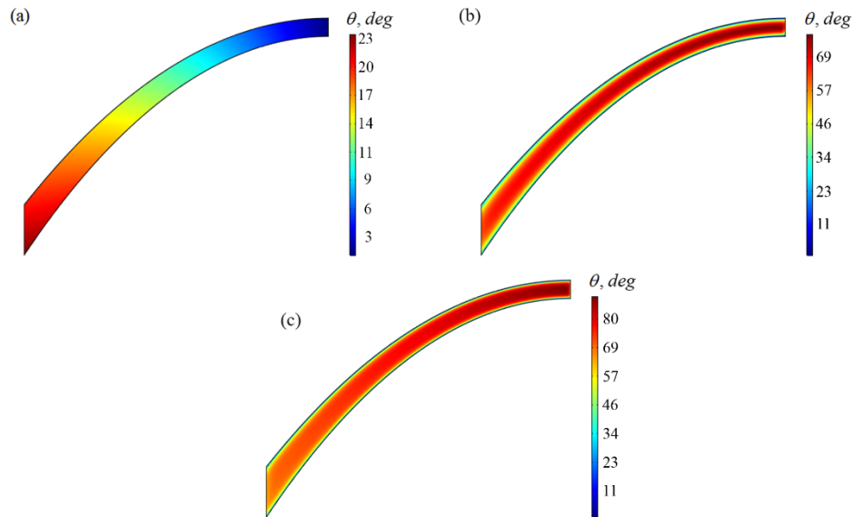
Fig. 5. Director reorientation angle for different applied voltages: (a) 0 \text{ V}_{\text{rms}} ; (b) 1.25 \text{ V}_{\text{rms}} ; (c) 2.5 \text{ V}_{\text{rms}} .
