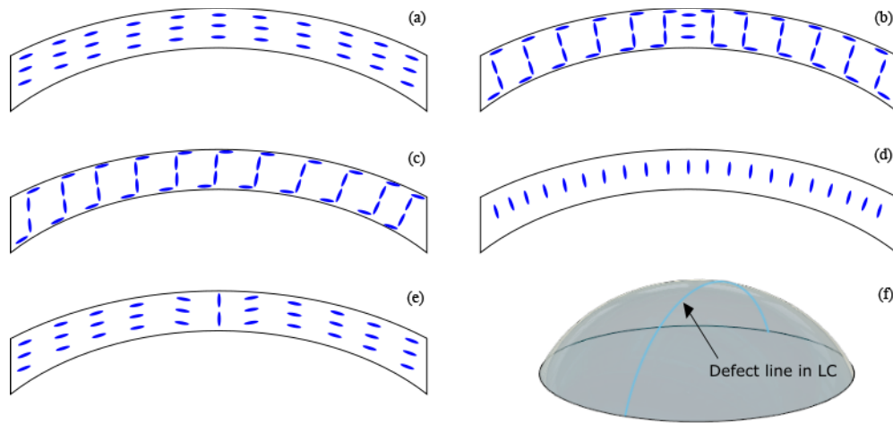
Fig. 4. (a) - Symmetric director distribution at 0 V rms , with orientation governed by boundary conditions. (b) - Symmetric director distribution at 2 V rms containing central defect. (c) - Asymmetric director distribution at 2 V rms . (d) - Lens containing well-oriented liquid crystal without central defect. (e) - Unoriented director distribution containing central defect. (f) - Caricature of optical signature of (e). Note that diagrams (a) to (e) should be regarded as cartoons indicating the basic topology of the calculated configurations, rather than as an accurate representation with particular parameters.
