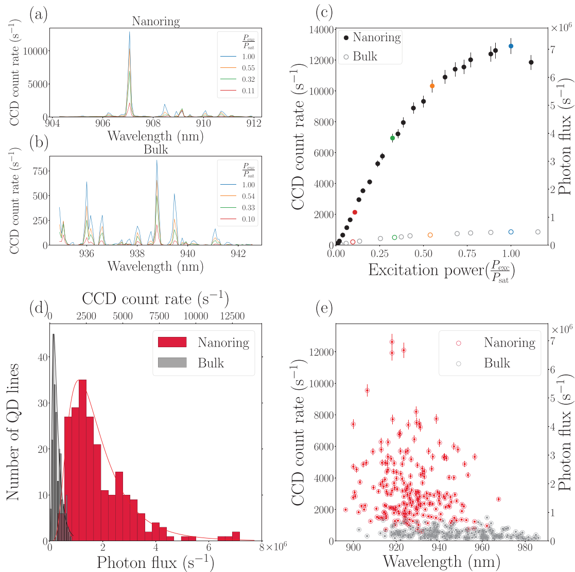
FIG. 3. (a) and (b) Example of photoluminescence spectra, collected at a temperature of about 4 K, on the CCD placed at the exit of the spectrometer, of quantum dots placed within (a) and outside (b) nano-rings, respectively. (c) Photoluminescence intensity of the emission lines with wavelength of 907.06 nm in panel (a) and 938.78 nm in panel (b) (color coded accordingly), as a function of excitation power of a continuous wave 780 nm laser ( P_{exc} ), normalized to the power giving the highest emission count rate for a specific emission line ( P_{sat} = 260 \mu W ). The photon flux corresponds to the number of single photons collected by the objective, once taking into consideration the losses in the collection path and the sensitivity of the detectors (correction factor of 550 \pm 22 ). Error bars represent one standard deviation values due to uncertainty in the loss calibration and are shown when larger than the data point size. (d) Statistics of the collected emission intensity for quantum dots in bulk (outside the nano-rings) and within nano-rings (gray and red histograms, respectively), each composed of about 230 emission lines. The solid lines are lognormal fits to the histograms. (e) Photoluminescence intensity of the emission lines from quantum dots within (red symbols) and outside (gray symbols) metallic nano-rings, plotted as a function of emission wavelength.
