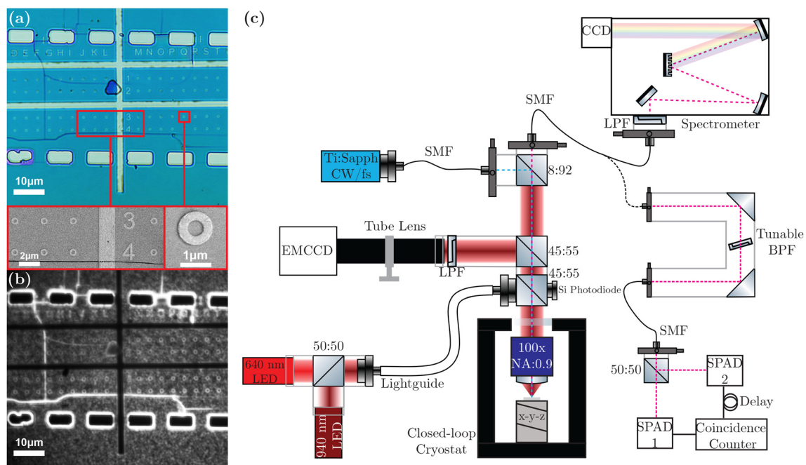
FIG. 2. (a) White-light image of a GaAs membrane (blue area) deposited on an Au layer (pale green areas), with metallic markers and arrays of nano-rings on its surface. The bottom panels show scanning electron micrograph images of the zoomed-in areas delimited by the red rectangles. (b) Photoluminescence image of the same membrane shown in the panel (a), collected under 640 nm-light emitting diode (LED) illumination at a temperature of about 4 K, showing the emission of InAs/GaAs quantum dots. (c) Schematic of the confocal micro-photoluminescence setup (see main text for more details). LPF: long-pass filter, BPF: bandpass filter, SMF: single-mode fiber, SPAD: single-photon avalanche detector, each square with a diagonal line represents a beam splitter whose splitting ratio is shown as reflection: transmission next to it.
