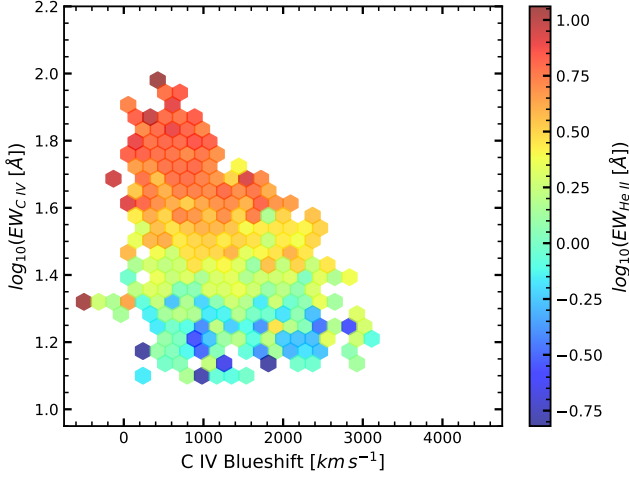
Figure B2. The median observed He II EW in bins of C IV blueshift and C IV EW for the 3.5 < z < 4.0 sample, using line properties derived from Wu & Shen (2022). The He II EW is correlated with C IV EW, however, the He II EW measurements are systematically overestimated when compared to this work. The correlation between the He II EW and the C IV blueshift is also significantly weaker than what is observed in Fig. 8.
