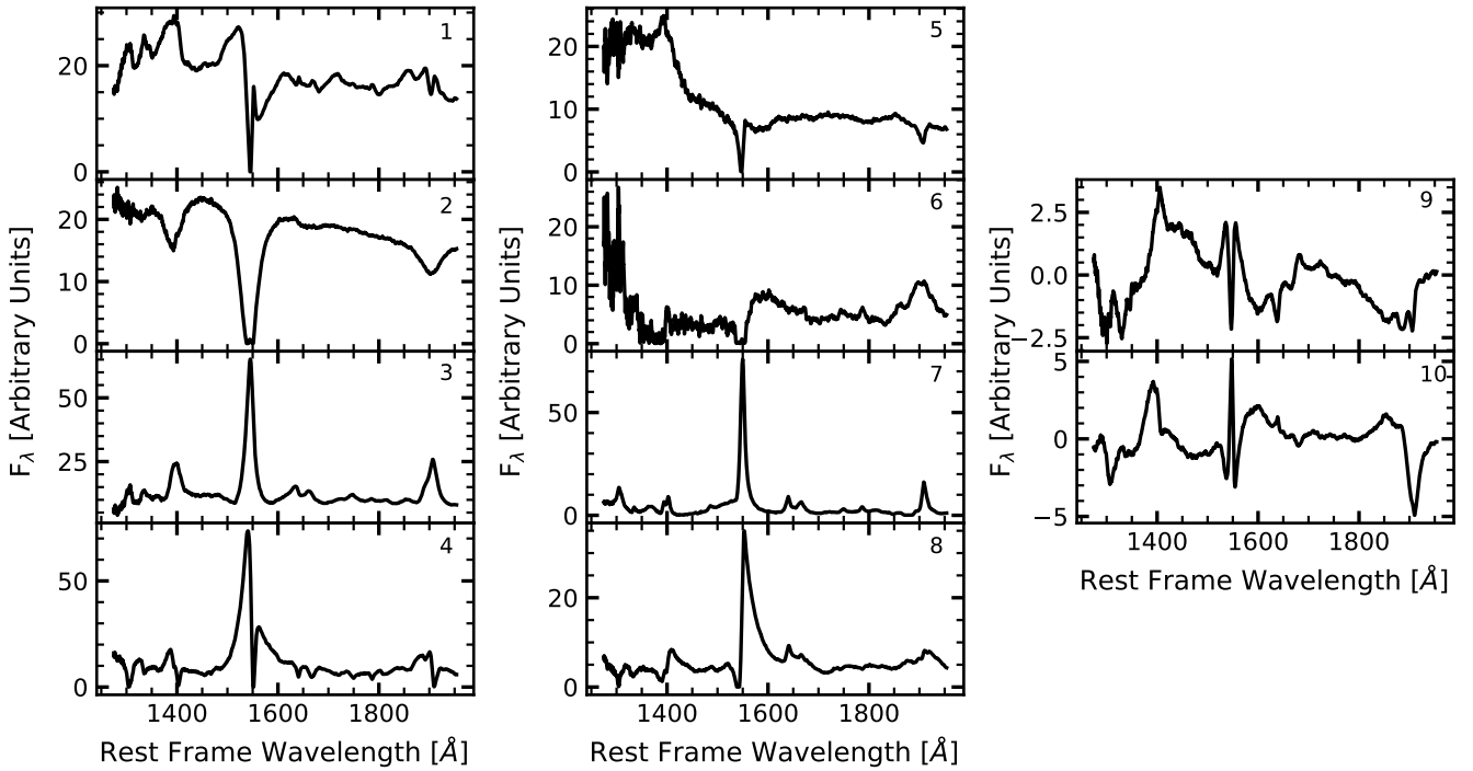
Figure A2. The MFICA components, generated using the technique described in Allen et al. (2013) , used to reconstruct quasar spectra whose 20 < C\text{IV EW} < 70\text{\AA} . Components "9" and "10" are correction components and are therefore permitted to have negative weights in the MCMC fitting.
