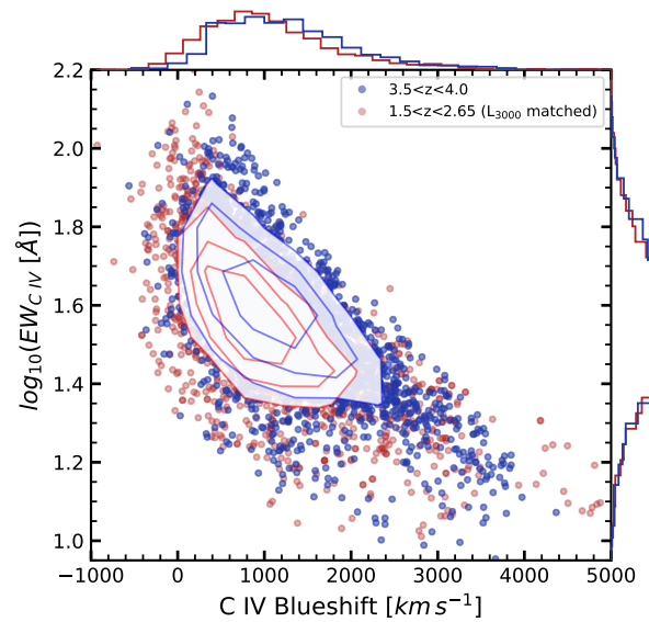
Figure 5. The C iv emission space for the 3.5 < z < 4.0 sample (blue) and the L_{3000} matched 1.5 < z < 2.65 quasars (red) from Temple et al. (2023) . Density contours encircle 68, 50 and 25 per cent of the sample, respectively.
