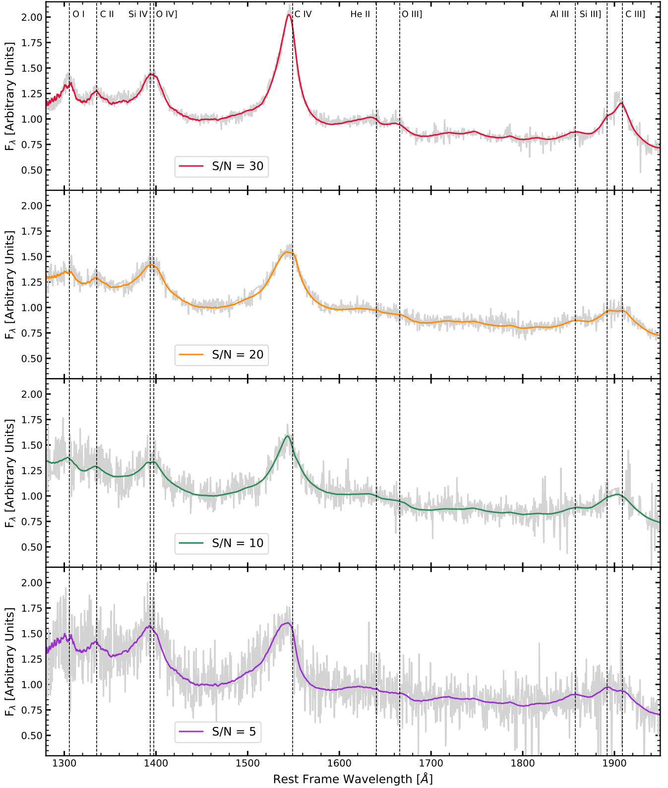
Figure 3. Example quasar spectra from our sample at 3.5 < z < 4.0 with signal-to-noise of 30 (top), 20 (top-middle), 10 (bottom-middle) and 5 (bottom), with their corresponding mean-field independent component analysis reconstructions overlaid. We can see that the MFICA reconstructions have the effect of boosting the signal-to-noise of the SDSS spectra, and hence robust UV emission line analysis becomes achievable.
