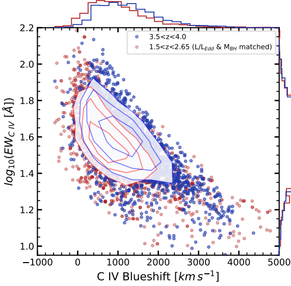
Figure 6. The C IV emission space for the 3.5 < z < 4.0 sample (blue) and the M_{\text{BH}} and L/L_{\text{Edd}} matched 1.5 < z < 2.65 quasars (red) from Temple et al. (2023). Density contours encircle 68, 50 and 25 per cent of the sample, respectively.
