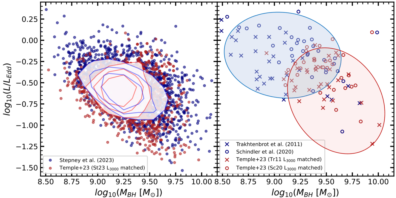
Figure 12. The M_{\text{BH}} - L/L_{\text{Edd}} plane for the 3.5 < z < 4.0 and corresponding UV luminosity matched 1.5 < z < 2.65 samples (left) and the z \sim 6 and corresponding UV luminosity matched 1.5 < z < 2.65 samples (right). Density contours (left) encircle 68, 50 and 25 per cent of the sample, respectively. The cartoon ellipses (right) approximate the locations of the z \sim 6 quasars (blue) and the 1.5 < z < 2.65 quasars, when UV luminosity matched to the z \sim 6 sample (red). When UV luminosity matching the 3.5 < z < 4.0 sample to the 1.5 < z < 2.65 quasars, the samples are consistent in the M_{\text{BH}} - L/L_{\text{Edd}} plane, explaining the results presented in Fig. 5 and Fig. 6. When UV luminosity matching the z \sim 6 sample to the 1.5 < z < 2.65 quasars, we see an inconsistency between the samples in the M_{\text{BH}} - L/L_{\text{Edd}} plane, with the z \sim 6 objects biased towards higher L/L_{\text{Edd}} and lower M_{\text{BH}} than their 1.5 < z < 2.65 counterparts.
