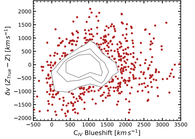
Figure C1. The velocity difference in systemic redshifts between those estimated by Rankine et al. (2020) and calculated using the same recipe and rest-frame wavelength range as this work. This is plotted as a function of the C IV blueshift for a random sample of 1000 1.5 < z < 2.65 quasars of comparable luminosity to the 3.5 < z < 4.0 quasar population. At low C IV blueshifts, the cross-correlation algorithm has a tendency to overestimate the systemic redshift and therefore biases the C IV line centroids blue-ward of their true position.
