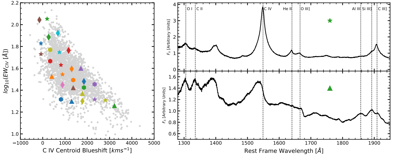
Figure 1. The left-hand panel shows the C IV blueshift versus equivalent width for the 3.5 < z < 4.0 quasar sample with the locations of the 33 high signal-to-noise templates used in the cross-correlation algorithm to calculate systemic redshifts. The spectra for templates at the extremes of the C IV emission space are also presented on the right. The high C IV EW and low C IV blueshift template (top right) features a strong symmetric C IV line profile. Conversely, the low C IV EW and high C IV blueshift template (bottom right) features both a weak and asymmetric C IV line profile and stronger Si III] relative to C III]. Accounting for these systematic changes in the SEDs as a function of the C IV line properties is critical to producing accurate systemic redshifts.
