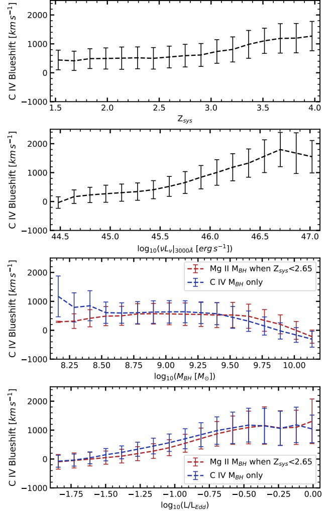
Figure 7. The C IV blueshift as a function of systemic redshift (top), UV continuum luminosity (top-middle), SMBH mass (bottom-middle) and Eddington-scaled accretion rate (bottom). The data is compressed into 17 equidistant bins, where we present the median and median absolute deviation (MAD) of each bin in the appropriate panels. We see a tendency for increasing C IV blueshifts with increasing systemic redshift, UV continuum luminosity and Eddington-scaled accretion rate. The trends with UV continuum luminosity and Eddington-scaled accretion rate can explain why we observe an increase in C IV blueshift as we tend to larger systemic redshifts. There is limited evidence of a strong trend between SMBH mass and C IV blueshift (bottom middle), with a slight tendency to lower C IV blueshifts as we approach the upper limit of our SMBH masses for the sample. There is limited evidence to suggest that the emission line used to estimate virial black hole masses will have any significant impact on our results.
