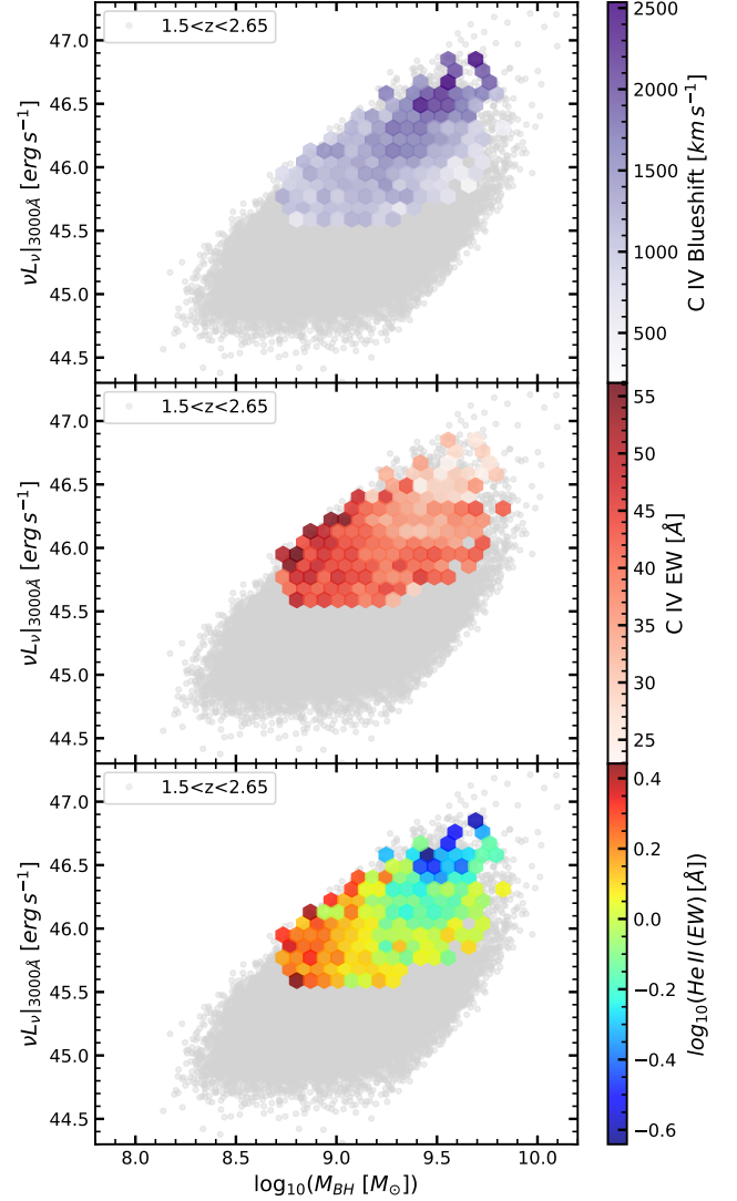
Figure 11. The median observed C IV blueshift (top), C IV EW (middle) and He II EW (bottom) in bins of SMBH mass and 3000\text{\AA} UV continuum luminosity for the 3.5 < z < 4.0 sample overlaid on the M_{\text{BH}} - L_{3000} plane at 1.5 < z < 2.65 (grey, Temple et al. 2023). A clear flux limit is observed at \nu L_{\nu}|_{3000\text{\AA}} \sim 45.5 \text{ erg s}^{-1} in the 3.5 < z < 4.0 sample. Apart from that the 1.5 < z < 2.65 and 3.5 < z < 4.0 samples are well-matched in this space. Below \sim 10^9 M_{\odot} the quasars have stronger UV emission lines and smaller C IV blueshifts. Above this threshold, the contrary is true.
