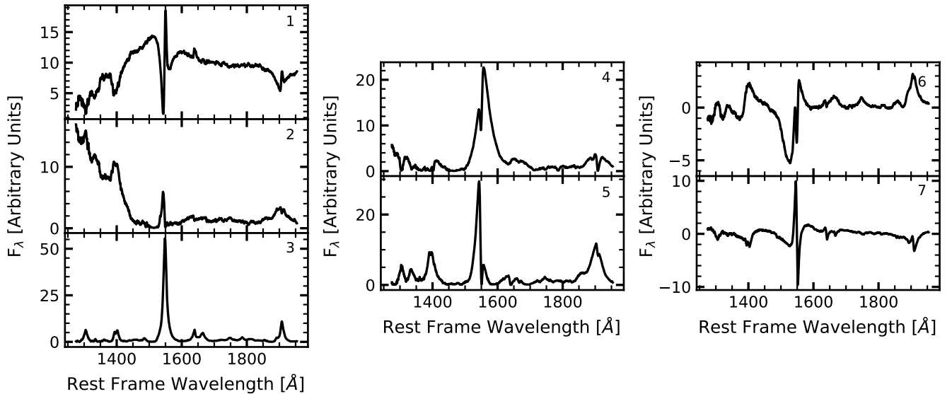
Figure A3. The MFICA components, generated using the technique described in Allen et al. (2013) , used to reconstruct quasar spectra whose C IV EW > 70 Å. Components "6" and "7" are correction components and are therefore permitted to have negative weights in the MCMC fitting.
