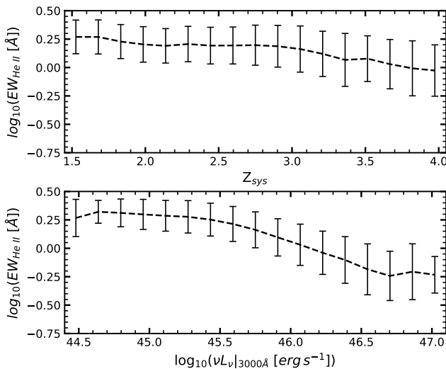
Figure 9. The He II EW as a function of systemic redshift (top) and UV continuum luminosity (bottom). The data is compressed into 17 equidistant bins, where we present the median and median absolute deviation (MAD) of each bin in the appropriate panels. We see a slight tendency for decreasing He II EWs with increasing systemic redshift. The trends with He II EW and UV continuum luminosity can therefore well explain the apparent evolution with systemic redshift.
