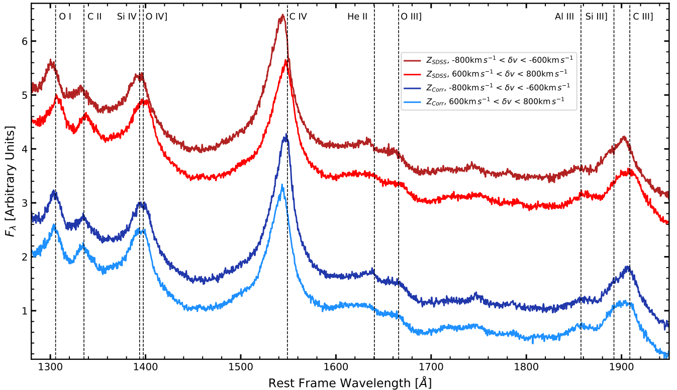
Figure 2. Composites of quasar spectra with redshift corrections -800 \text{ km s}^{-1} < \delta v < -600 \text{ km s}^{-1} or 600 \text{ km s}^{-1} < \delta v < 800 \text{ km s}^{-1} . We present composites before a redshift correction is applied (red) and afterwards (blue). The corrected composites (blue) align with the lower ionisation lines, such as O I, C II, Si IV] and O IV] far more convincingly than when the original SDSS systemic redshifts are used.
