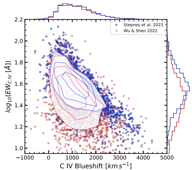
Figure B1. The C IV emission space for the 3.5 < z < 4.0 sample, using line properties derived from Wu & Shen (2022) (red) and this work (blue). C IV blueshifts are calculated from line centroids in both distributions. Density contours encircle 68, 50 and 25 per cent of the sample, respectively. Marginalised distributions of the C IV blueshift and EW are also shown. The distributions do not feature the same characteristic shape in C IV emission space, with the Wu & Shen (2022) objects biased to lower C IV EW.
