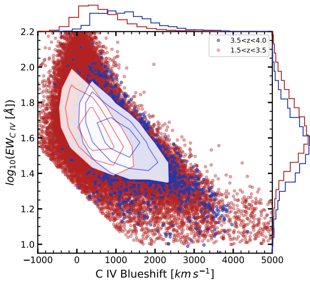
Figure 4. The C iv emission space for both the 1.5 < z < 3.5 (red, Rankine et al. 2020 ; Temple et al. 2023 ) and 3.5 < z < 4.0 (blue) samples. Density contours encircle 68, 50 and 25 per cent of the sample, respectively. Marginalised distributions of the C iv blueshift and EW are also shown. While the distributions feature the same characteristic shape, the 3.5 < z < 4.0 sample is biased to higher C iv blueshift and lower C iv EW. The following criteria was applied to remove poorly fit spectra from both samples; \log_{10}(\text{C iv EW} [\text{Å}]) < -2.3077 \times 10^{-4} \times \text{C iv blueshift} [\text{km s}^{-1}] + 1.3231 .
