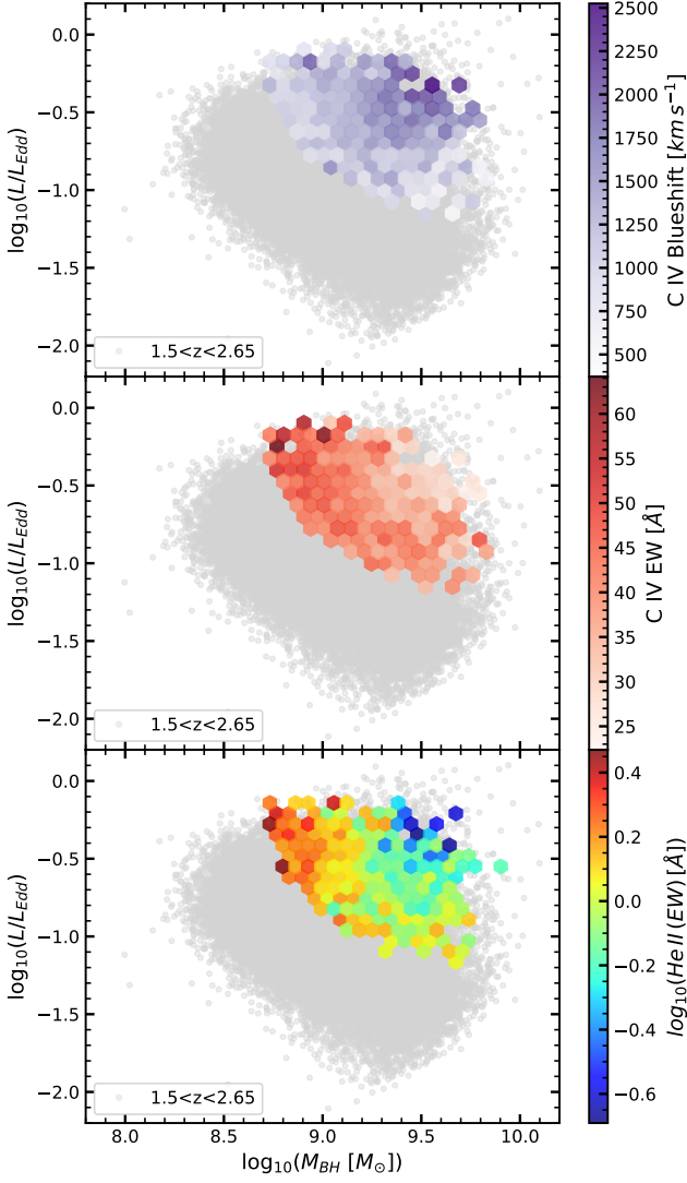
Figure 10. The median observed C IV blueshift (top), C IV EW (middle) and He II EW (bottom) in bins of SMBH mass and Eddington-scaled accretion rate for the 3.5 < z < 4.0 sample overlaid on the M_{\text{BH}} - L/L_{\text{Edd}} plane at 1.5 < z < 2.65 (grey, Temple et al. 2023). Save for a clear flux limit, the 1.5 < z < 2.65 and 3.5 < z < 4.0 samples are well-matched in this space. We note that above L/L_{\text{Edd}} \sim 0.2 there is evidence of a clear trend between He II EW and SMBH mass. Below \sim 10^9 M_{\odot} , the quasars generally have stronger UV emission lines and weaker C IV blueshifts and above this threshold, the contrary is true.
