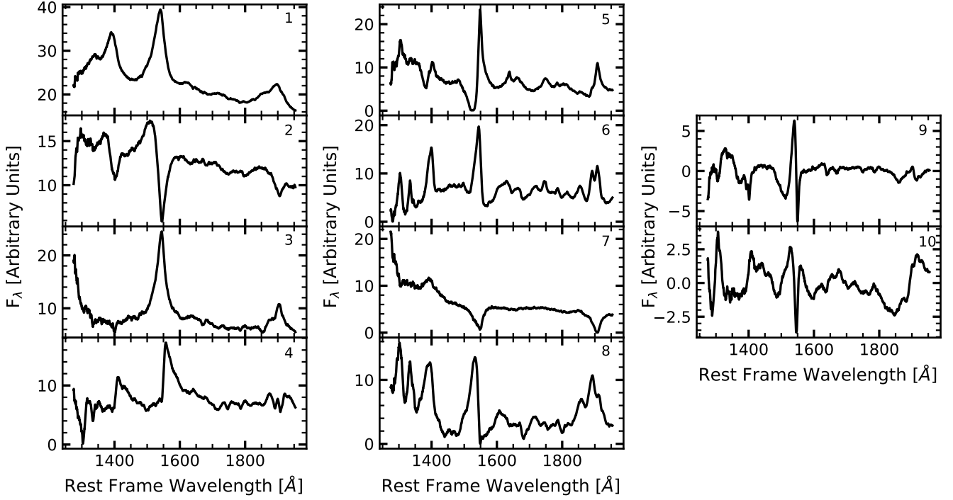
Figure A1. The MFICA components, generated using the technique described in Allen et al. (2013) , used to reconstruct quasar spectra whose C\text{IV EW} < 20\text{\AA} . Components "9" and "10" are correction components and are therefore permitted to have negative weights in the MCMC fitting.
