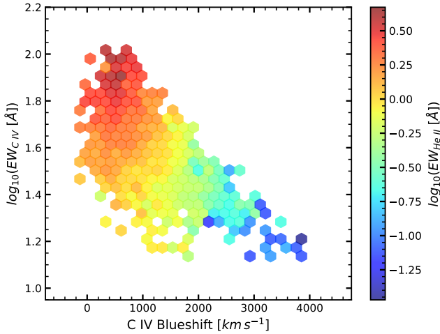
Figure 8. The median observed He II EW in bins of C IV blueshift and C IV EW for the 3.5 < z < 4.0 sample. The He II EW is correlated with both C IV blueshift and C IV EW, with the most blueshifted C IV lines only observed when the He II EW is low. Conversely, the highest EW C IV lines are only observed when the He II EW is high.
