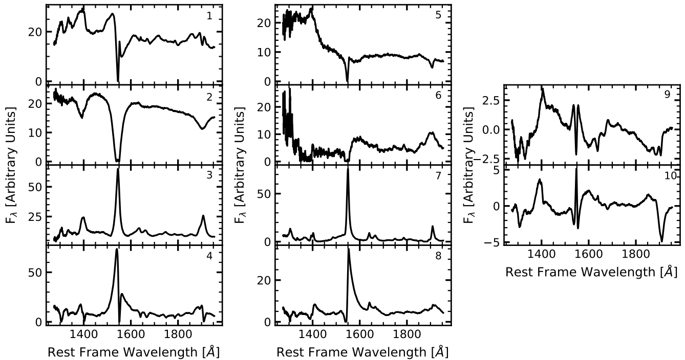
Figure A2. The MFICA components, generated using the technique described in Allen et al. (2013), used to reconstruct quasar spectra whose 20 < \text{C IV EW} < 70 \text{ \AA} . Components "9" and "10" are correction components and are therefore permitted to have negative weights in the MCMC fitting.
