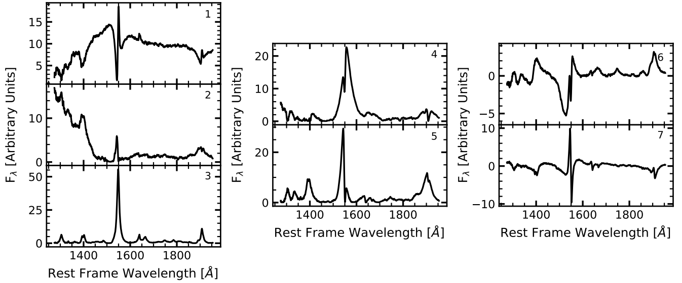
Figure A3. The MFICA components, generated using the technique described in Allen et al. (2013) , used to reconstruct quasar spectra whose C iv EW > 70\text{\AA} . Components "6" and "7" are correction components and are therefore permitted to have negative weights in the MCMC fitting.
