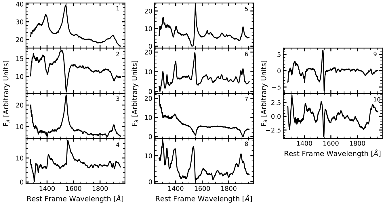
Figure A1. The MFICA components, generated using the technique described in Allen et al. (2013), used to reconstruct quasar spectra whose C IV EW < 20 \text{ \AA} . Components "9" and "10" are correction components and are therefore permitted to have negative weights in the MCMC fitting.
