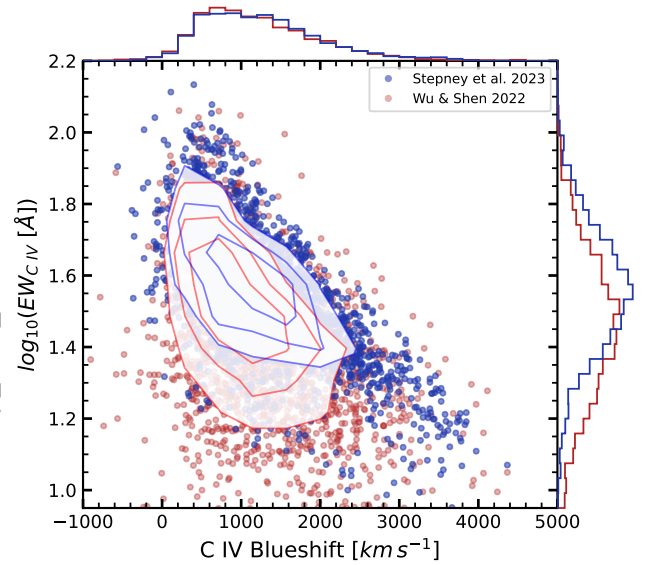
Figure B1. The C iv emission space for the 3.5 < z < 4.0 sample, using line properties derived from Wu & Shen (2022) (red) and this work (blue). C iv blueshifts are calculated from line centroids in both distributions. Density contours encircle 68, 50 and 25 per cent of the sample, respectively. Marginalised distributions of the C iv blueshift and EW are also shown. The distributions do not feature the same characteristic shape in C iv emission space, with the Wu & Shen (2022) objects biased to lower C iv EW.
