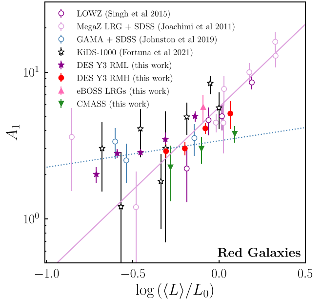
Figure 9. IA strength as a function of k + e -corrected r -band luminosity in red galaxies. By convention, the luminosities are defined relative to a pivot L_0 , which corresponds to an absolute magnitude M_r = -22 . Open points show previous results from the literature (as indicated in the legend). For illustrative purposes we also show two power-law fits from the literature, one fit to GAMA + SDSS at low-mid L (dotted blue), and the other to MegaZ at high L (solid purple). The filled points show our measurements on redMaGiC low- z (stars; five points), redMaGiC high- z (red dots, four points), eBOSS LRGs (pink triangle; one point), and CMASS (green upside down triangles; three points). Note that all results shown here assume the one-parameter NLA model.
