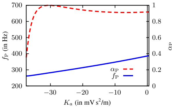
Figure 8. Relationship between the sound absorption maximum properties (frequency f_P and peak absorption \alpha_P ) and the acceleration feedback gain K_a for active MAM absorber configuration B.
