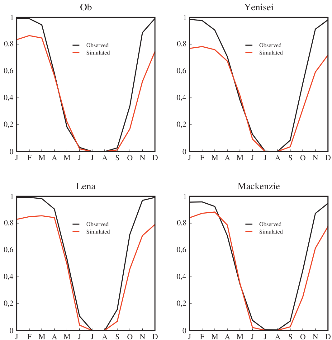
FIG. 6. Comparison between simulated and observed mean annual cycles of snow cover extent over high-latitude basins (expressed in fraction of each basin area).
