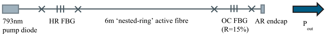
Fig. 3 A typical fibre laser cavity using the nested-ring fibre
