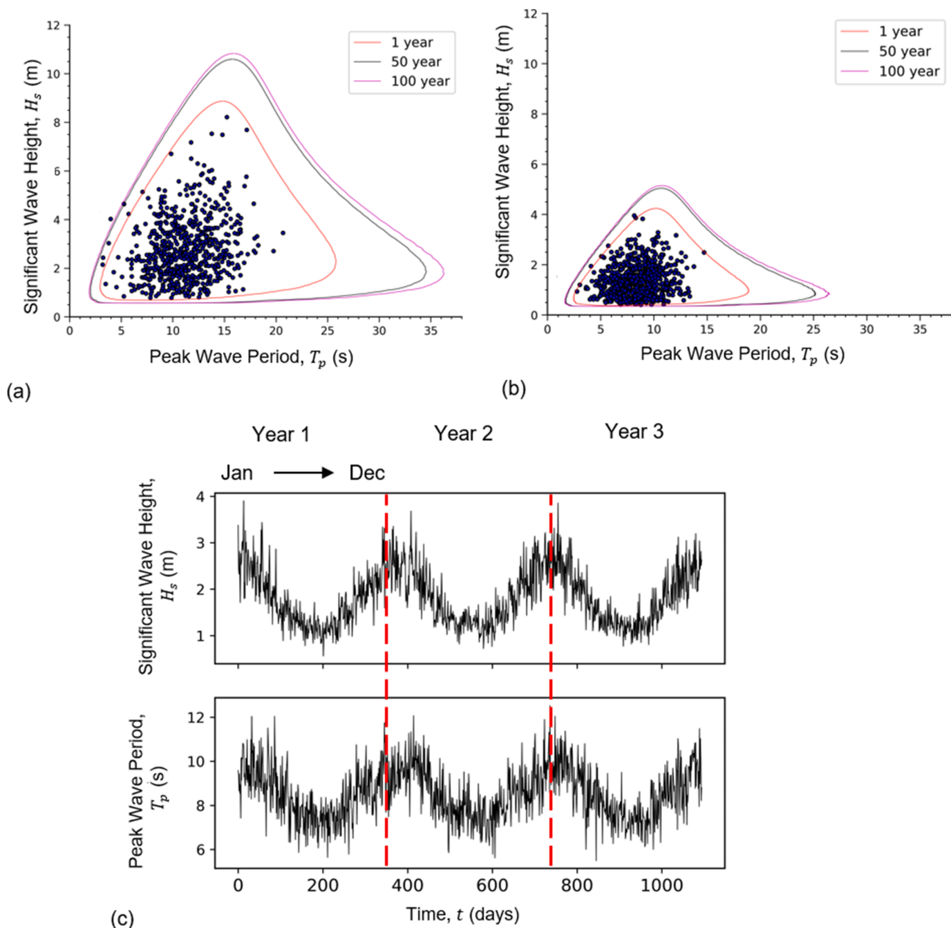
Fig. 5. Monthly seasonal variation in sea states selected during simulations: Typical sea states sampled at (a) the beginning of the year (January), (b) middle of the year (July) and (c) throughout the 3-year simulated time period.
