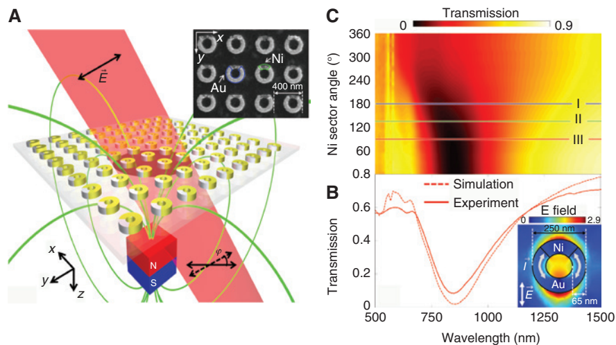
Figure 1: Linear optical properties of bimetallic ring resonator arrays.
