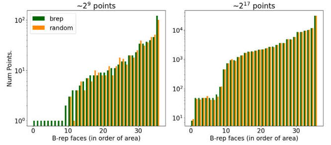
Fig. C.18. Histograms showing the number of points sampled from each b-rep face in a single MFCAD++ example. B-rep faces are sorted in order of surface areas. The distribution resulting in using b-rep stratified sampling and simple random sampling are shown side-by-side for comparison. Two input point cloud sizes are also shown for comparison. (For interpretation of the references to colour in this figure legend, the reader is referred to the web version of this article.)
