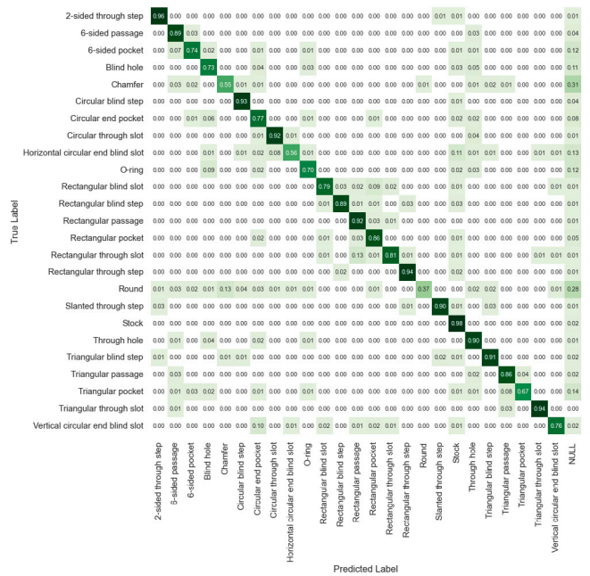
Fig. A.15. Confusion matrix for b-rep face predictions of a trained baseline model configuration.
