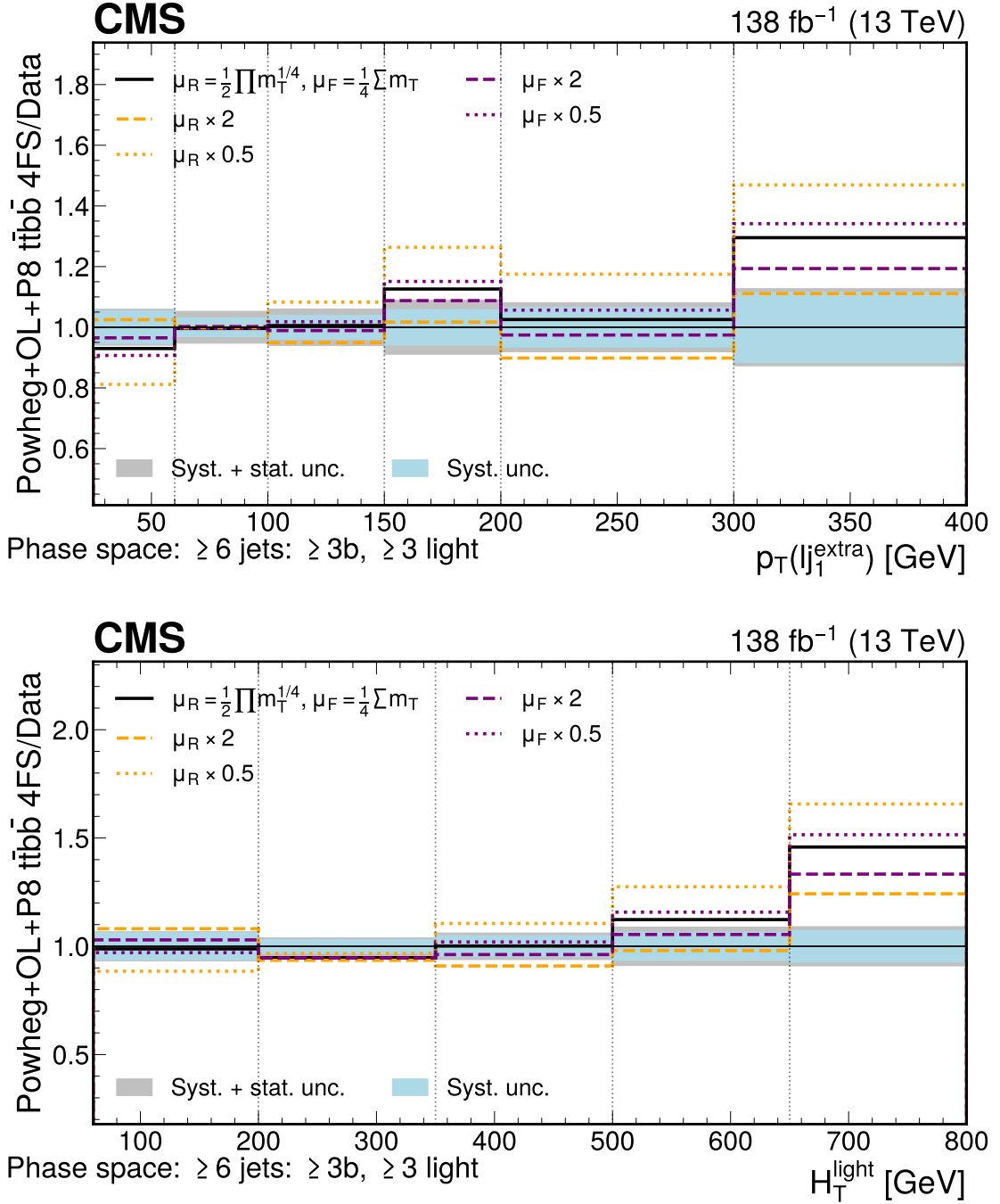
Figure D.2: Ratio of normalized differential cross section predictions of the POWHEG+OL+P8 \bar{t}t\bar{b}\bar{b} 4FS modeling approach with different \mu_R and \mu_F scale settings relative to the measured normalized differential cross sections for the extra light jet (upper) and H_T of light jets (lower) in the \geq 6 \text{ jets: } \geq 3b, \geq 3 \text{ light} phase space. The systematic (total) uncertainties of the measurement are represented as grey (blue) bands. The systematic (total) uncertainties of the measurement are represented as grey (blue) bands. Variations of the \mu_R ( \mu_F ) scale relative to the nominal scale setting are shown in orange (purple). The last bin in the distributions contains the overflow.
