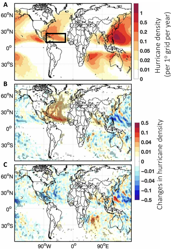
Fig. 3. Maps of hurricane track density. (A) Climatological hurricane track density averaged over 1885–1920 and eight members based on HadISST1. The Atlantic main development region is highlighted by a black box. (B) Ensemble-mean changes in simulated hurricane track density (HadISST1b- minus HadISST1-based simulations). Accounting for groupwise SST offsets significantly increases hurricane density in the North Atlantic over 1885–1920 (dots, P < 0.05 ). (C) as (B) but for changes over 1930–1949. The pattern of changes in hurricane density is similar using either HIRAM or AM2.5 runs (fig. S6). For visualization purposes, hurricane track density on 1^\circ grid-cell is smoothed using a nine-grid two-dimensional (2D) convolutional smoother.
