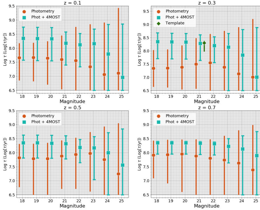
Figure 14. The simulated \log (star formation timescale) results of an elliptical galaxy as a function of magnitude and redshift. The precision of the value is drastically improved at all simulated magnitudes and redshifts when 4MOST is used with photometry. However, at fainter magnitudes the \tau value appears to be restricted by the lower limit. The limits of \log \tau covered in FAST's libraries is shown by the grey shaded region. The limits are set at 6.5 and 11 ( \log[\tau/\text{yr}] ).
