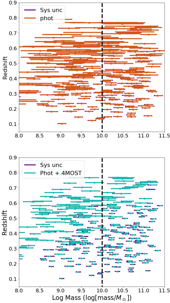
Figure 11. The mass-redshift distribution graph is created with our uncertainties. The SNe were taken from the Supernova Legacy Survey third year data set and the DES 3 year data. Each SN was assigned an uncertainty calculated from phot (in the top panel) and an uncertainty calculated from phot + 4MOST (in the bottom panel). Both plots have a black dashed line representing 10^{10} M_{\odot} . There are 310 SNe plotted. The uncertainty values from the photometry lead to 35 SNe crossing the dashed line. Whilst, the uncertainty values from phot + 4MOST lead to 13 SNe crossing the dashed line.
