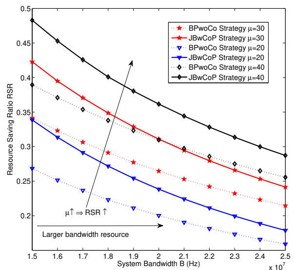
Fig. 7. RSRs achieved by the proposed BPwCo and JBwCoP as the functions of bandwidth resource B for different \mu , given \lambda_m = 5 BS/km 2 , \lambda_s = 10 BS/km 2 , \lambda_u = 400 UE/km 2 , R_m = R_s = 0.35 Mbits/s, \alpha = 4 and \mu = 20 .
