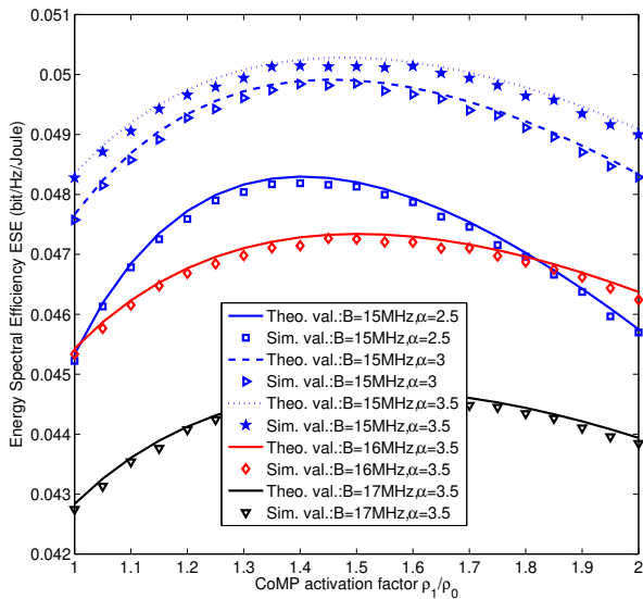
Fig. 4. Theoretical and simulated network's ESEs versus CoMP factor \rho_1/\rho_0 for different B and \alpha , given R_m = R_s = 0.2 Mbits/s, \lambda_m = 5 BS/km 2 , \lambda_s = 200 BS/km 2 , \lambda_u = 500 UE/km 2 and \mu = 20 .
