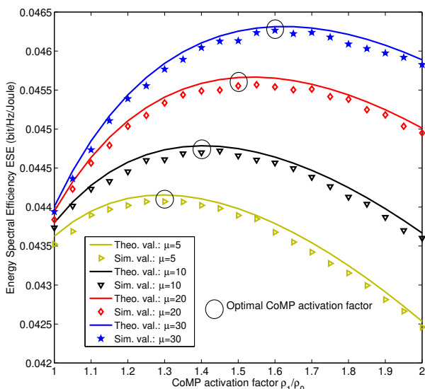
Fig. 2. Theoretical and simulated network's ESEs versus CoMP factor \rho_1/\rho_0 for different \mu , given B = 20 MHz, \lambda_m = 5 BS/km 2 , \lambda_s = 200 BS/km 2 , \lambda_u = 600 UE/km 2 , R_m = R_s = 0.15 Mbits/s and \alpha = 4 .
