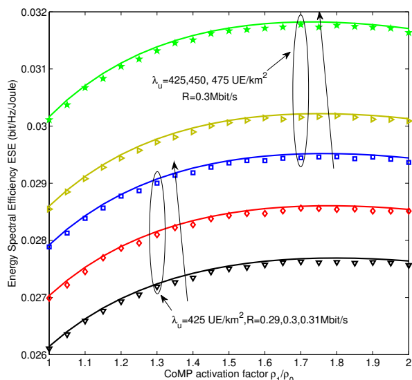
Fig. 3. Theoretical and simulated network's ESEs versus CoMP factor \rho_1/\rho_0 for different \lambda_u and R_m = R_s = R , given B = 20 MHz, \lambda_m = 6 BS/km 2 , \lambda_s = 225 BS/m 2 , \mu = 10 and \alpha = 4 .
