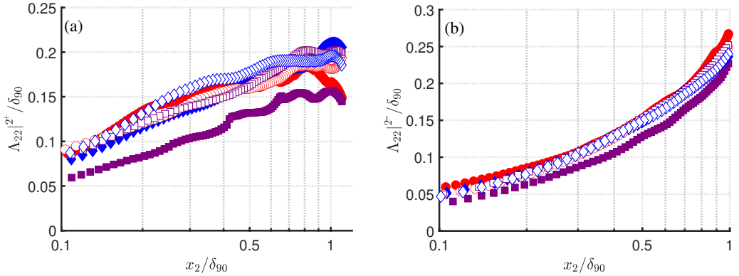
Figure 11: Longitudinal length scales of wall-normal velocity component, estimated from PIV measurements performed at U_\infty \approx 10 m/s. (a) Integral length scale \Lambda_{22}^{+}(x_2) (b) Integral length scale \Lambda_{22}^{-}(x_2) Legends: Red circles 10 PPI, purple squares 45 PPI, and blue diamonds 90 PPI. Open symbols are for 3 mm thick substrate, while filled symbols correspond to 15 mm substrate.
