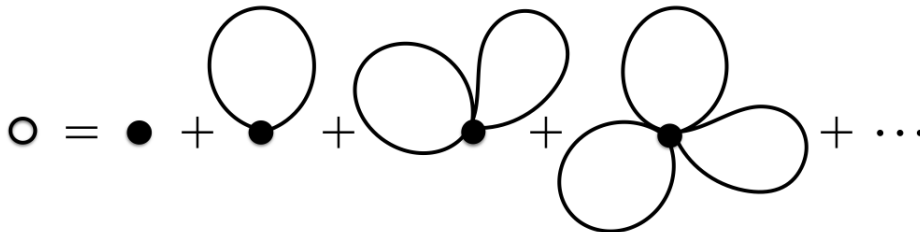
Figure 3.1: The classical interaction vertex is represented by the black dot and has any number of external legs (which are not drawn). Added to this is all its 1PI quantum corrections i.e. the sum over all tadpole corrections.
