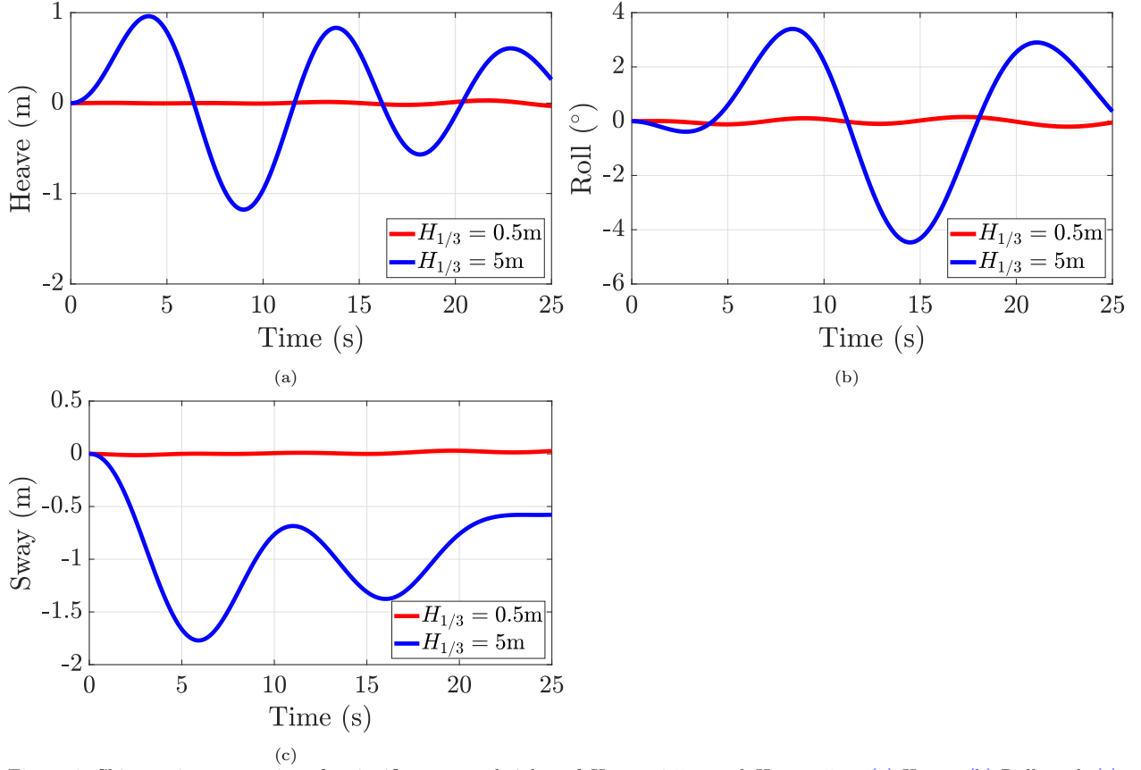
Figure 6: Ship motion comparison for significant wave heights of H_{1/3} = 0.5\text{ m} and H_{1/3} = 5\text{ m} : (a) Heave; (b) Roll; and, (c) Sway.
