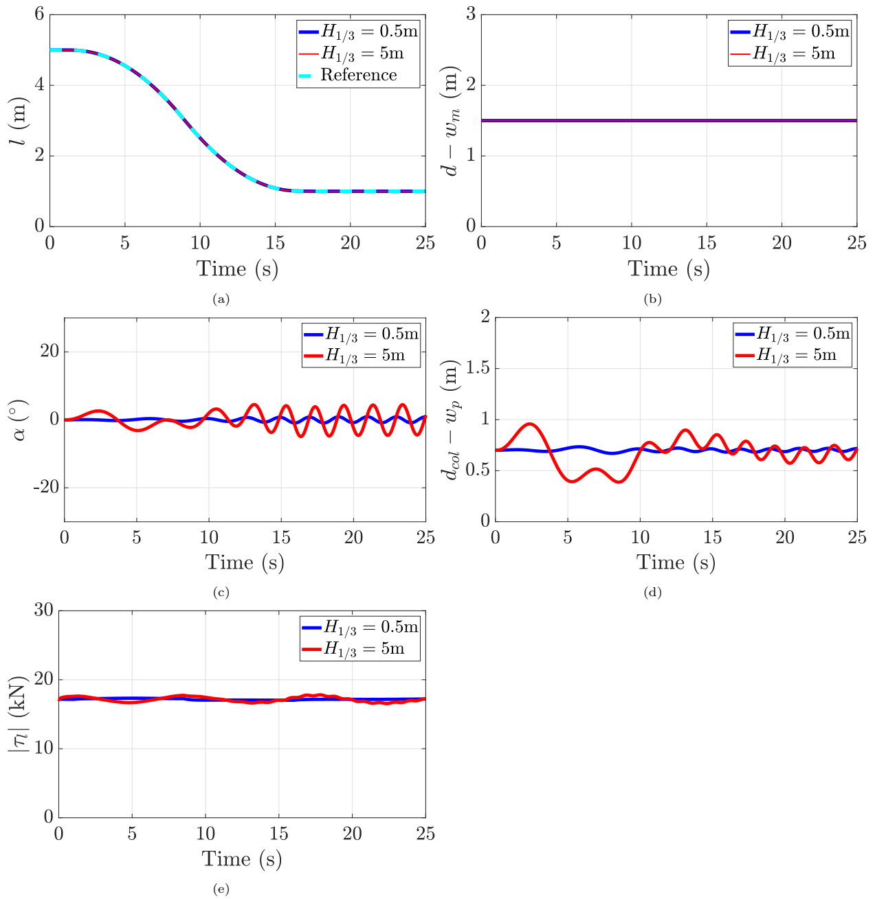
Figure 7: Comparison of crane motions comparison with fixed boom for significant wave heights of H_{1/3} = 0.5\text{m} and H_{1/3} = 5\text{m} , with initial conditions \alpha_0 = 0^\circ , \dot{\alpha}_0 = 0^\circ/\text{s} : (a) Cable length ( l ); (b) Suspension point overhang ( d - w_m ); (c) Swing angle ( \alpha ); (d) Separation distance ( d_{col} - w_p ); and, (e) Tension in crane cable ( |\tau_l| )
