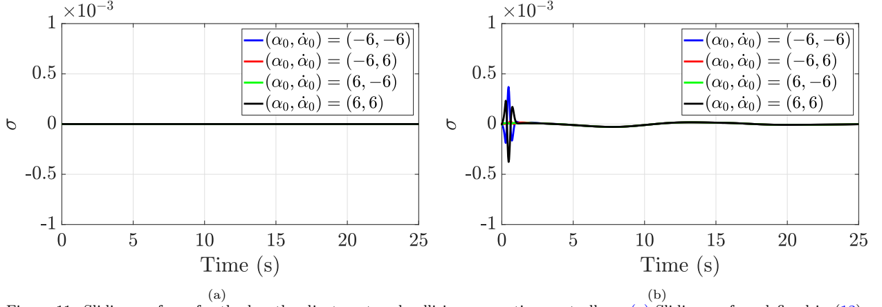
Figure 11: Sliding surfaces for the length adjustment and collision prevention controllers. (a) Sliding surface defined in (12); (b) Sliding surface defined in (42)
