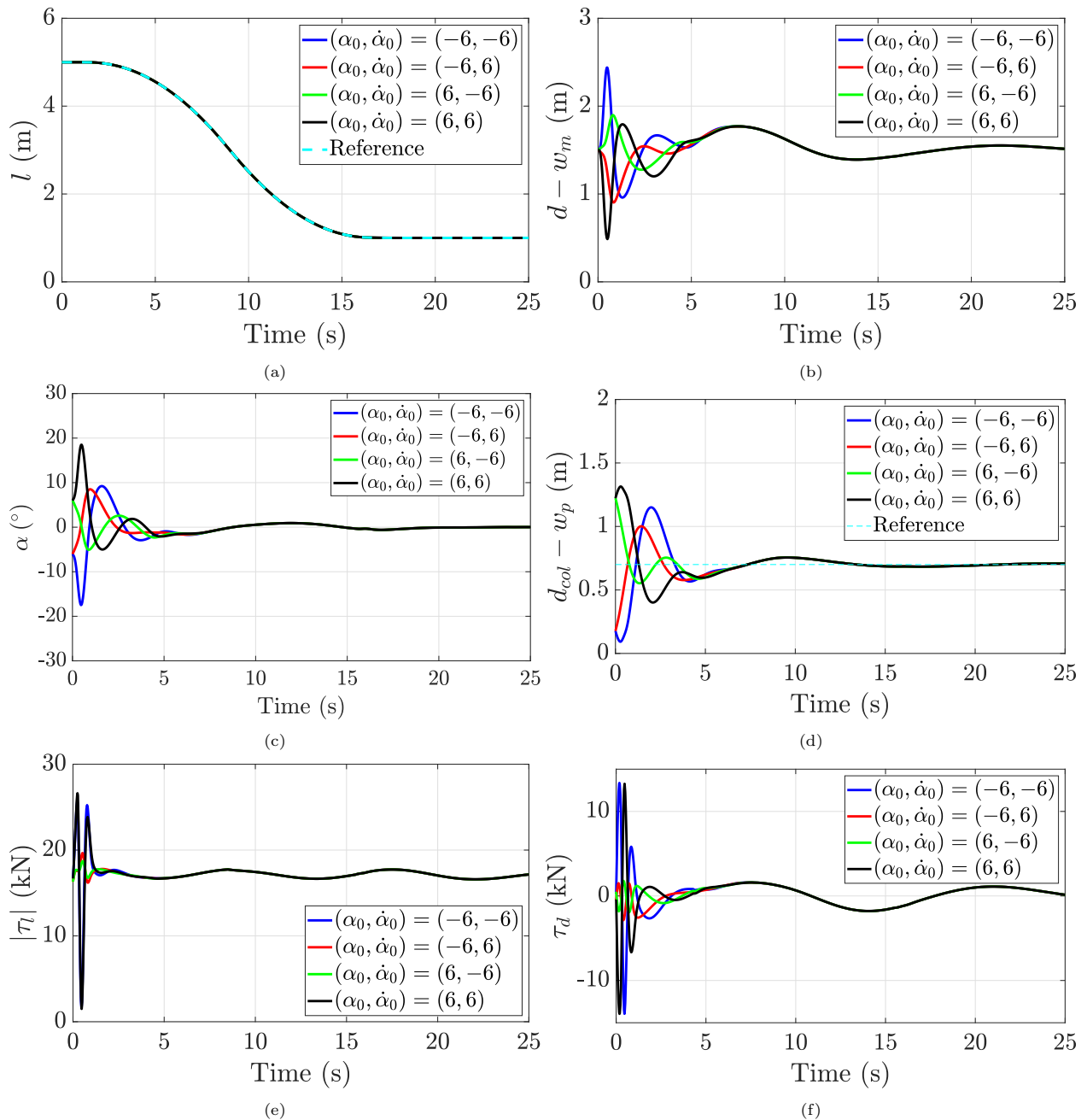
Figure 10: Crane motions with adjustable boom for a significant wave height of H_{1/3} = 5 m and (\alpha_0, \dot{\alpha}_0) = (\pm 6, \pm 6) : (a) Cable length ( l ); (b) Suspension point overhang ( d - w_m ); (c) Swing angle ( \alpha ); (d) Separation distance ( d_{col} - w_p ); (e) Tension in crane cable ( |\tau_l| ); and, (f) Control force on boom ( \tau_d )
