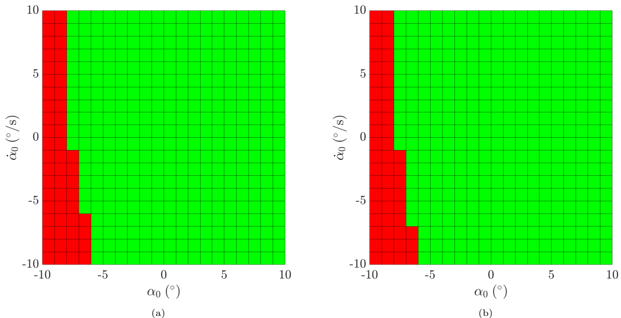
Figure 16: Analysis of the separation distance between the mothership and small boat for a range of initial swing angle and velocities for multiple significant wave heights. The red regions indicate a collision, while the green regions indicate safe operation region. (a) H_{1/3} = 0.5 m, H_{1/3} = 5 m and H_{1/3} = 7.5 m; (b) H_{1/3} = 11.5 m and H_{1/3} = 14 m
