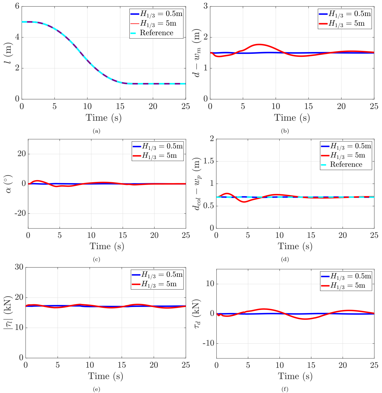
Figure 9: Comparison of crane motions with adjustable boom for a significant wave heights of H_{1/3} = 0.5\text{ m} and H_{1/3} = 5\text{ m} , with initial conditions \alpha_0 = 0^\circ and \dot{\alpha}_0 = 0^\circ/\text{s} : (a) Cable length ( l ); (b) Suspension point overhang ( d - w_m ); (c) Swing angle ( \alpha ); (d) Separation distance ( d_{col} - w_p ); (e) Tension in crane cable ( |\tau_l| ); and, (f) Control force on boom ( \tau_d )
