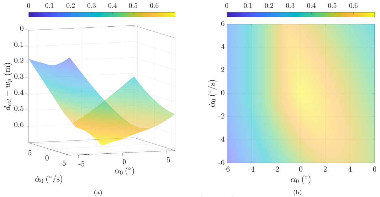
Figure 14: Surface plots for the minimum separation distance ( d_{col} - w_p ) between the small vessel and mothership with an adjustable crane boom for a range of initial swing angle ( \alpha_0 ) and velocities ( \dot{\alpha}_0 ) for a significant wave height of H_{1/3} = 0.5 m: (a) 3D plot; (b) 2D plot
