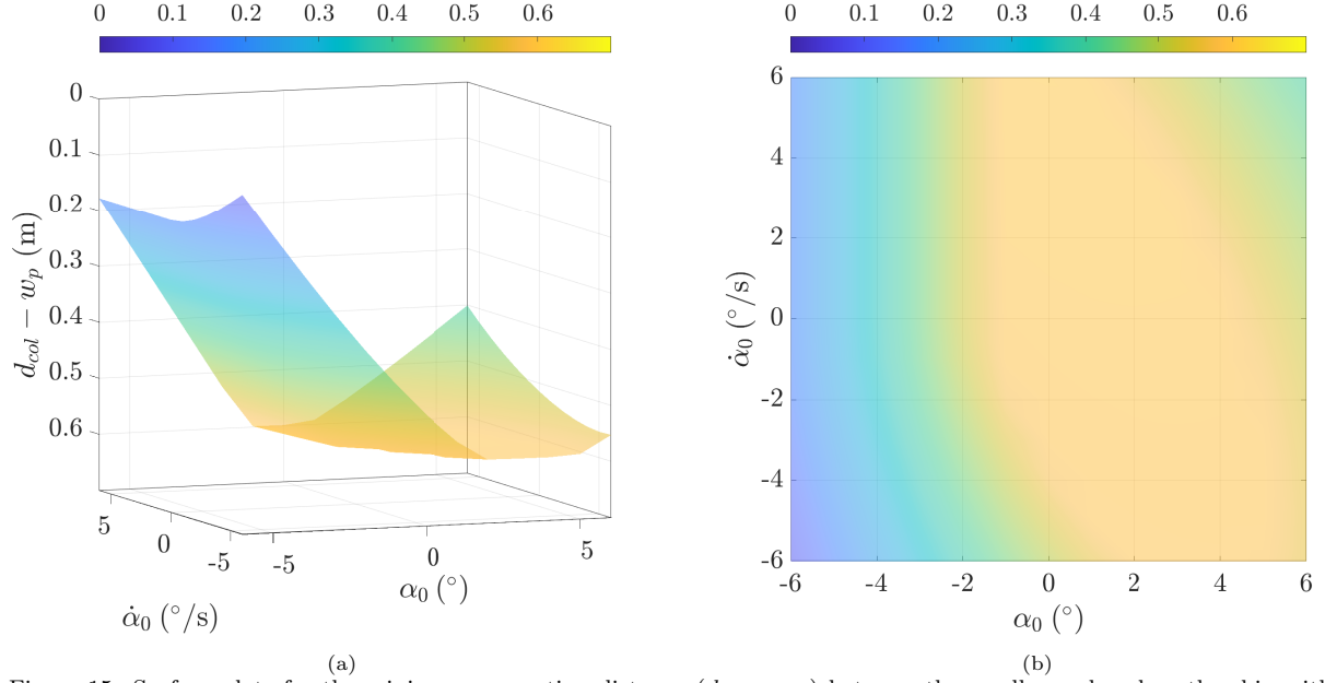
Figure 15: Surface plots for the minimum separation distance ( d_{col} - w_p ) between the small vessel and mothership with an adjustable crane boom for a range of initial swing angle ( \alpha_0 ) and velocities ( \dot{\alpha}_0 ) for a significant wave height of H_{1/3} = 5 m: (a) 3D plot; (b) 2D plot;
