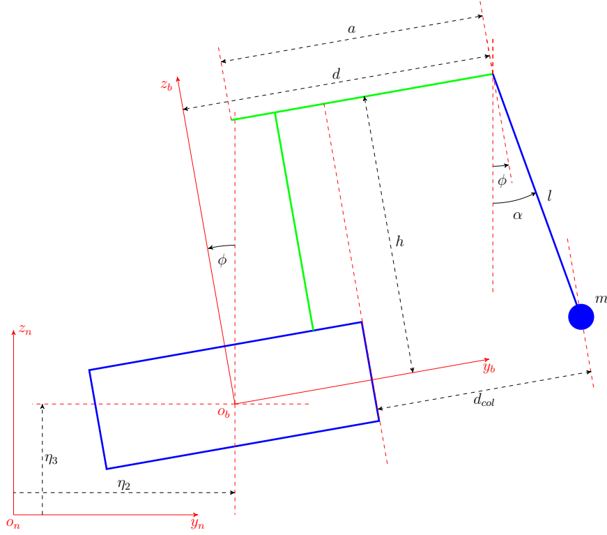
Figure 4: 2D Model of the mothership and small vessel
