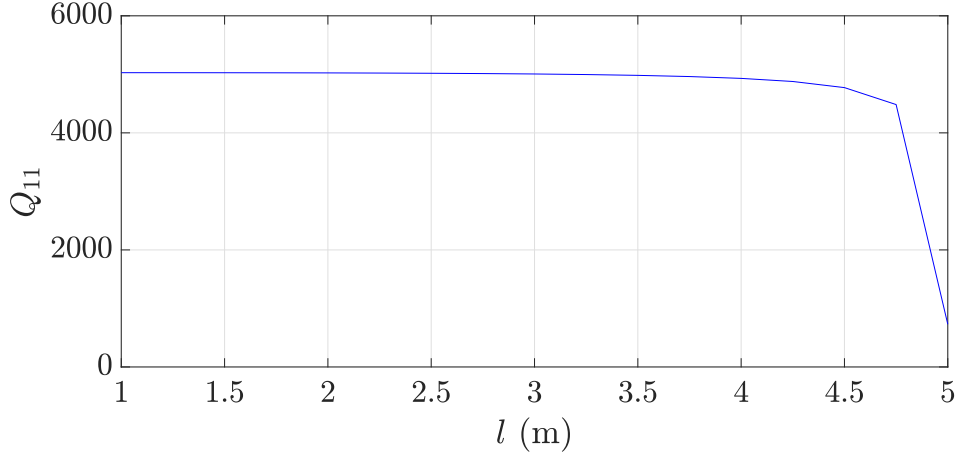
Figure 5: Plot of Q_{11}(l) with respect to l
