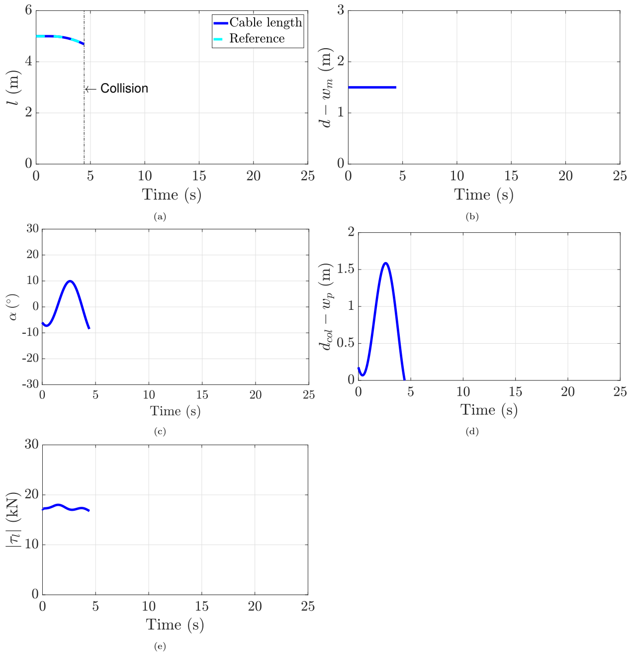
Figure 8: Crane motions with fixed boom for a significant wave height of H_{1/3} = 5 m, \alpha_0 = -6^\circ and \dot{\alpha}_0 = -6^\circ/\text{s} : (a) Cable length ( l ); (b) Suspension point overhang ( d - w_m ); (c) Swing angle ( \alpha ); (d) Separation distance ( d_{col} - w_p ); and, (e) Tension in crane cable ( |\tau_l| )
