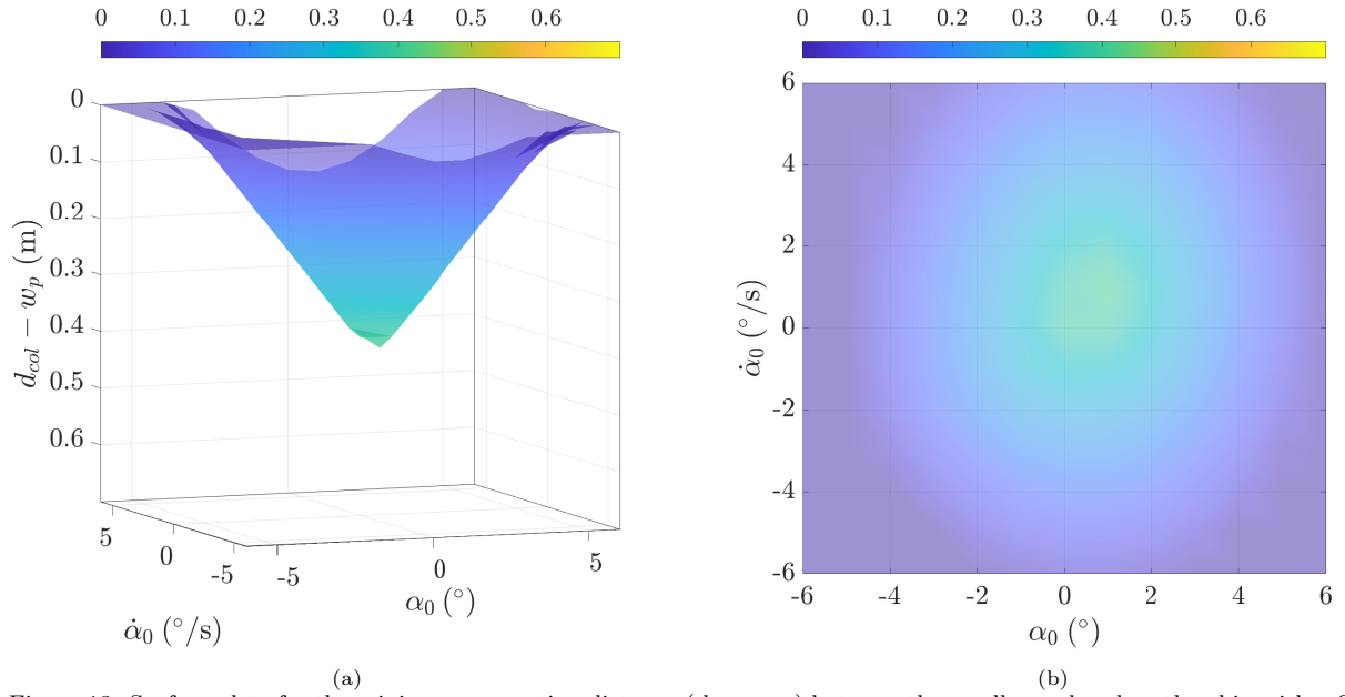
Figure 13: Surface plots for the minimum separation distance ( d_{col} - w_p ) between the small vessel and mothership with a fixed crane boom for a range of initial swing angle ( \alpha_0 ) and velocities ( \dot{\alpha}_0 ) for a significant wave height of H_{1/3} = 5 m: (a) 3D plot; (b) 2D plot
