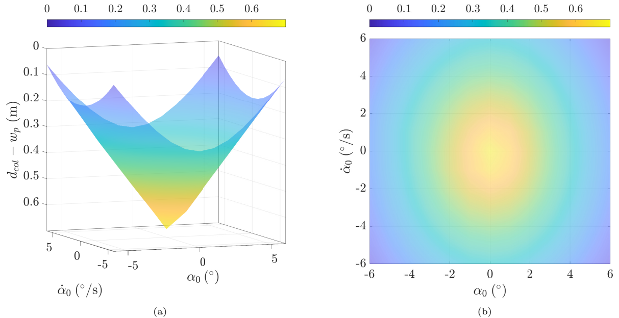
Figure 12: Surface plots for the minimum separation distance ( d_{col} - w_p ) between the small vessel and mothership with a fixed crane boom for a range of initial swing angle ( \alpha_0 ) and velocities ( \dot{\alpha}_0 ) for a significant wave height of H_{1/3} = 0.5 m: (a) 3D plot; (b) 2D plot
