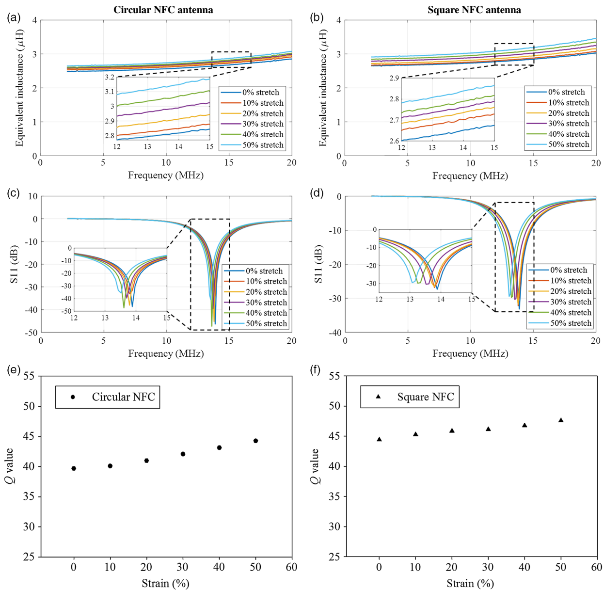
Figure 3. Experimental results of the coil's EM properties under uniaxial deformation with 10%, 20%, 30%, 40% up to 50% elongation. a,b) Circular and square coils inductance. c,d) Circular and square coils S11 parameters with respect to resonant frequencies. e,f) Circular and square coils Q values.
