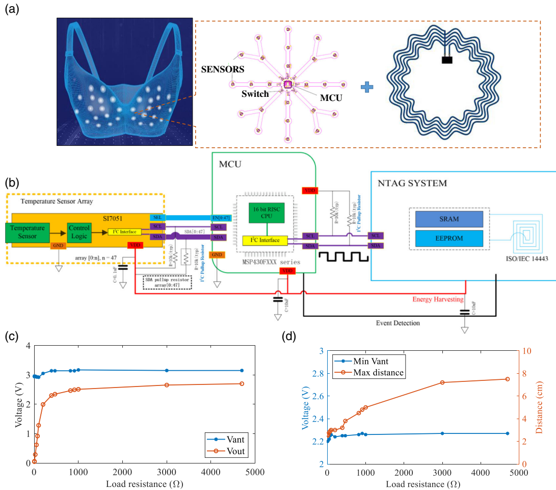
Figure 6. NFC-based battery-free body sensing system. a) Exploded-view and schematic illustration of the temperature monitoring bra. b) Circuitry schematic of the NFC-powered temperature-sensing system. c) Harvested voltage at the NFC antenna terminals. d) The maximum reading distance (right) and the rectified DC voltage (left) under different loads. e) Android-based APP for NFC communication and sensing temperature acquisition. f) The fluctuation of the sensing temperature at different controlled temperatures of 33, 35, 37, 39 and 41 °C, respectively. g) The Newton thermal manikin system used for temperature-sensing experiments. h,i) The acquired temperatures of right-side and left-side bra on the manikin, with temperature set from 35 to 39 °C.
