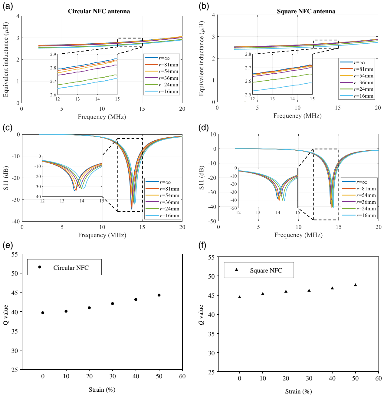
Figure 4. Experimental results of the coil's EM properties under bending curvature of 81, 54, 36, 24, and 16 mm. a,b) Circular and square coils inductance. c,d) Circular and square coils S11 parameters with respect to resonant frequencies. e,f) Circular and square coils Q values.
