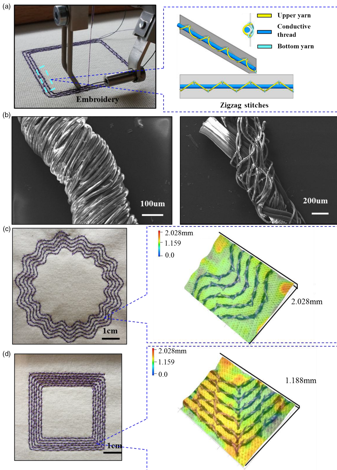
Figure 1. Proposed embroidery processes of the NFC coils a) Conductive threads fastened by the zigzag stitches. b) SEM images of the conducting copper yarns twisted and covered with nylon yarns. c.,d) Images of embroidered conductive yarn-based circular ( d = 62 \text{ mm} ) and square ( d = 42.8 \text{ mm} ) coil antennas.
