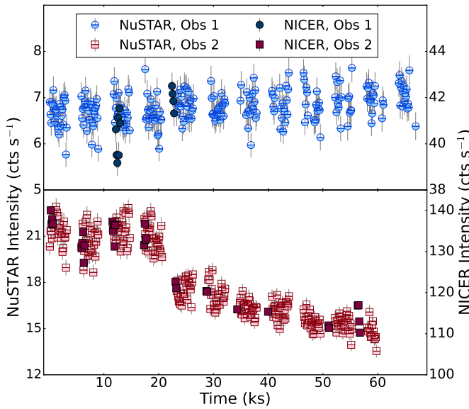
Figure 2. Light curve for the NuSTAR (half-filled) and NICER (filled) observations of SLX 1735–269 binned to 128 s. The top panel represents Obs 1 (blue circles) and the bottom represents Obs 2 (red squares). Only one NuSTAR focal plane module (FPM) is shown for clarity.
