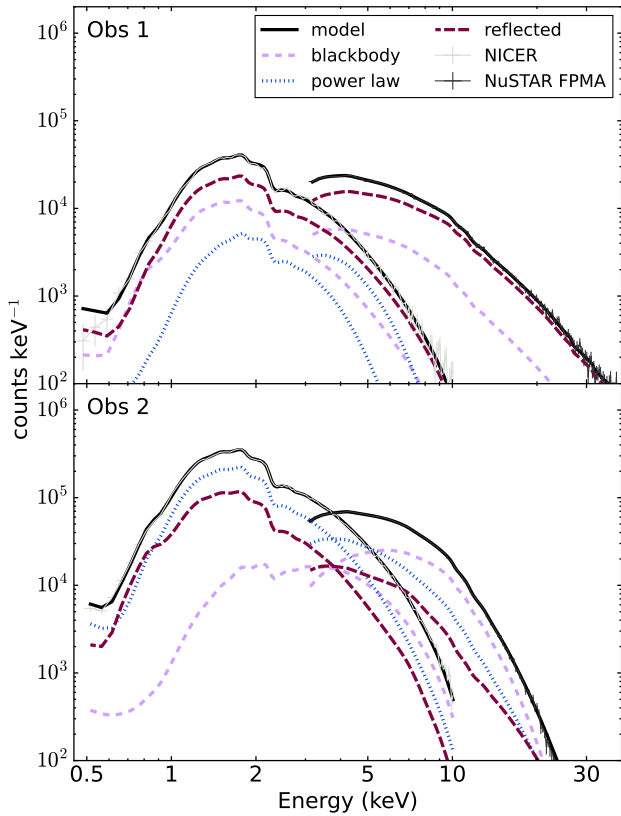
Figure 4. The NICER and NuSTAR spectra in units \text{counts keV}^{-1} and the respective model components from XILLVERCO for both observations. We can see here that Obs 1 has an overall lower flux and different shape to that of Obs 2, which displays a cutoff in the power law around 5.8 keV.
