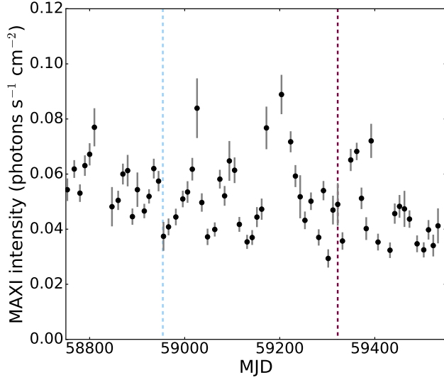
Figure 1. A long term MAXI light curve for the source. Vertical lines indicate the dates at which Obs 1 (left, blue) and Obs 2 (right, red) occur. We see that Obs 1 occurs during a lower flux state than Obs 2. The MAXI data are binned to 10 days.
