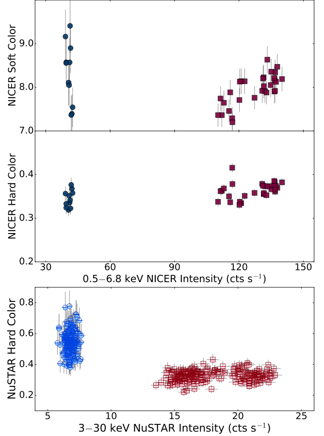
Figure 3. Color-Intensity diagrams for NICER and NuSTAR observations of SLX 1735–269. Markers match those used in Figure 2. The top and middle panels represent the soft and hard color in NICER (respectively defined using the bands 1.1–2.0 keV/0.5–1.1 keV and 3.8–6.8 keV/2.0–3.8 keV), and the bottom panel represents the hardest color measurement in NuSTAR, defined using the bands 10–16 keV/6.4–10 keV.
