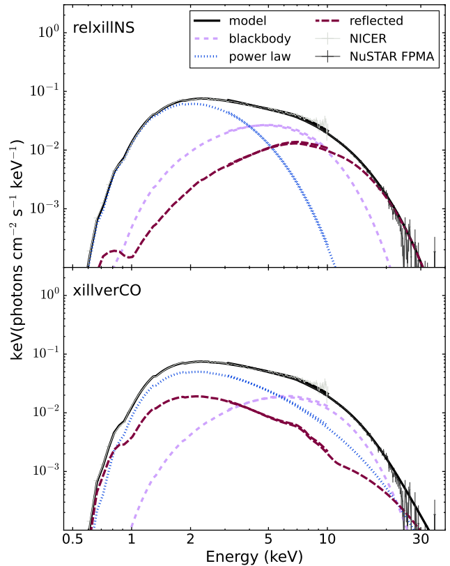
Figure 7. This plot compares the unfolded spectrum for Obs 2 when modeled with RELXILLNS with logN fixed at 17 to the spectrum modeled with XILLVERCO (the same spectrum shown in Figure 4). We see that the reflection component shifts strongly toward higher energies, and so the powerlaw and blackbody must shift toward lower energies to account for this.
