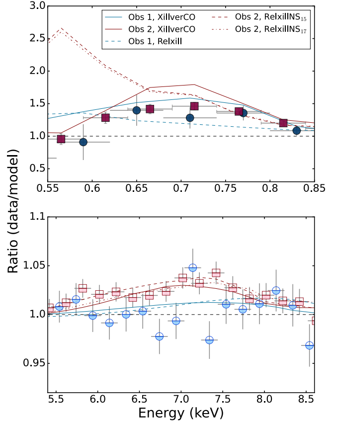
Figure 5. Shown here are the regions containing the (top) O VIII \text{Ly}\alpha in NICER and (bottom) Fe \text{K}\alpha reflection in NuSTAR FPMA. These are constructed by ignoring the regions surrounding the line in XSPEC, fitting a continuum, then reintroducing these regions and plotting the ratio of the data to the model. The subscripts 15 and 17 refer to the value at which \log N is fixed for RELXILLNS in each model. We see strong evidence for a feature around the O VIII energy band, but a feature around the Fe \text{K}\alpha energy band is significantly weaker, at only about 3-4% above continuum. We show the different models used and find that only XILLVERCO effectively detects the feature in the lower energy bands.
