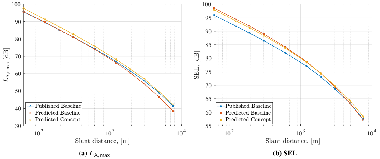
Fig. 9 Estimated departure NPD curves for Concept B8, compared against the published ones of the reference aircraft DHC-6 Twin Otter.
