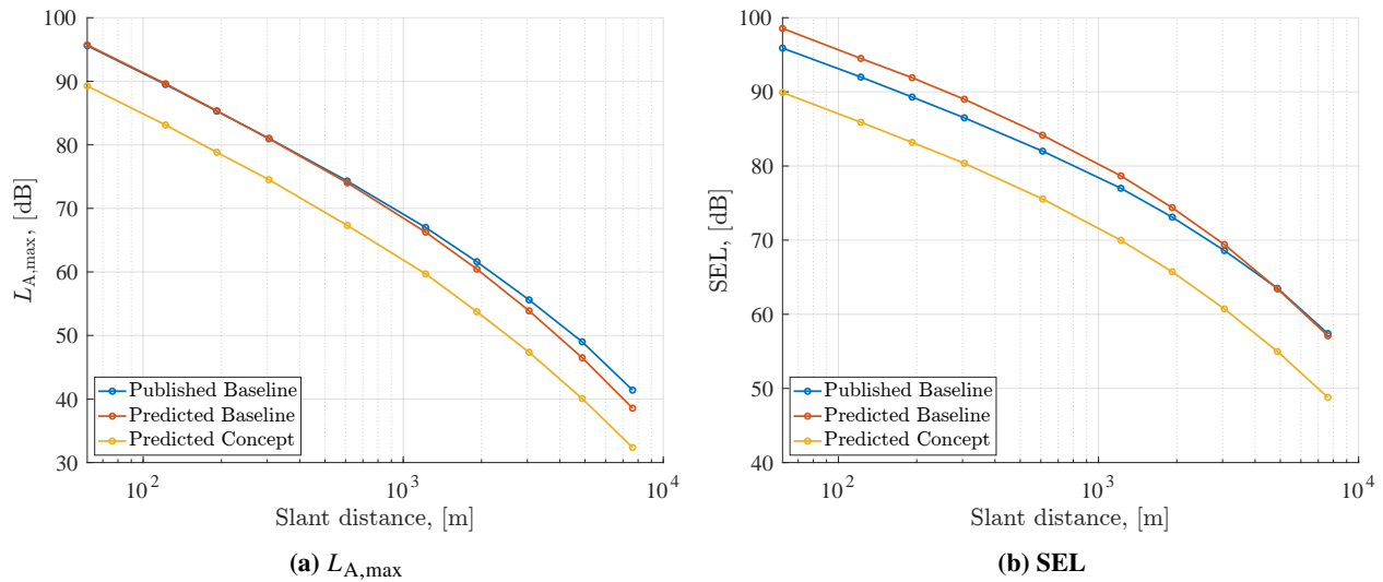
Fig. 8 Estimated departure NPD curves for Concept B5, compared against the published ones of the reference aircraft DHC-6 Twin Otter.
