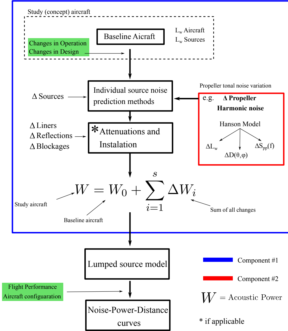
Fig. 1 Flow diagram of the lumped noise source modelling framework.
