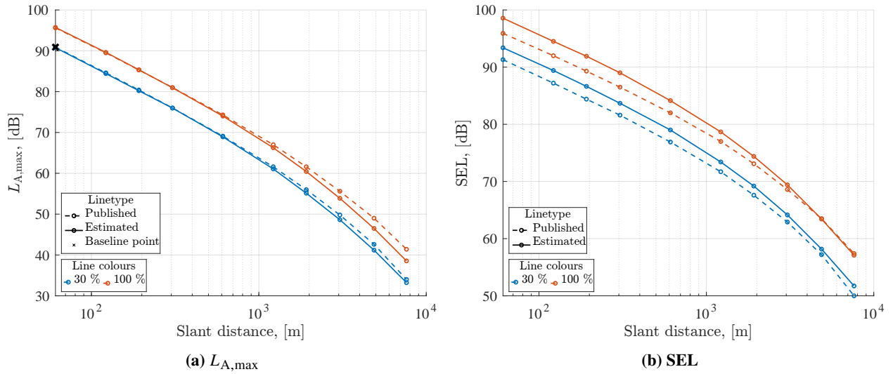
Fig. 5 Takeoff NPD curves for a twin engine de Havilland Canada DHC-6 (Twin Otter). Solid lines indicate the predicted levels, whereas dashed are the baseline aircraft published NPD data.
