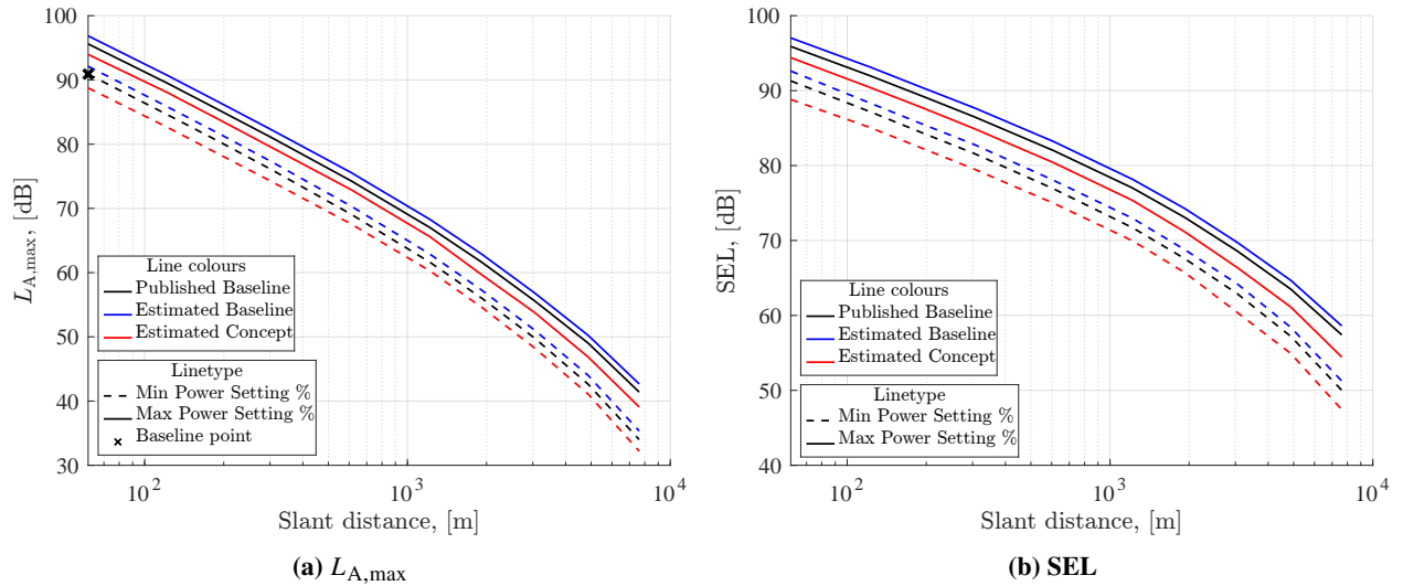
Fig. 11 Estimated approach NPD curves for Concept B5, compared against the published ones of the reference aircraft DHC-6 Twin Otter.
