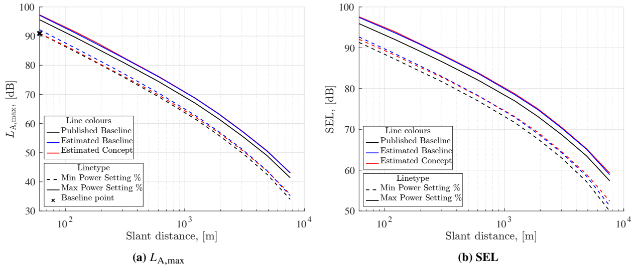
Fig. 12 Estimated approach NPD curves for Concept B8, compared against the published ones of the reference aircraft DHC-6 Twin Otter.
