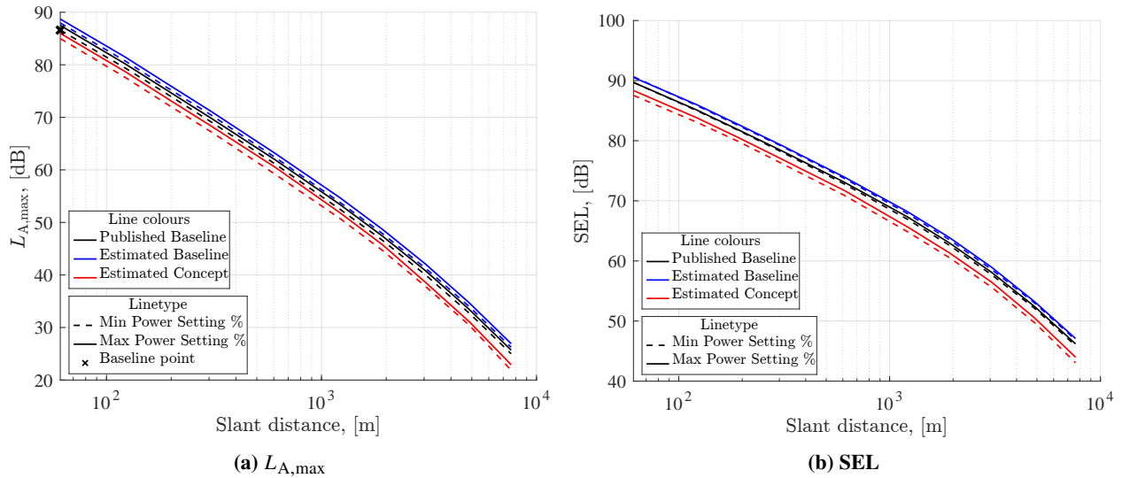
Fig. 13 Predicted approach NPD curves for Concept E1, compared against the published ones of the reference aircraft ATR72-212A.
