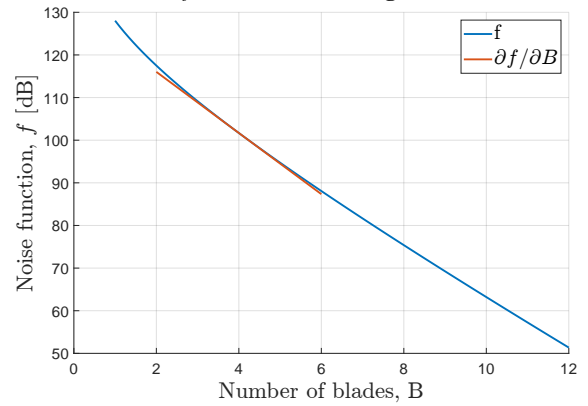
(d) Variation of f as a function of propeller number of blades.
