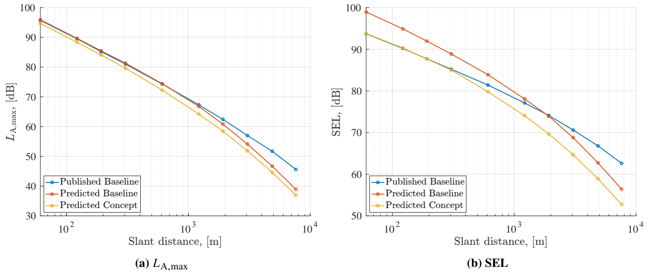
Fig. 10 Estimated departure NPD curves for Concept E1, compared against the published ones of the reference aircraft ATR72-212A.
