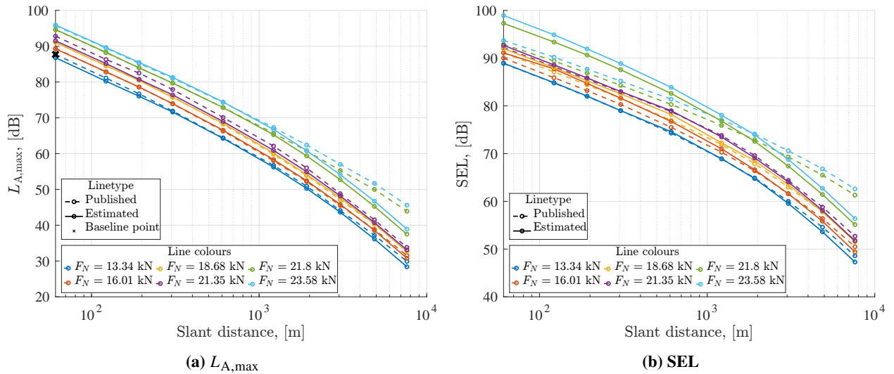
Fig. 6 Takeoff NPD curves for a twin-engine turboprop ATR 72-212A. Solid lines indicate the predicted levels, whereas dashed are the baseline aircraft published NPD data.
