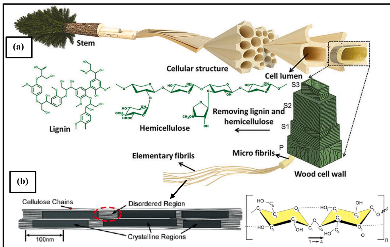
Fig. 3. (a) Schematic representation showing the hierarchical structure of a wood (adapted with permission from [76], copyright 2020, Wiley VCH GmbH); (b) CNCs and amorphous regions (disordered) of fibrils composed of cellulose chain unit (adapted from [77] copyright 2011, the Royal Society of Chemistry).
