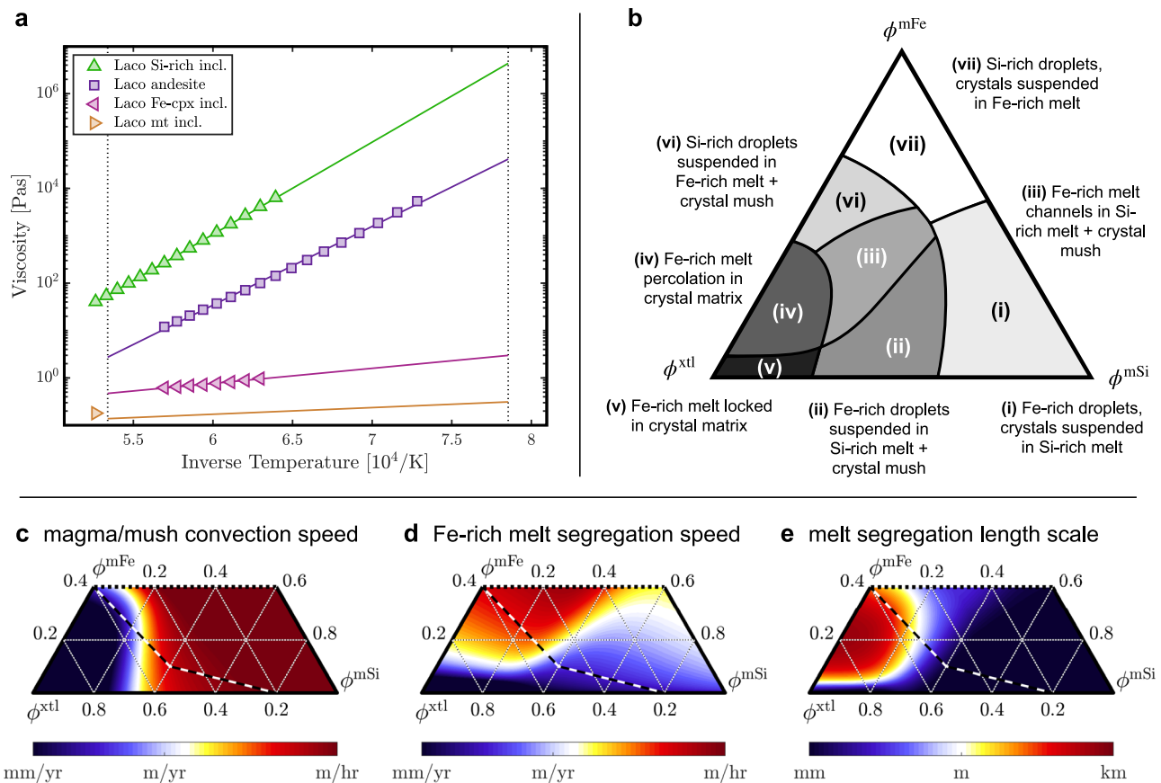
Fig. 4 | Viscometry and scaling analysis pertaining to ore melt separation from parent magma body. a Viscometry results (symbols) with fitted model (lines) for rhyolite (green), andesite (purple), Fe-clinopyroxene (pink), and magnetite (amber) compositions (see Table 1 and Supplementary Table 1); b regime diagram of three-phase flow between Si-rich melt ( \phi^{mSi} ), Fe-rich melt ( \phi^{mFe} ), and phenocryst ( \phi^{xtl} )
