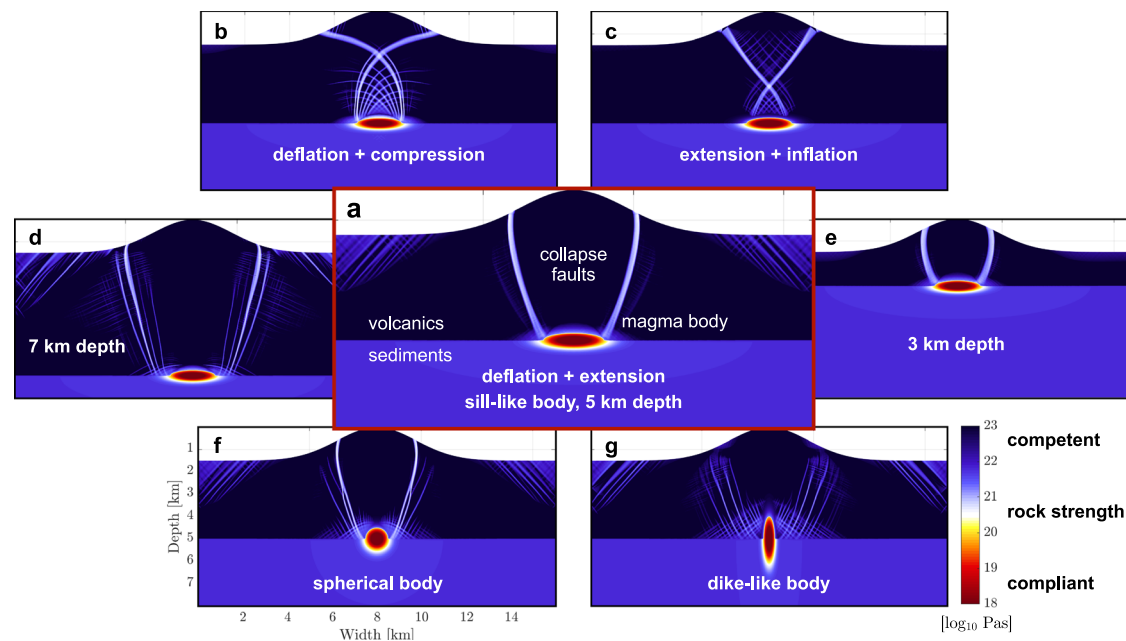
Fig. 5 | Results of volcano deformation models show emerging collapse fracture geometries. a Best-fit case of deflating magma body under tectonic extension, steep failure zones extend laterally from base of magma body to edifice flanks; b for deflation combined with compression, and c for extension combined with inflation, steep cross-cutting fracture zones emerge from roof of magma body. Favourable
