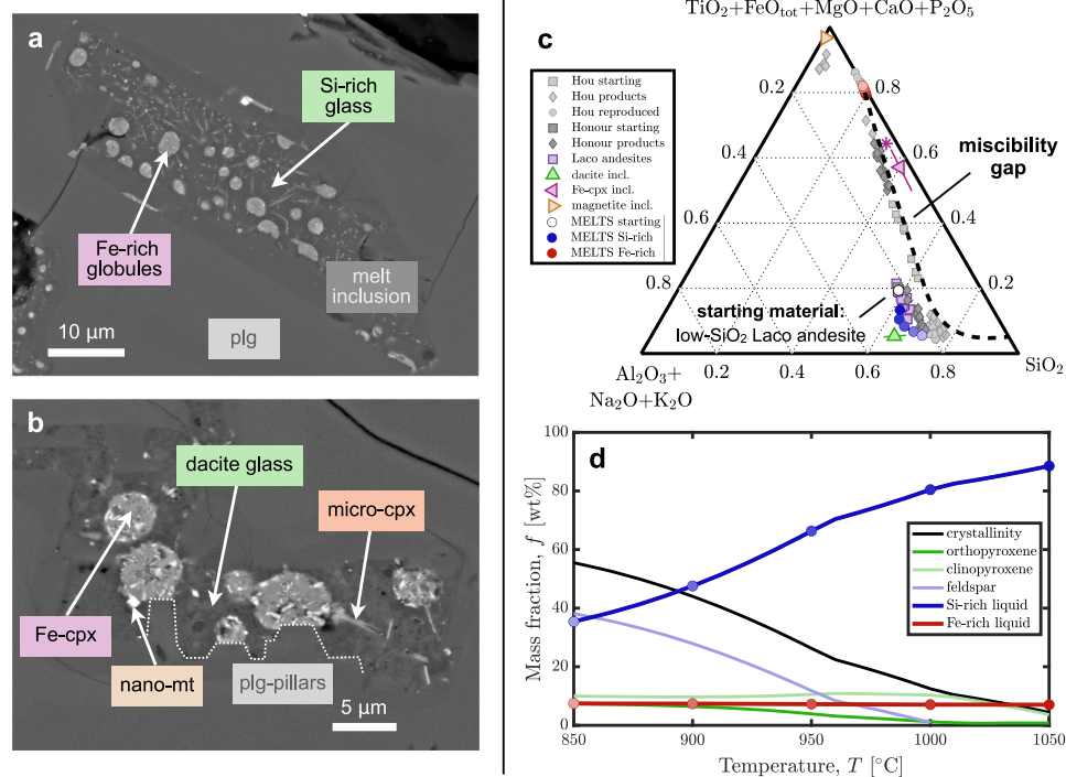
Fig. 3 | Liquid immiscibility in El Laco andesite. Back-scattered electron images of plagioclase-hosted (plg) melt inclusions from ore-hosting andesites; a Fe-rich globules in Si-rich matrix; b higher magnification image shows high-SiO 2 dacite glass matrix with some clinopyroxene micro-phenocrysts (micro-cpx), and Fe-rich globules comprised of Fe-clinopyroxene (Fe-cpx) with some nanocrystalline magnetite (nano-mt); plagioclase shows pillar structures indicative of melt unmixing during crystallisation 9 . Modelling of closed-system isobaric cooling in alphaMELTS shown at 50 °C intervals from 1050 °C (darker) to 850 °C (lighter) in (c) predict Si-rich melt
