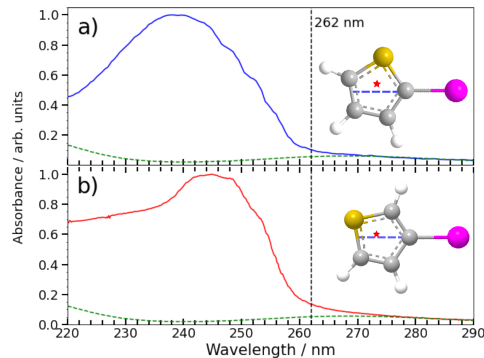
FIG. 7: Gas phase absorption spectrum of 2IT a) and 3IT b) are plotted as solid lines along with a scaled absorption spectrum of \text{CH}_2\text{BrI} (dashed line) to emphasise the weak long wavelength absorption attributable to n\sigma^* excitation in both 2- and 3-iodothiophene. The intensity scale has been normalized to the maximum measured for each isomer to show relative changes in the shape. The structure of the two isomers are plotted as insets with the C-I bond vector highlighted as a dashed blue line and the center of mass of the thiophenyl radical marked by a star.
