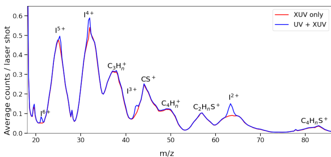
FIG. 2: Mass spectra obtained from ionization of 2IT by UV + XUV pulses (blue) and by XUV pulses only (red). Each spectrum has been normalized by the total number of shots. The UV + XUV signal has been summed over all positive pump-probe delays (i.e. with the UV pulse preceding the XUV pulse).
