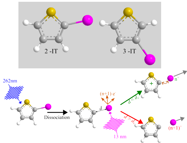
FIG. 1: Top: A ball and stick representation of 2-iodothiophene (2IT) and 3-iodothiophene (3IT). In both structures carbon atoms are grey, hydrogen is white, iodine is purple and sulphur is yellow. Bottom: A schematic representation of the measurement process. 262 nm light absorption leads to fission of the C-I bond. Subsequent site-selective ionization with a 13 nm pulse leads to an (n+1)^+ charge on the iodine atom. If the separation between the co-fragments, d , is less than the critical distance, d_c , charge can transfer to the neutral thiophenyl co-fragment leading to Coulomb explosion. Once the distance is greater than d_c , CT can no longer occur, and the kinetic energy of the iodine ion measured is determined by the neutral dissociation process.
