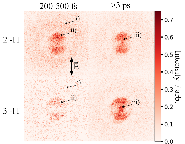
FIG. 3: I^{2+} ion images following UV pump and subsequent XUV ionization of 2IT (top row) and 3IT (bottom row) summed over 200-500 fs (left column) and at all delays >3 ps (right column), representative of early and late dynamics. Each image was normalized to its peak intensity and the laser polarization axis E is marked in the top left panel.
