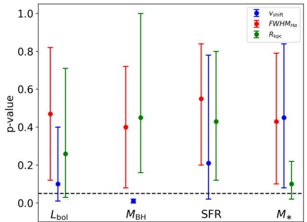
Figure 4. The plot shows the null-hypothesis probability for non-correlation between different extended H \alpha properties and the properties of the black hole and the host galaxy. The dashed black line shows the 5 percent line for p-value, used as a demarcation between the presence or absence of correlations.
