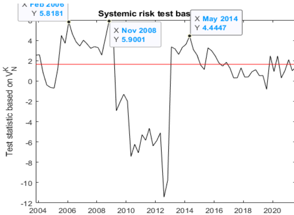
Figure 6: Evolution of systemic risk statistics for coverage probability \bar{\tau} = 0.05 and KS based test statistics introduced in (36). The cross section of stocks is comprised by N = 68 assets of the FTSE-100 index computed over 72 rolling windows of T = 1000 in-sample observations. The red flat line denotes the Gaussian critical value of the systemic risk tests at an \alpha = 0.05 significance level. The evaluation period is October 2003 to July 2022.
