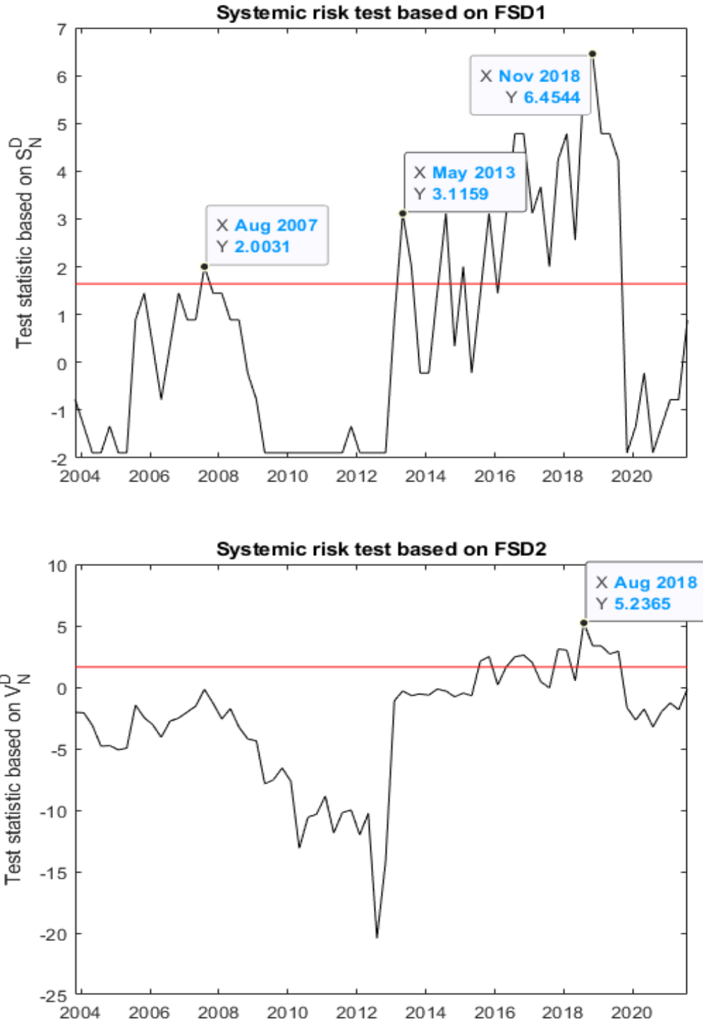
Figure 3: Evolution of systemic risk statistics for coverage probability \bar{\tau} = 0.10 and FSD based test statistics \bar{S}_N^D(q) and \bar{V}_N^D(q) . The cross section of stocks is comprised by N = 68 assets of the FTSE-100 index computed over 72 rolling windows of T = 1000 in-sample observations. The red flat line denotes the Gaussian critical value of the systemic risk tests at an \alpha = 0.05 significance level. The evaluation period is October 2003 to July 2022.
