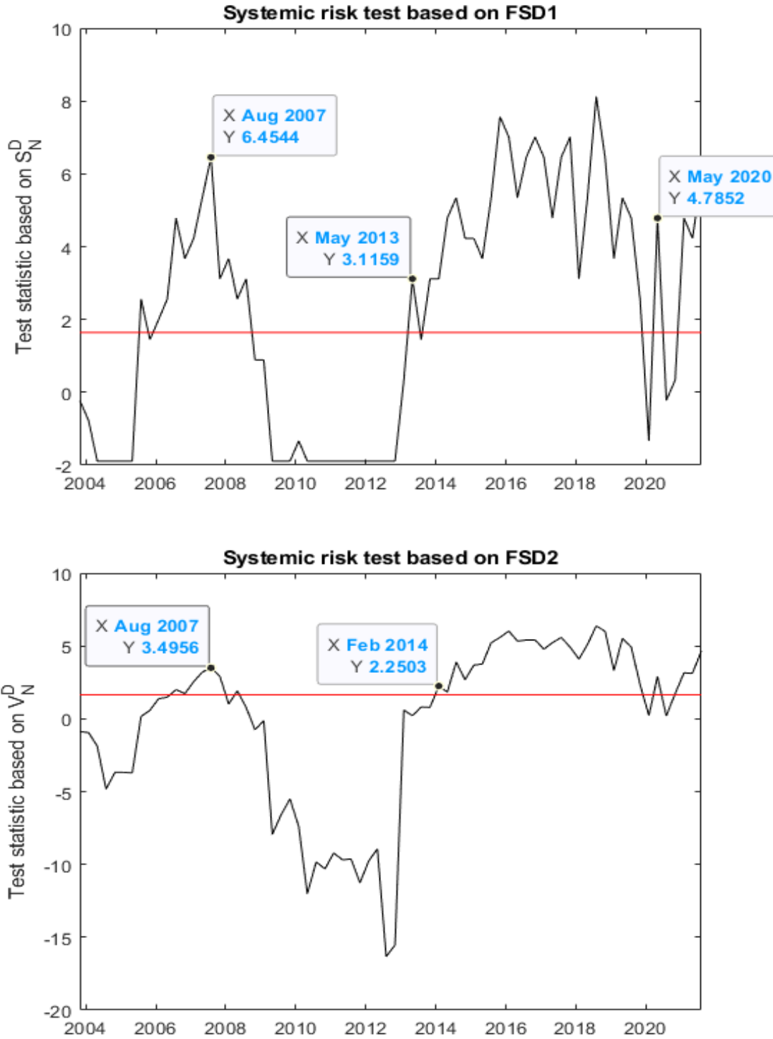
Figure 5: Evolution of systemic risk statistics for coverage probability \bar{\tau} = 0.05 and FSD based test statistics \bar{S}_N^D(q) and \bar{V}_N^D(q) . The cross section of stocks is comprised by N = 68 assets of the FTSE-100 index computed over 72 rolling windows of T = 1000 in-sample observations. The red flat line denotes the Gaussian critical value of the systemic risk tests at an \alpha = 0.05 significance level. The evaluation period is October 2003 to July 2022.
