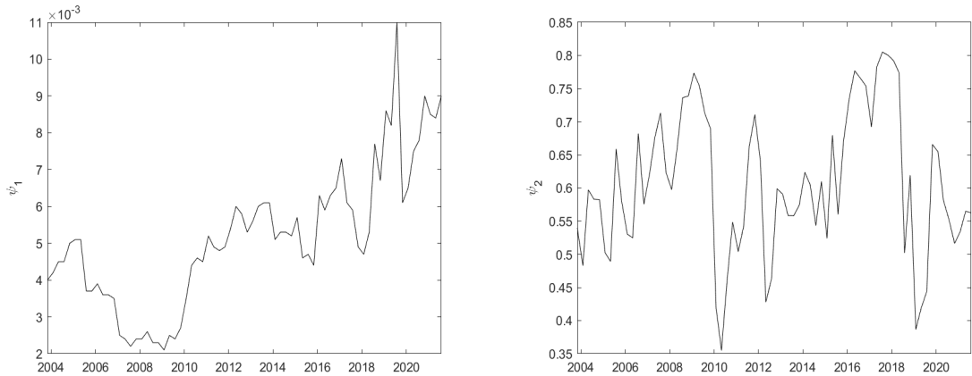
Figure 2: Dynamics of DCC parameters \psi_1 and \psi_2 for DCC-GARCH model (3)-(5) estimated by quasi-maximum likelihood for the vector of 68 stocks remaining in the FTSE-100 index over the period 4/1/2000 to 22/7/2022 ( 5754 \times 68 observations). The estimates are obtained from rolling windows of 66 observations with an in-sample estimation period of T = 1000 observations.
