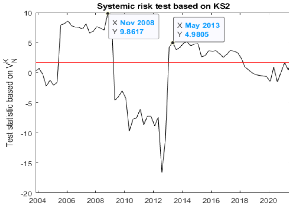
Figure 4: Evolution of systemic risk statistics for coverage probability \bar{\tau} = 0.10 and KS based test statistics introduced in (36). The cross section of stocks is comprised by N = 68 assets of the FTSE-100 index computed over 72 rolling windows of T = 1000 in-sample observations. The red flat line denotes the Gaussian critical value of the systemic risk tests at an \alpha = 0.05 significance level. The evaluation period is October 2003 to July 2022.
