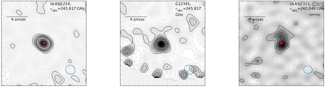
Figure 2. 16 \times 16'' continuum images at \nu_{\text{obs}} \sim 245 GHz produced from the ALMA Band 6 data for ULASJ1234 (left), G1234S (middle) and ULASJ2315 (right). The solid and dashed lines represent positive and negative flux contours at intervals of 1.5\sigma . The location of the quasars is marked with a star and the beam size and position angle is indicated in the bottom right-corner of each image. North is up and East is to the right.
