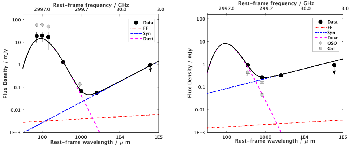
Figure 6. Best-fit SEDs to the far infra-red and radio continuum for ULASJ1234 (left) and ULASJ2315 (right). Black points represent the observed photometry used for the fitting. Error-bars for the ALMA and JVLA continuum data points are generally smaller than the symbol size on the plot. The SED is modelled as the sum of three components - a T_d = 47\text{K} , \beta = 1.6 greybody to model the dust emission (dashed line), a power-law with spectral index, \alpha to model synchrotron emission (dot-dashed line) and a free-free emission component with a power-law index of \alpha_{\text{ff}} = -0.1 (dotted line). The free parameters in the fit are the SFR, the synchrotron spectral index, \alpha and the scaling factor for the non-thermal synchrotron emission. We also show the upper limits on the 1.4GHz flux densities from FIRST for both quasars. In the case of ULASJ1234 we also include Herschel -SPIRE photometry at 250, 350 and 500 \mu\text{m} to constrain the peak of the SED. The total Herschel emission shown by the grey points, is a blend of the quasar and the two other companion galaxies and for the fitting we assume that the fluxes are divided equally between the three systems (black points). We also show the total ALMA Band 3 continuum flux from all 3 galaxies in grey. In the case of ULASJ2315, the fits have been conducted by considering the integrated fluxes of both components of the major merger, as we do not have the angular resolution at all the observed frequencies to be able to disentangle emission from the two components of the merger. At the highest frequencies, where we do have enough angular resolution to be able to measure the flux densities for each component of the merger, we also show the individual flux densities for the QSO and the GAL component, although these have not been used in the fitting.
