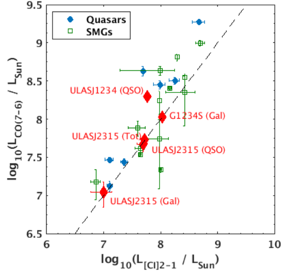
Figure 8. The CO(7-6) versus CI(2-1) intrinsic (magnification corrected) luminosity for quasars and SMGs from Carilli & Walter (2013) and Gullberg et al. (2016) compared to our reddened quasars and their companion galaxies. In the case of ULASJ2315, which is a close separation merger, we present both integrated line luminosities for the entire system as well as the individual line luminosities for each spatial component from Section 3.3. The dashed line shows the 1:1 relation between the two luminosities.
