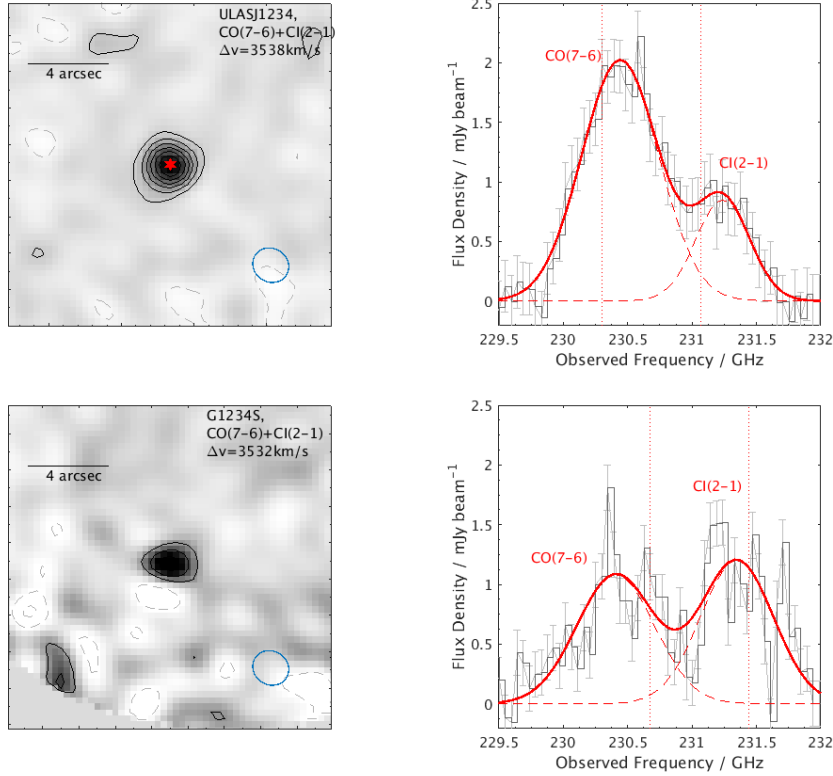
Figure 4. Left: 16 \times 16'' CO(7-6)+CI(2-1) line maps integrated over the two subbands containing both lines for ULASJ1234 (top) and its companion galaxy G1234S (bottom). The solid and dashed lines represent positive and negative flux contours at intervals of 1.5\sigma . The location of the quasar is marked with a star and the beam size and position angle is indicated in the bottom right-corner of each image. North is up and East is to the right. Right: CO(7-6) and CI(2-1) spectral line profiles together with the best-fit model to these line profiles represented by the sum (solid) of two (dashed) Gaussian profiles. Error-bars denote the 1\sigma RMS per channel. Vertical dotted lines mark the expected position of these lines based on the CO(3-2) derived redshifts for the sources in B17 and Paper II.
