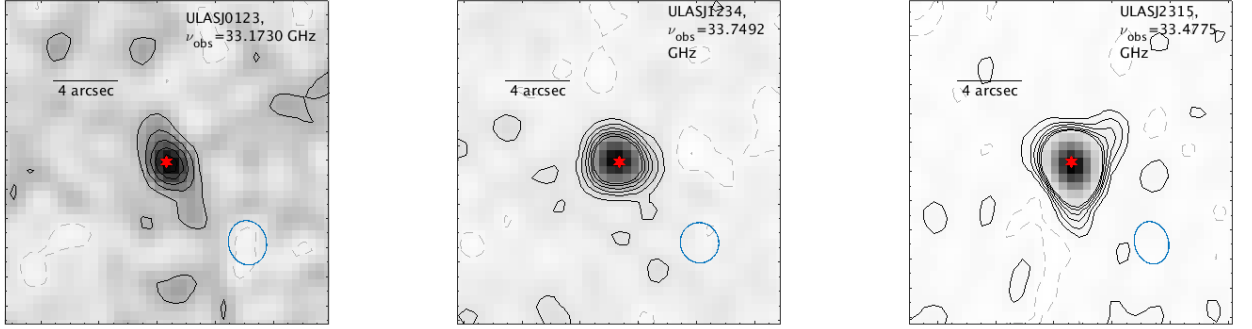
Figure 1. 20 \times 20'' continuum images at \nu_{\text{obs}} \sim 33 GHz produced from the JVLA data for ULASJ0123 (left), ULASJ1234 (middle) and ULASJ2315 (right). The solid and dashed lines represent positive and negative flux contours at intervals of 1.5\sigma . The location of the quasar is marked with a star and the beam size and position angle is indicated in the bottom right-corner of each image. North is up and East is to the right.
