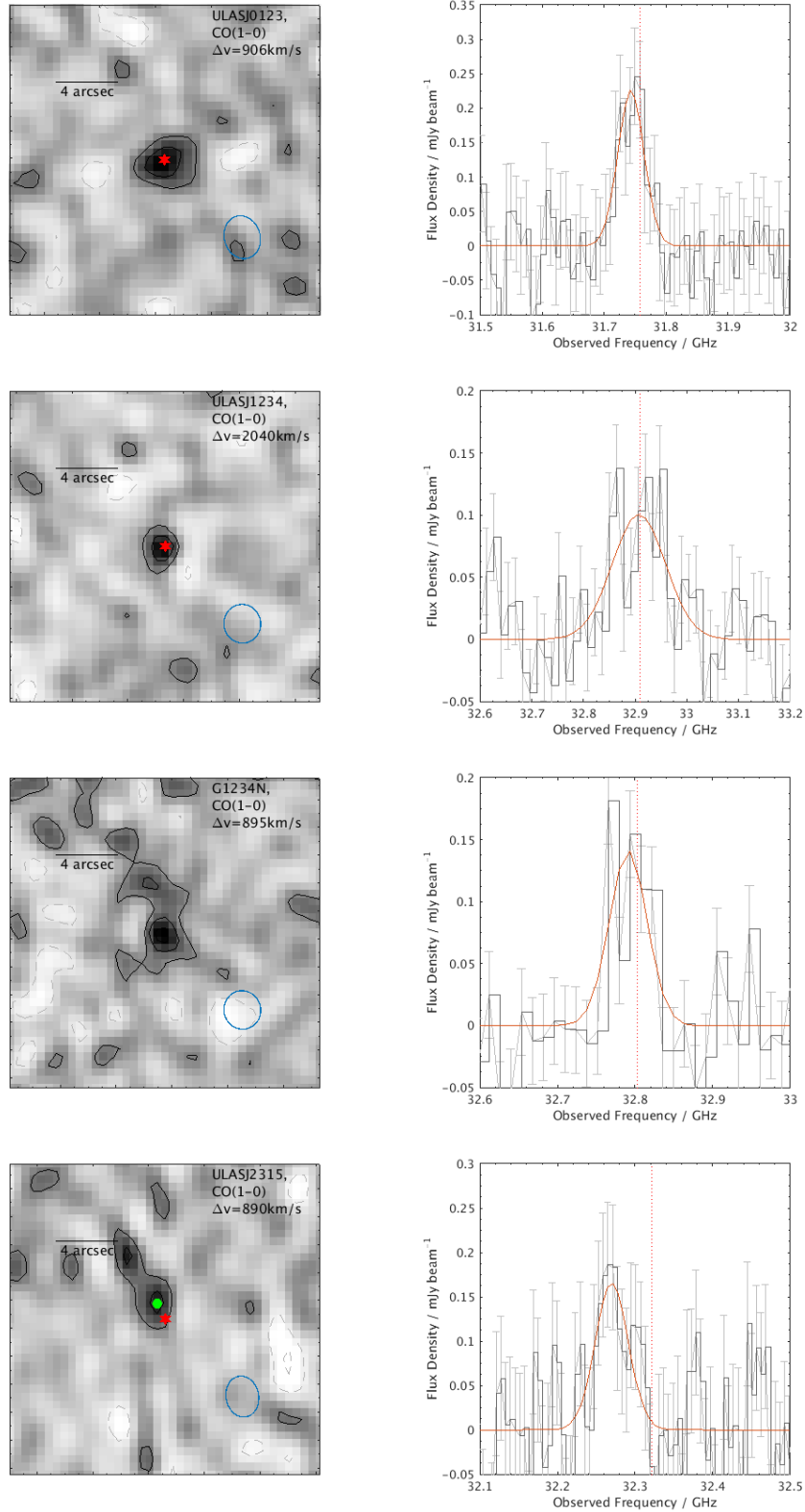
Figure 3. Left: 20 \times 20'' CO(1-0) line maps integrated over \pm FWHM of the line profile corresponding to velocity intervals of \Delta v as indicated in each panel. The solid and dashed lines represent positive and negative flux contours at intervals of 1.5\sigma . The location of the quasars is marked with a star and the beam size and position angle are indicated in the bottom right-corner of each image. North is up and East is to the right. Right: CO(1-0) spectral line profiles together with the best-fit single Gaussian model. Error-bars denote the 1\sigma RMS per channel. Vertical dotted lines mark the expected position of CO(1-0) based on the CO(3-2) derived redshifts for the sources in B17 and Paper II. For ULASJ2315 (bottom panels), the peak of the CO(1-0) emission is spatially offset from the quasar centroid and the CO(1-0) spectrum has therefore been extracted from the position of the green circle. The CO(1-0) line in ULASJ2315 is also shifted in velocity relative to CO(3-2).
