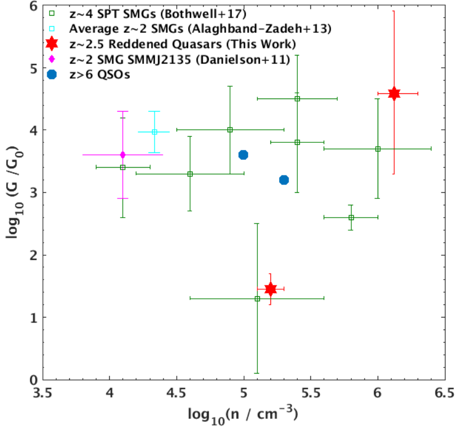
Figure 10. The gas density versus radiation field strength inferred from PDR modelling of our two heavily reddened quasars, ULASJ1234 and ULASJ2315 assuming \zeta=10^{-15}\text{s}^{-1} and A_V=7 mags. These values are compared to both SMGs and quasars from the literature (Alaghband-Zadeh et al. 2013; Danielson et al. 2011; Bothwell et al. 2017; Venemans et al. 2017). In the case of ULASJ2315, we plot constraints from the integrated emission from the QSO and Gal components of the merger. The Bothwell et al. (2017) SMG sample forms the most direct comparison sample to ours, on account of using exactly the same PDR model and model set-up as assumed in this work.
