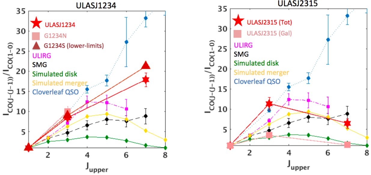
Figure 9. The CO Spectral Line Energy Distributions for all galaxies in the ULASJ1234 (left) and ULASJ2315 (right) systems. G1234N and G1234S are represented by the square and triangle symbols respectively in the left-hand panel, while the GAL component of ULASJ2315 is represented by the square symbols in the right-hand panel. As we did not detect CO(1-0) in G1234S, the triangles are used to represent lower limits on the line ratio for this galaxy. For ULASJ2315 we show integrated line ratios from both components of the merger as well as line ratios assuming all the CO(1-0) emission is coming from the northern companion galaxy. For comparison we also show the SLEDs for Ultraluminous Infrared Galaxies (Papadopoulos et al. 2012), Submillimetre Galaxies (Bothwell et al. 2013), the Cloverleaf quasar (Carilli & Walter 2013) and simulated SLEDs for both high-redshift disk galaxies and mergers (Bournaud et al. 2015) that are designed to reproduce observational data for these kinds of systems.
