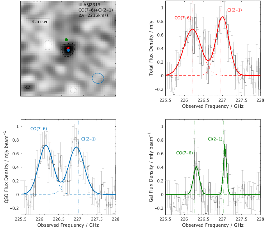
Figure 5. Top Left: 16 \times 16'' CO(7-6)+CI(2-1) line maps integrated over \pm FWHM of both lines in the ULASJ2315 system corresponding to a velocity interval \Delta v = 2236 km/s. The solid and dashed lines represent positive and negative flux contours at intervals of 1.5\sigma . The location of the quasar is marked with a star while the blue and green circles mark the centroids of the two components corresponding to the quasar host and the northern companion inferred from the high angular resolution observations of the CO(3-2) emission in Paper II. North is up and East is to the right. In the top-right we show the spectrum integrated over the entire spatial extent of the source while the bottom two panels show the spectra extracted from the centroids of the two components of the merger. The best-fit model to these line profiles is the sum (solid) of two (dashed) Gaussian profiles. Error-bars denote the 1\sigma RMS per channel. Vertical dotted lines mark the expected positions of these lines based on the CO(3-2) derived redshifts for the sources in Paper II.
