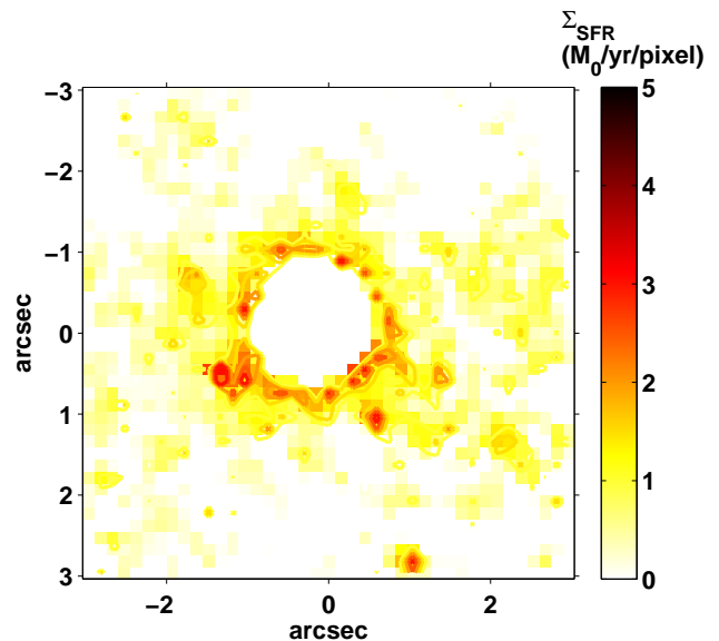
Figure A1. Narrow-band H\alpha emission map in a region of 6 \times 6 arcsec around ULASJ1234+0907 where the H\alpha emission per pixel has been converted to a star formation rate density per pixel. The pixel size is 0.148 arcsec. The image has been smoothed using median filtering over a 2 \times 2 pixel box. The 1\sigma contours can also be seen. From this map, we obtain a 1\sigma limit on the star formation rate density of \Sigma_{\text{SFR}} < 1 M_{\odot} \text{ yr}^{-1} per pixel
