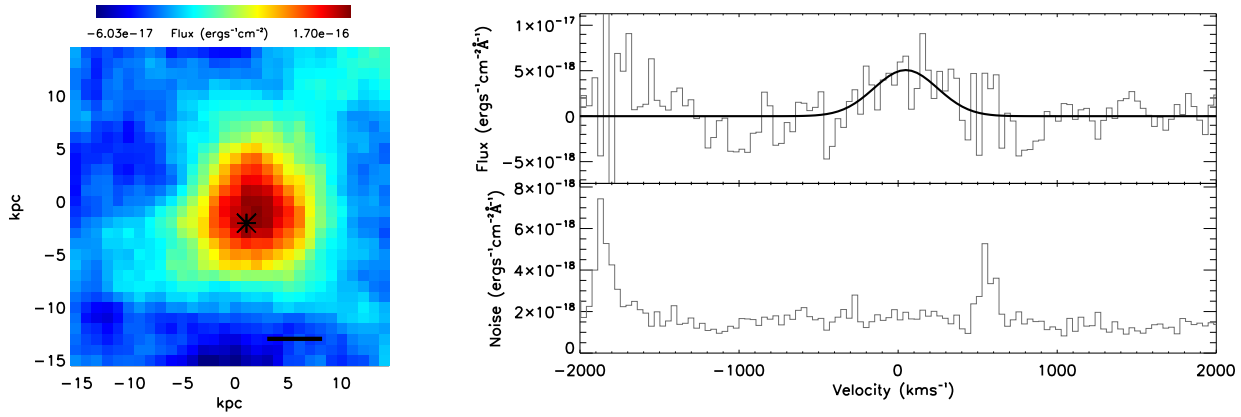
Figure C12. As for C1 for the resolved narrow H \alpha emission in VHSJ2144-0523. A narrow Gaussian profile with a width of \sigma=200 \text{ km s}^{-1} was found to give a better fit therefore the map is created by integrating over \pm 300 \text{ km s}^{-1} ( 1.5\sigma ) and the Gaussian profile overlaid has a width of \sigma=200 \text{ km s}^{-1} . The narrow H \alpha emission is spatially resolved.
