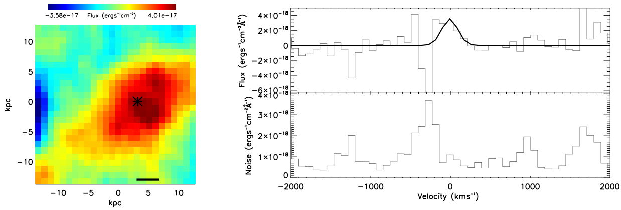
Figure C1. Left: Map of the narrow H\alpha emission in ULASJ1002+0137, created by integrating the profile-subtracted cube from the centre of the narrow line \pm 150 \text{ km s}^{-1} ( 1.5\sigma ). The profile-subtracted cube is made by subtracting the broad line profile (scaled using the maximum likelihood technique) from the spectrum in each binned spaxel. Since we find evidence for extended (spatially resolved) narrow H\alpha emission in this case the spaxels are binned such that each spaxel represents the sum of the surrounding spaxels in a region the size of which maximises the S/N of the detection. The black cross marks the quasar centre and corresponds to the aperture in which the total spectrum has evidence for a narrow Gaussian of width \sigma=100 \text{ km s}^{-1} . We show the FWHM of the PSF-aperture by the black line in the bottom, right-hand corner. Top Right: The total spectrum from the aperture at the quasar centre with the scaled Gaussian overlaid. Bottom Right: The noise spectrum (as detailed in Section 2.1).
