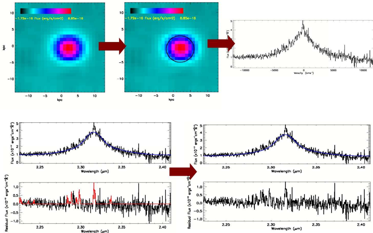
Figure 1. An example sequence (using VHSJ2355-0011) to illustrate the method used to search for narrow H\alpha emission. First we integrate the cube over the broad H\alpha line (from H\alpha-12000 \text{ km s}^{-1} to H\alpha+12000 \text{ km s}^{-1} ) to create an estimate of the PSF. The radius at which the PSF-signal has maximum S/N is determined and the signal from within the radius (the ‘PSF-aperture’) is used to provide the optimal estimate of the broad line profile. We characterise the broad line profile by first fitting a single or double Gaussian profile to the spectrum (blue line). The fit requires that the Gaussian profiles must have FWHMs greater than 1000 \text{ km s}^{-1} . Since it is possible that the narrow component may be spatially coincident with the broad line PSF, and therefore included in this spectrum, the residuals of the initial fit are searched for regions of excess positive flux on scales of > 100 \text{ km s}^{-1} (red line). These regions are then excluded and the fit is recalculated (blue line). This final fit represents the broad line profile to be subtracted from each spaxel region. We re-bin the spaxels such that each spaxel contains the sum of the surrounding spaxels in a region the size of the PSF-aperture. We then subtract the broad profile, using a maximum likelihood technique to scale the profile, from each spaxel region and search the profile-subtracted cube for narrow Gaussian H\alpha emission with \sigma=100 \text{ km s}^{-1} and 200 \text{ km s}^{-1} .
