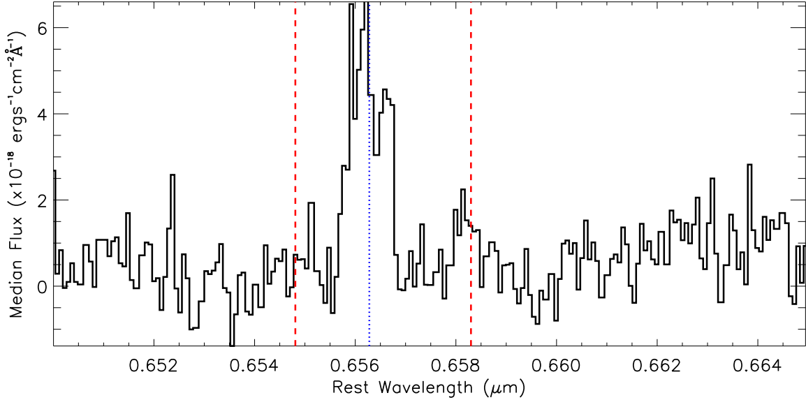
Figure 5. The stacked spectra of 14 detections of narrow H \alpha emission (marked by the blue line) with the position of the [NII] lines marked by the red lines. We do not include the 2 high S/N narrow H \alpha detections (VHSJ1556-0835 and ULASJ2200+0056) as discussed in Section 3.2.3. The ratio of [NII]/H \alpha in the stack is 0.25 \pm 0.08 .
