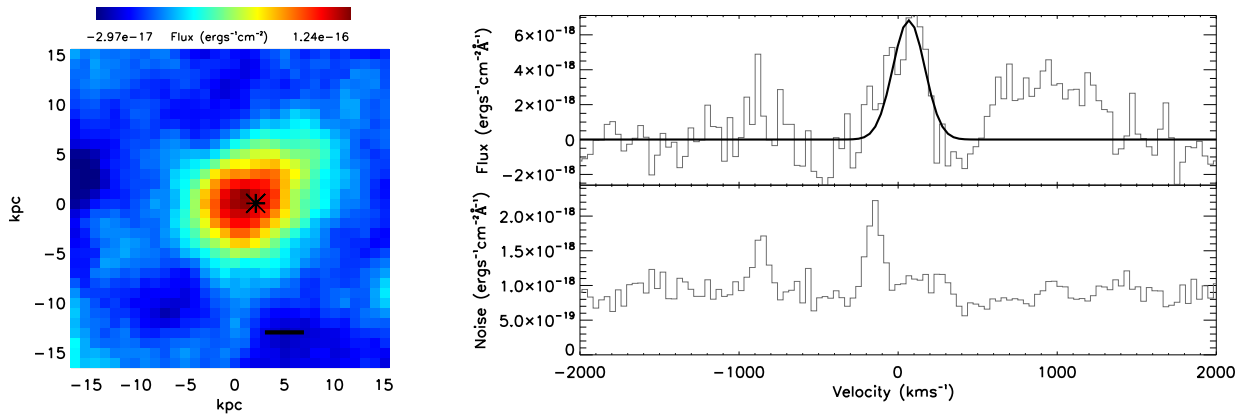
Figure C2. As for C1 for the narrow H\alpha emission in VHSJ1556-0835. Since the narrow H\alpha emission is spatially unresolved the spaxels are binned such that each spaxel represents the sum of the surrounding spaxels in a region the size of PSF-aperture. The black cross marks the quasar centre and corresponds to the PSF-aperture in which the total spectrum has evidence for a narrow Gaussian of width \sigma=100 \text{ km s}^{-1} . We show the FWHM of the PSF-aperture by the black line in the bottom, right-hand corner.
