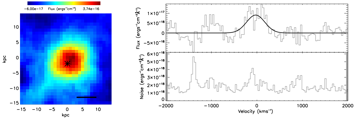
Figure C6. As for C2 for the unresolved narrow H \alpha emission in VHSJ2100-5820. A narrow Gaussian profile with a width of \sigma=200 km s^{-1} was found to give a better fit therefore the map is created by integrating over \pm 300 km s^{-1} ( 1.5\sigma ) and the Gaussian profile overlaid has a width of \sigma=200 km s^{-1} .
