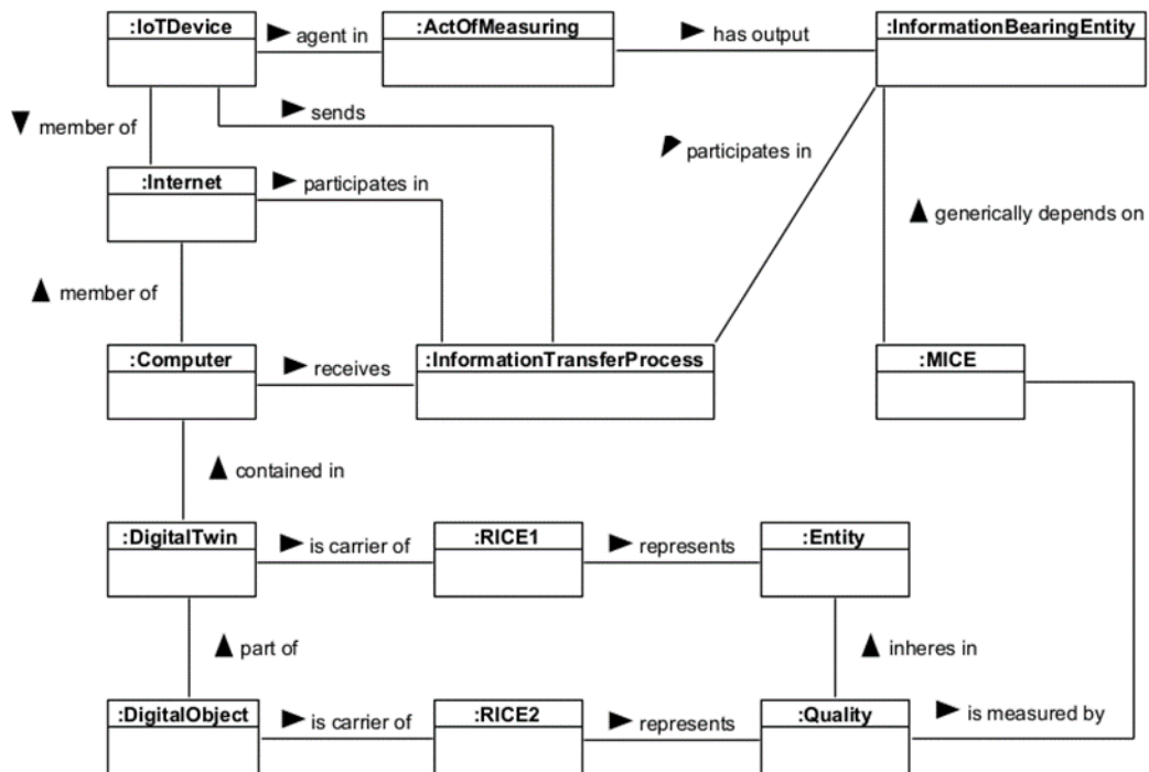
Figure 35. Representing digital twins in CCO. [Acronyms: RICE (Representational Information Content Entity) and MICE (Measurement Information Content Entity).]
