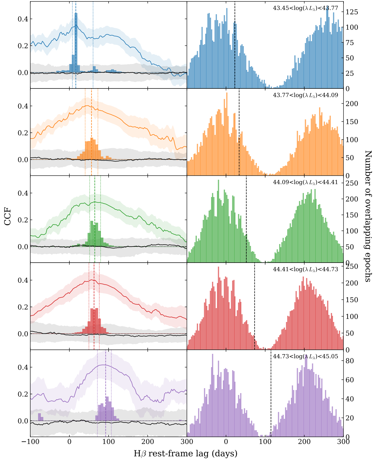
Figure 3. Left column: The coloured solid lines are the stacked cross correlation functions (CCF) for each of the five luminosity bins for the H \beta sample. The colours correspond to the respective bins in Figure 2. The 1 \sigma scatter of the bootstrapped CCF's is shown by the coloured shaded region. The vertical dashed and dotted lines indicate the recovered average lag and its uncertainty, as measured from the bootstrap distribution (coloured histogram). The black solid line and grey shaded area show the mean and 1 \sigma scatter of the CCF's generated using the randomised spectroscopic light curves following the procedure described in §3. Right column: The number of overlapping spectroscopic and photometric epochs as a function of time lag, in total for each source in the corresponding bin. The expected mean lag for the bin is indicated by the black dashed line.
