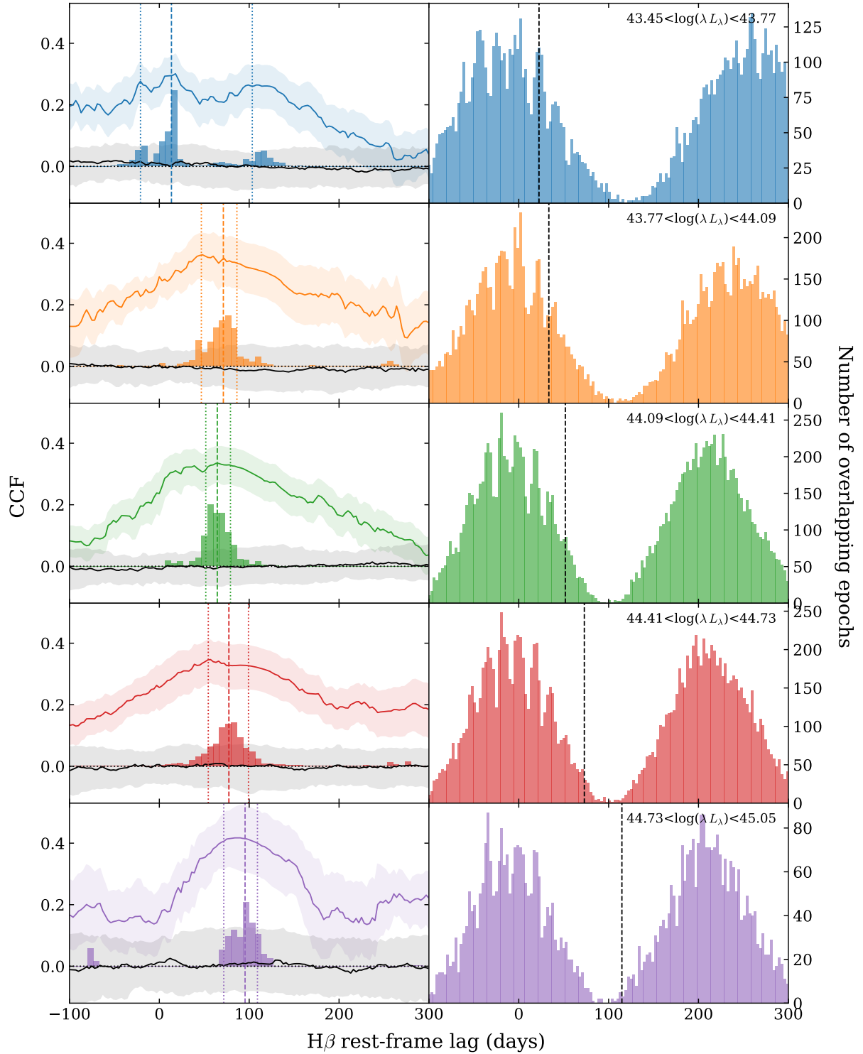
Figure B2. The same as Figure 3 after excluding sources with individual lag recoveries from the stacked sample.
