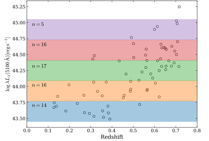
Figure 2. The luminosity bins for the H \beta sample, labelled with the number of binned sources. Within each bin, the standard deviation of the expected lags for the individual sources (measured using the source luminosity and the Bentz et al. (2013) R - L relation for H \beta ) is \sim 10\% of the expected mean lag for the binned sample (measured as the mean of the expected lags for the individual sources).
