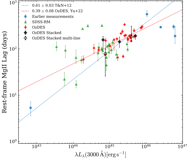
Figure 7. Radius-Luminosity relation for Mg II, with existing individual lag measurements from Metzroth et al. (2006); Lira et al. (2018); Czerny et al. (2019); Zajaček et al. (2020, 2021) and SDSS-RM (Homayouni et al. 2020, gold sample), along with the OzDES individual measurements (Yu et al. 2023), and our stacked average lag measurements. The multi-line average lag measurements are presented in §4.4.
