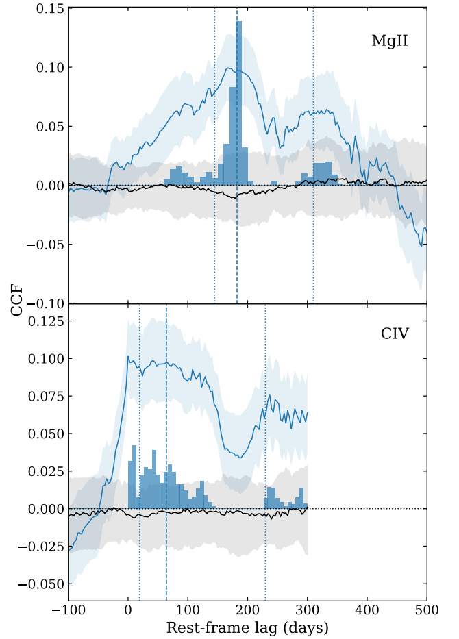
Figure 12. The stacked cross correlation functions (CCF) for the multi-line sample with both Mg II and C IV, comprising 106 AGN.
