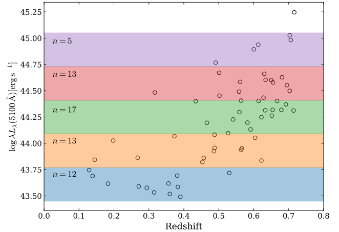
Figure B1. The same as Figure 2 after excluding sources with individual lag recoveries.
