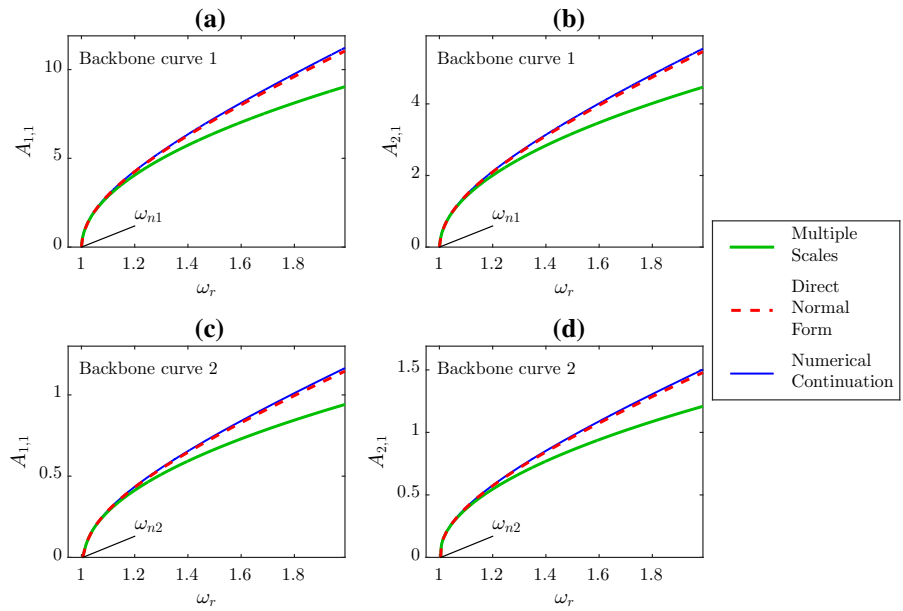
Fig. 4 Fundamental amplitude response curves for the 2DOF system, using \omega_{n1} = 1, \omega_{n2} = 1.005, \kappa_1 = 0.5, and \kappa_2 = 0.05 . Panels a and c show the response of the first mode, and panels b and d show the response of the second mode
