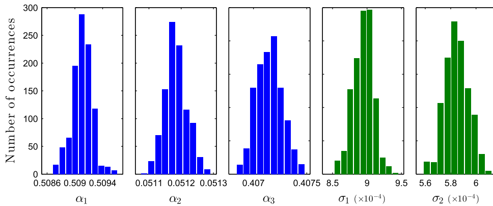
Fig. 6. Histograms, for system 3NL, showing the estimated values of the nonlinear parameters and the standard deviations of the residuals of the expressions describing the backbone curves. The nonlinear parameters, \alpha_1 , \alpha_2 and \alpha_3 , are shown in blue and the standard deviations, \sigma_1 and \sigma_2 , are shown in green. (For interpretation of the references to colour in this figure caption, the reader is referred to the web version of this paper.)
