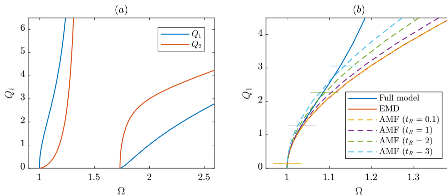
Fig. 6. The backbone curves of the 2-DoF mass–spring model. Panel (a) shows the first and second backbone curves in the projection of the response frequency, \Omega , against the modal amplitudes, Q_1 and Q_2 . Panel (b) shows the first backbone curve of the full model, compared to the backbone curve of five different ROMs. This is in the projection of frequency against the first modal amplitude. The horizontal lines show the maximum value of Q_1 reached in the data used for fitting the AMF-based ROMs.
