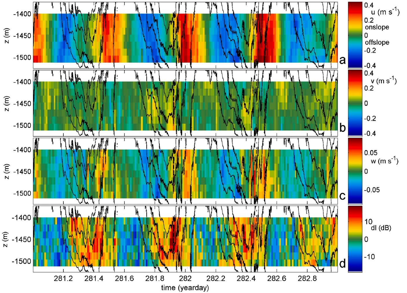
Fig. 5. As Fig. 4 including the black isotherms for reference, but for 900 s sampled current and acoustic measurements by ADCP smoothed vertically over 2 bins for display purposes. The lower 10 m above the seafloor did not provide useful data due to side-lobe contamination. (a) Along-canyon current component. (b) Cross-canyon current component. (c) Vertical current component with different colour-scale compared to a.,b. (d) Acoustic echo amplitude relative to time mean values.
