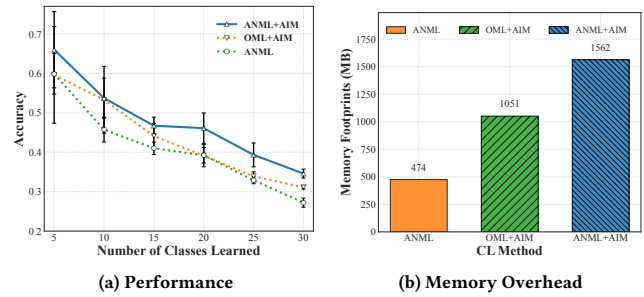
Figure 1: Preliminary analysis of the prior Meta CL methods (i.e., ANML, OML+AIM, ANML+AIM). (a) shows the CL accuracy degradation of the Meta CL methods after learning c number of classes on CIFAR-100 [47]. (b) shows the memory footprint needed to run the Meta CL methods on MiniIma-geNet [95] with a batch size of 8.
