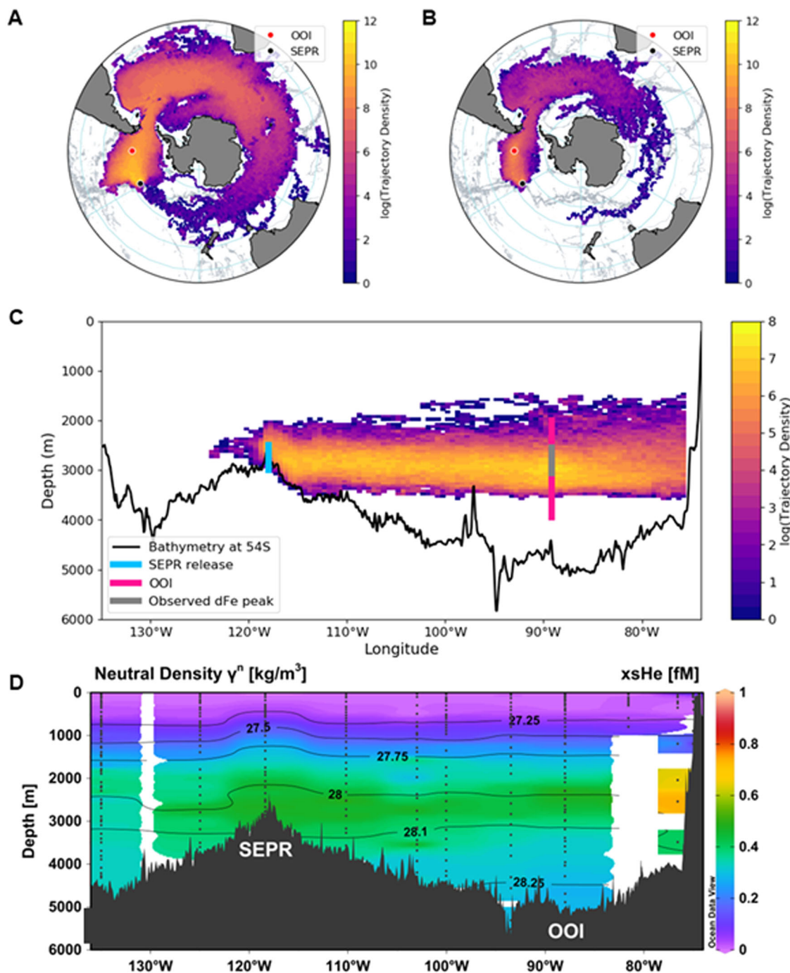
Fig. 3 | Forward-tracking simulations from the Southeast Pacific Rise and coincident xs^3He anomaly. Trajectories of the forward-tracking simulations from the SEPR (A–C) and coincident xs^3He anomaly (D). Trajectories were released between the ridge and 500 m above to mimic a neutrally buoyant hydrothermal plume. A Trajectory density, which indicates the number of instances of trajectories passing into a grid cell (log scale), of all SEPR trajectories. B Trajectory density map of SEPR trajectories that pass within a 0.5° area around the OOI station (red marker). C Depth section of trajectory density for the SEPR trajectories that pass within a 0.5°
