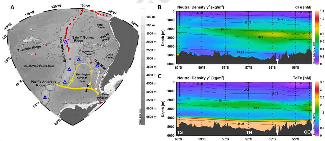
Fig. 1 | Study region and dissolved iron and total dissolvable iron transects. A Study area in the southeast Pacific and Southern Ocean. Red dots are the location of known active vent sites 82 . Lack of exploration means that knowledge of active vent site locations over the region is incomplete. The yellow arrow is the approximate flow of water at 2000–4000 m depth 33 and white arrow is the approximate flow of Southeast Pacific Deep Slope Water 54 . The solid black line is the transect occupied by this study. The white cross is the sampling location of a previous 3 He profile 50 collected in 1993 ~83 km northeast (bearing of 055°) of our northernmost station. Triangles indicate the start locations for forward-tracked trajectory modelling in this
