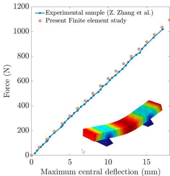
Figure B1. Bending behavior of the fractal lattice (order 6) beam subjected to three-point bending test.
