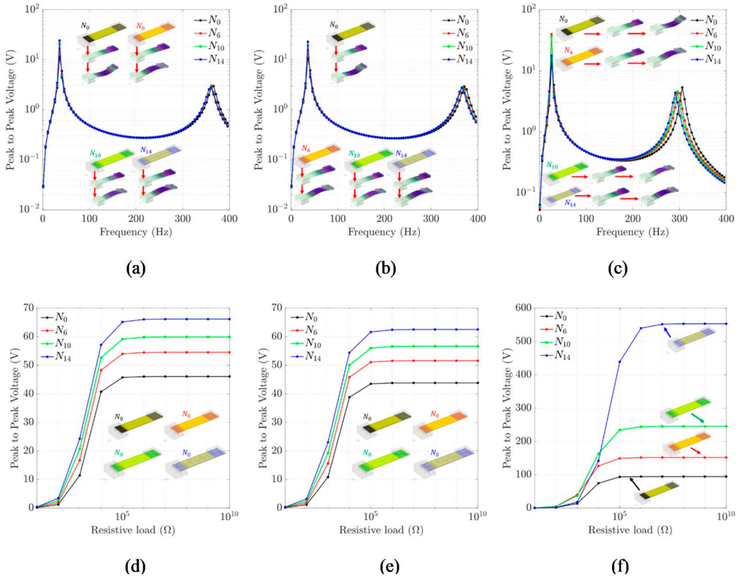
Figure 21. Energy performance of typical (i.e., solid) and fractal PVEHs (with bimorph piezo configurations in series connection) in terms of output peak-to-peak closed-circuit voltage where the substrate layer is made of: (a) Aluminum (b) CFRP (c) Steel. Note that frequency responses of the output voltage are recorded across 1 k \Omega load resistance in all three cases. Later the same voltage at 1st resonance zone is further optimized through a load dependency study in the range of 1 to 10 7 k \Omega . Load dependency study in case of substrate layer made of (d) Aluminum (e) CFRP (f) Steel. Note that the finite element analysis for all instances here considers a fixed tip mass and no variable masses. All three fractal beams are made of four fractal unit cells with a fixed slit width of 0.625 mm. However the overall dimension of each fractal lattice (beam) is kept the same as the prior normal solid beams i.e., 25 \times 100 \times 0.5 mm.
