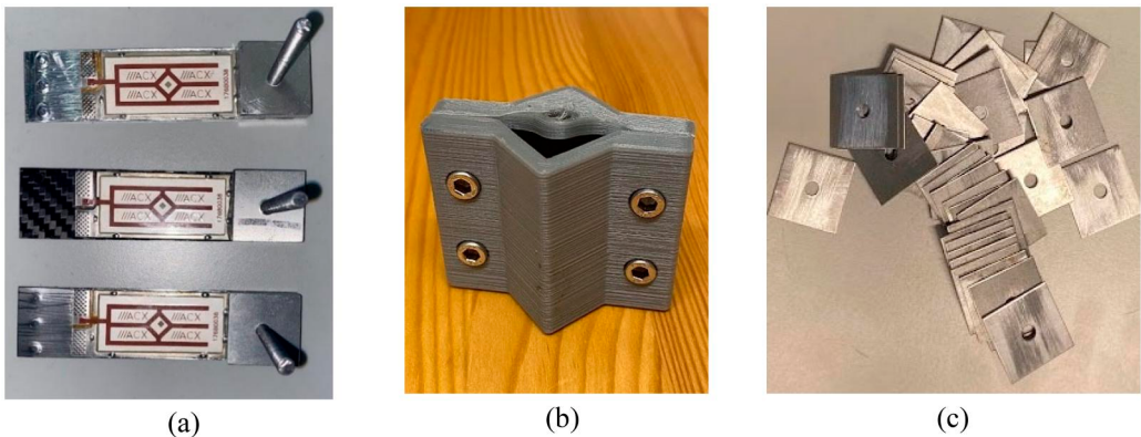
Figure 2. (a) Beams used in experiments. Aluminum (top), CFRP (middle), Steel (bottom) (b) 3D printed hole jig (c) Variable mass steel plates.
