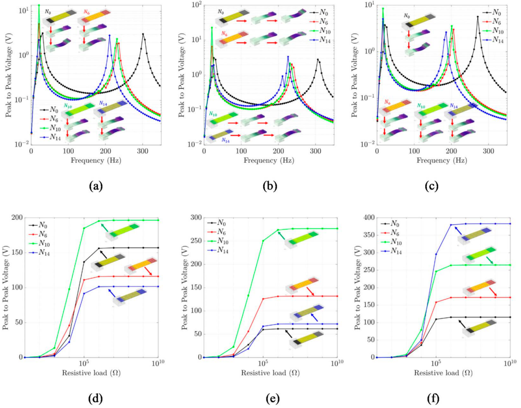
Figure 20. Energy performance of typical (i.e., solid) and fractal PVEHs (with unimorph piezo configurations) in terms of output peak-to-peak closed-circuit voltage where the substrate layer is made of: (a) Aluminum (b) CFRP (c) Steel. Note that frequency responses of the output voltage are recorded across 1 \text{ k } \Omega load resistance in all three cases. Later the same voltage at 1st resonance zone is further optimized through a load dependency study in the range of 1 to 10^7 \text{ k } \Omega . Load dependency study in case of substrate layer made of (d) Aluminum (b) CFRP (c) Steel. Note that the finite element analysis for all instances here considers a fixed tip mass and no variable masses. All three fractal beams are made of four fractal unit cells with a fixed slit width of 0.625 \text{ mm} . However the overall dimension of each fractal lattice (beam) is kept the same as the prior normal solid beams i.e., 25 \times 100 \times 0.5 \text{ mm} .
