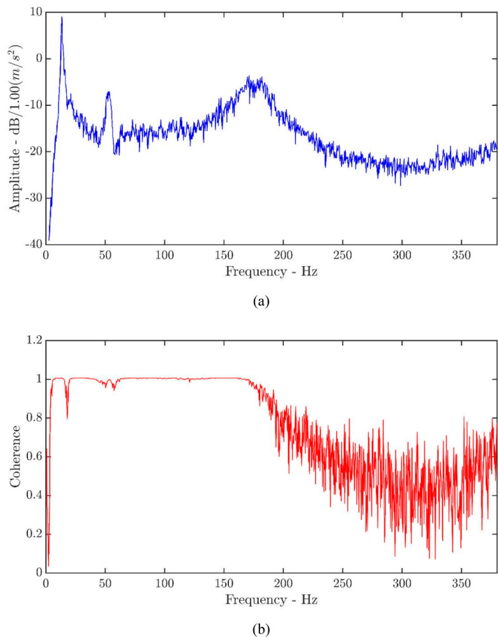
Figure A2. (a) Auto spectrum graph for steel beam with no added (b) Coherence graph for steel beam with no added mass.
