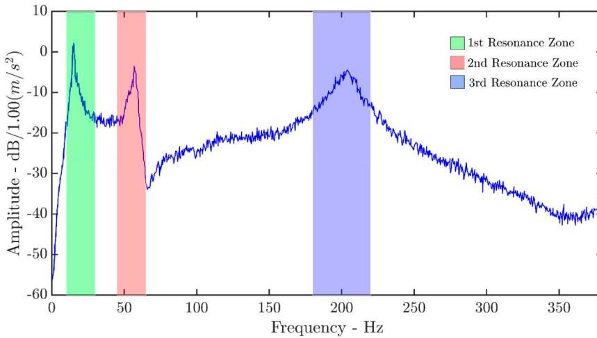
Figure 9. Auto spectrum graph for an aluminum beam with no added external tip mass.
