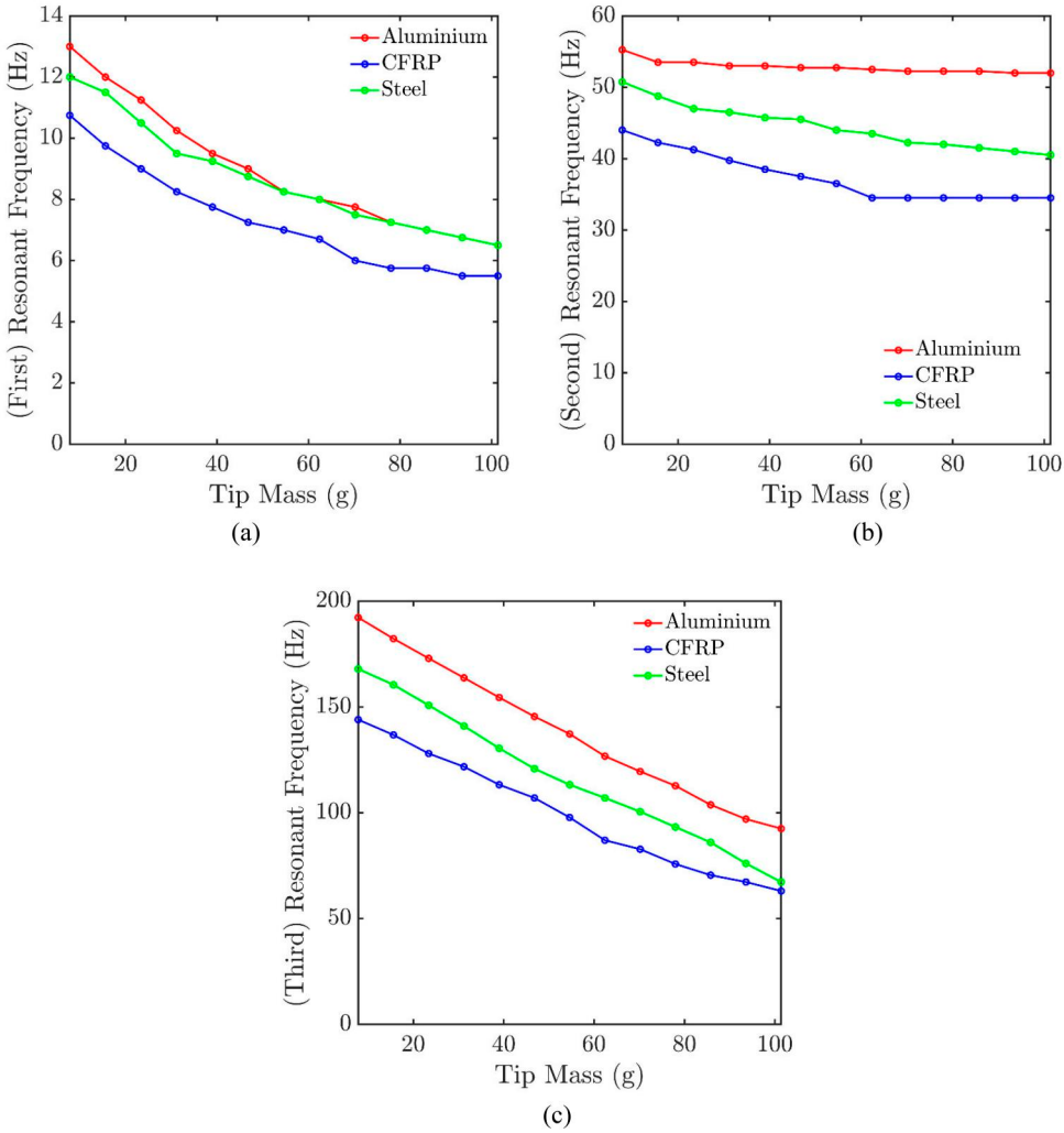
Figure 15. (a) Tip mass dependence of first resonant frequency (b) Tip mass dependence of second resonant frequency (c) Tip mass dependence of third resonant frequency.
