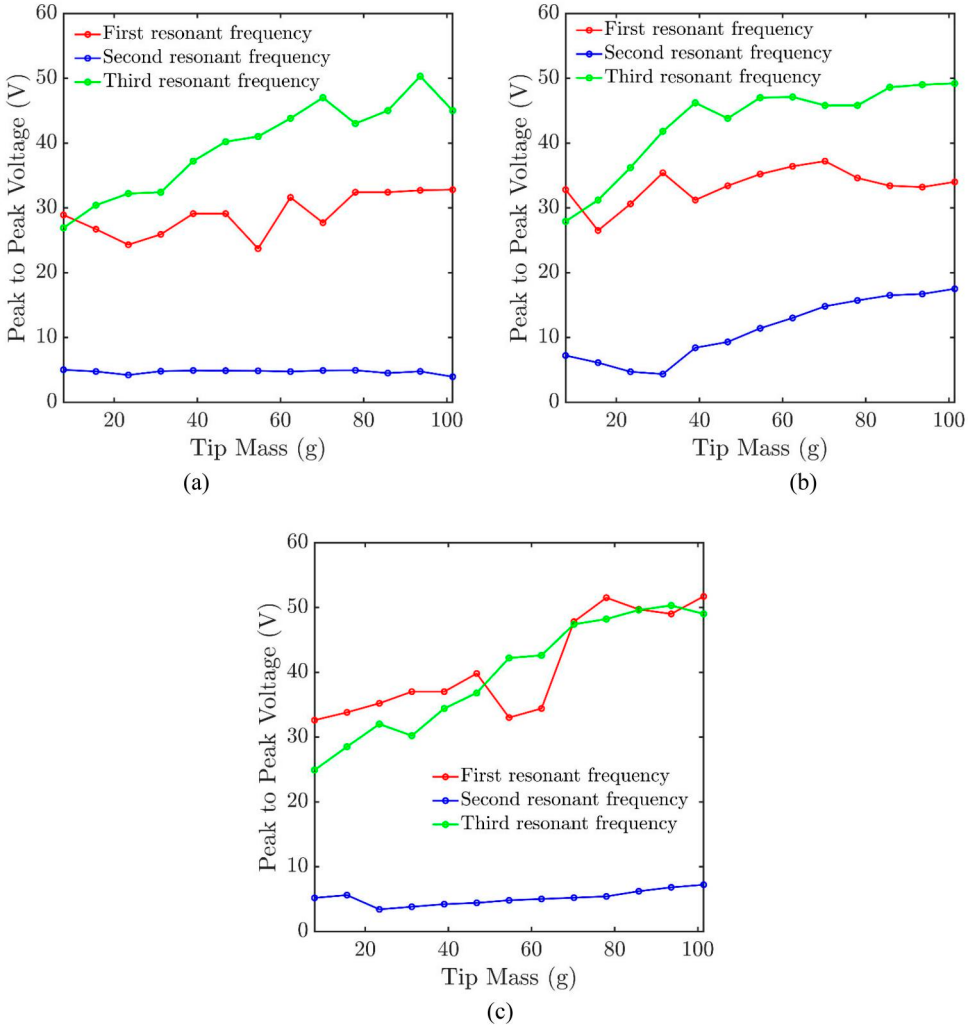
Figure 14. (a) Tip mass dependence of Aluminum beam open circuit voltage (b) Tip mass dependence of Steel beam open circuit voltage (c) Tip mass dependence of CFRP beam open circuit voltage.
