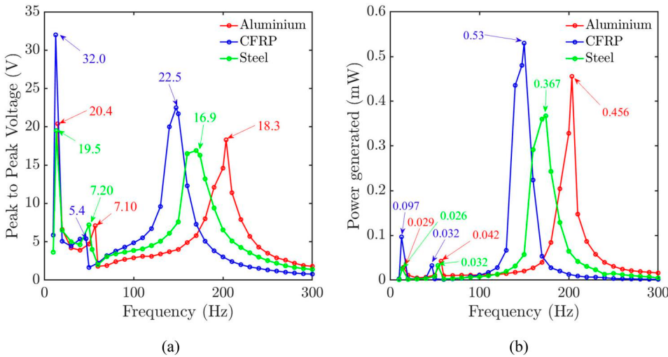
Figure 13. (a) Open circuit measurement of peak-to-peak AC voltage against vibration frequency. (b) Closed circuit measurement of AC power generated against vibration frequency.
