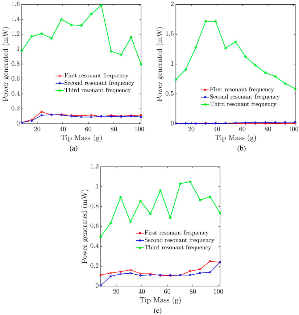
Figure 16. (a) Tip mass dependence of Aluminum beam AC power (b) Tip mass dependence of Steel beam AC power (c) Tip mass dependence of CFRP beam AC power.
