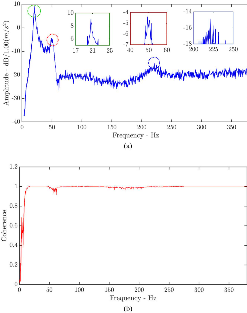
Figure 8. (a) Auto spectrum graph for simple beam calibration experiment (b) Coherence graph for simple beam calibration experiment.
