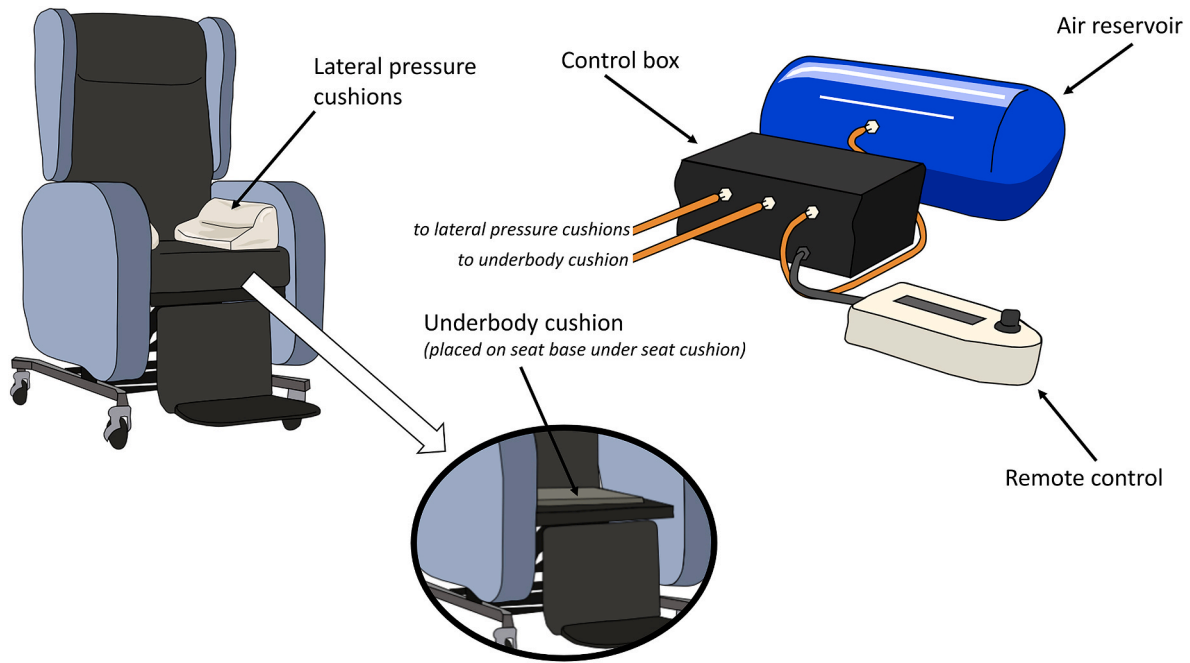
Fig. 1. The lateral pressure device, including lateral cushions, an underbody cushion, control box, remote control, and an air reservoir.
