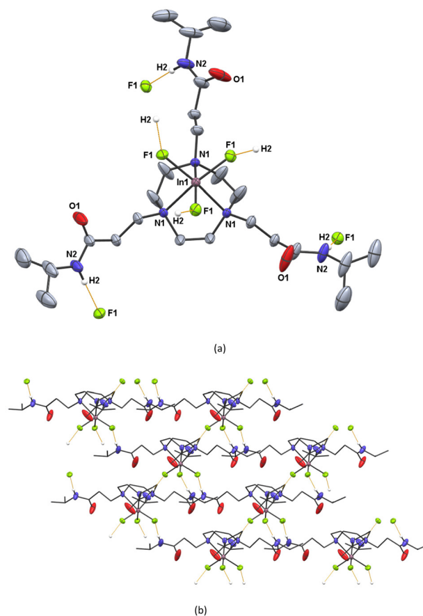
Fig. 4 (a) View of the structure of [InF 3 (L 2 )] showing the atom numbering scheme. H atoms are omitted for clarity. Ellipsoids on In, F, N and O are drawn at the 50% probability level. Selected bond lengths (Å) and angles (°): In1–F1 2.071(2), In1–N1 2.299(3), F1–In1–F1 = 97.99(8), N1–In1–N1 = 78.04(10); (b) view down the a -axis showing the intermolecular F...HN hydrogen bonding contacts.
