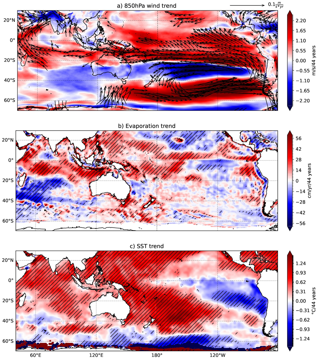
Figure 3. (a) Trend in JJAS 850 hPa wind (colors –speed (m s -1 /44 years)) from ERA5. The arrows are plotted only if at least a component of the wind is statistically significant at the 95% confidence level. (b) Trend in JJAS oceanic evaporation rate (cm ann -1 /44 years) from OAflux. (c) Trend in JJAS SST (°C/44 years) from HadISST1. The hashed regions indicate values that are significant at the 95% confidence level.
