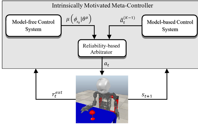
Fig. 4. Intrinsicly Motivated Meta-Controller (IM2C): At each time step t , the learning progress is checked. If greater or equal to zero, the meta-controller queries the model-based control system for an action \hat{a}_t^{(K-1)} , which is the output of the plan optimization (Section 2.2). Otherwise, the meta-controller queries the model-free control system for an action \mu(\phi_{s_t}|\theta^\mu) , which is the output of the actor network. The selected action is then sent to the environment with exploration noise, and the environment returns the next state s_{t+1} and extrinsic reward r_t^{ext} .
