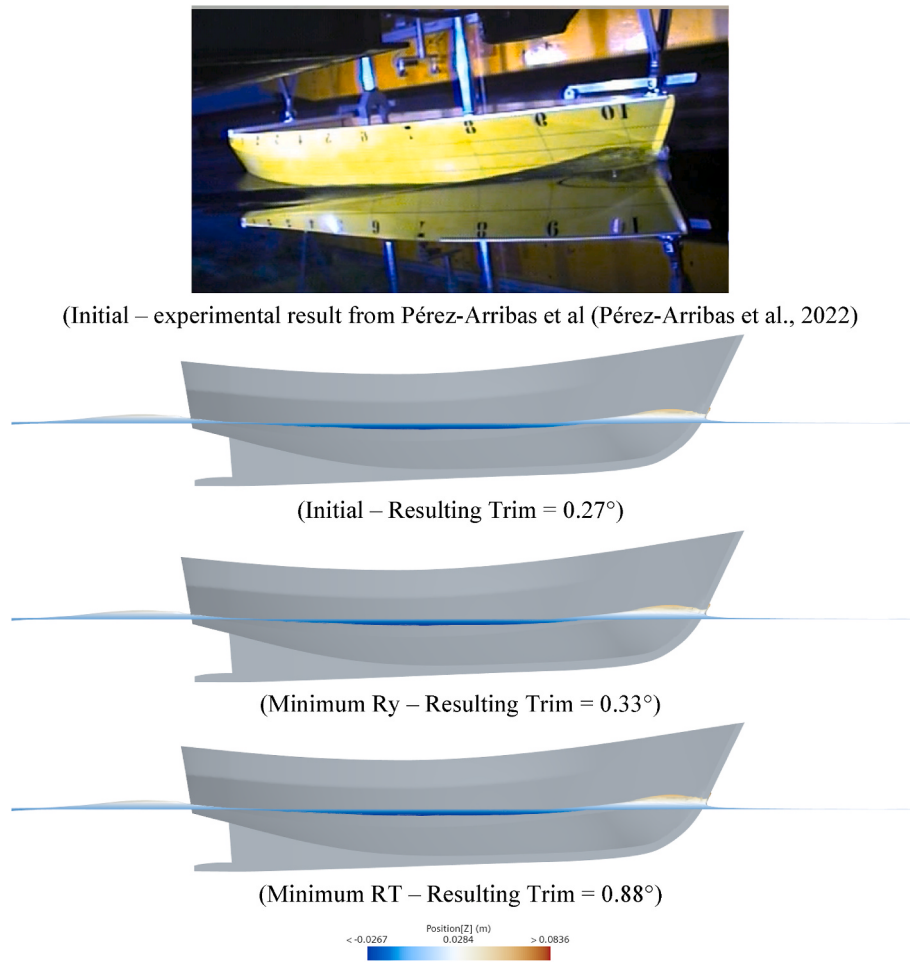
Fig. 7. The visualisation of free surface elevation on hull.
