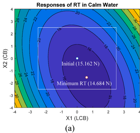
Fig. 9. The Comparison of Response Surface Result for RT Influenced by LCB and CB with the constraints
