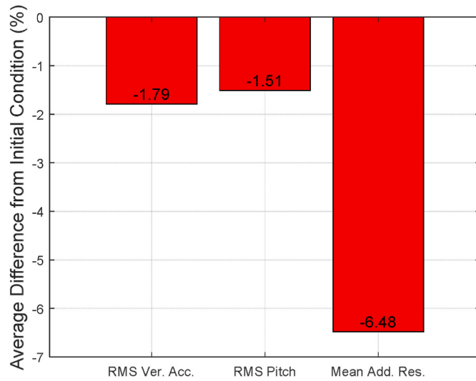
Fig. 16. The comparison of seakeeping performance.
