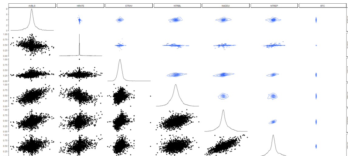
Figure 1 Scatter plots and densities for each pair of variables as well as univariate distributions
