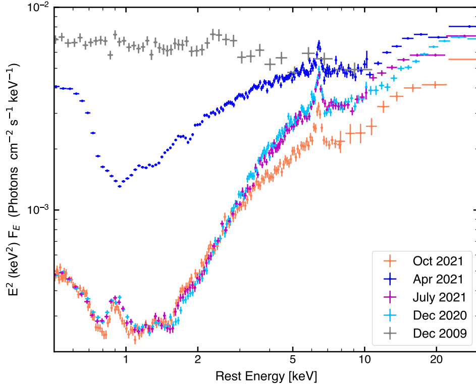
Figure 2. Flux density multiplied by E^2 for the four XMM-Newton+NuSTAR epochs from the prime AGN STORM 2 X-ray campaign. For comparison, we show the archival XMM-Newton observation from December 2009 (Winter et al. 2011) in gray. There is significant variability in the soft X-rays (due to the ionized obscurer) as well as changes in the hard X-ray emission indicative of intrinsic variability in the corona. The 2021 Apr observation, in blue, is the focus of this paper.
