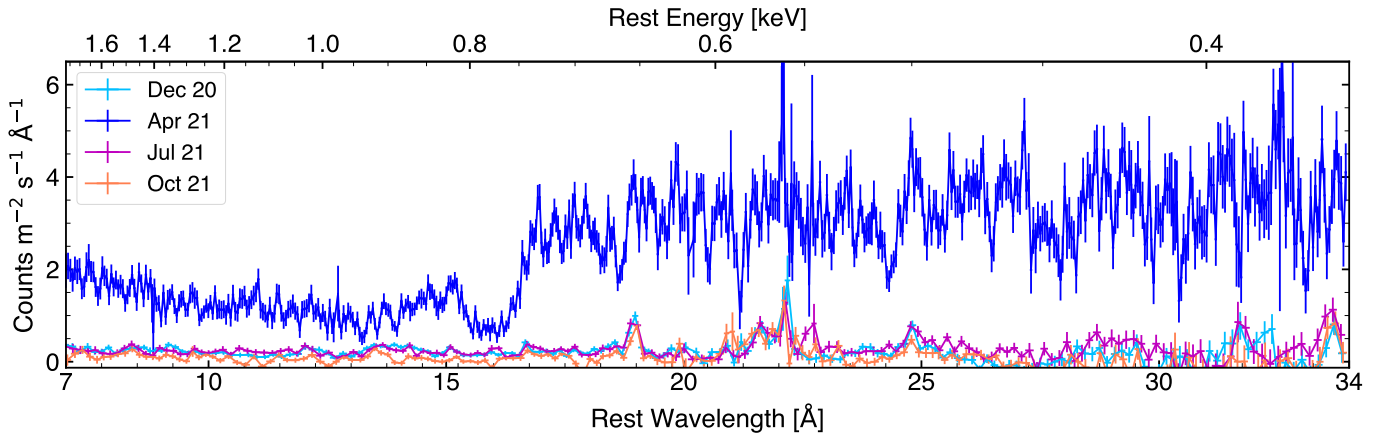
Figure 3. The stacked RGS spectra from the four epochs. The 2021 Apr high-flux observation (blue) shows clear absorption troughs and is the subject of this paper. All the observations are binned using ‘optimal binning’ (Kaastra & Bleeker 2016). The 2020 Dec, 2021 Jul, and 2021 Oct RGS spectra are shown in light blue, purple, and orange, respectively. These epochs are lower flux and show clear emission lines (Zaidouni et al., in prep.). These three observations are further binned by a factor of 3 for visualization purposes.
