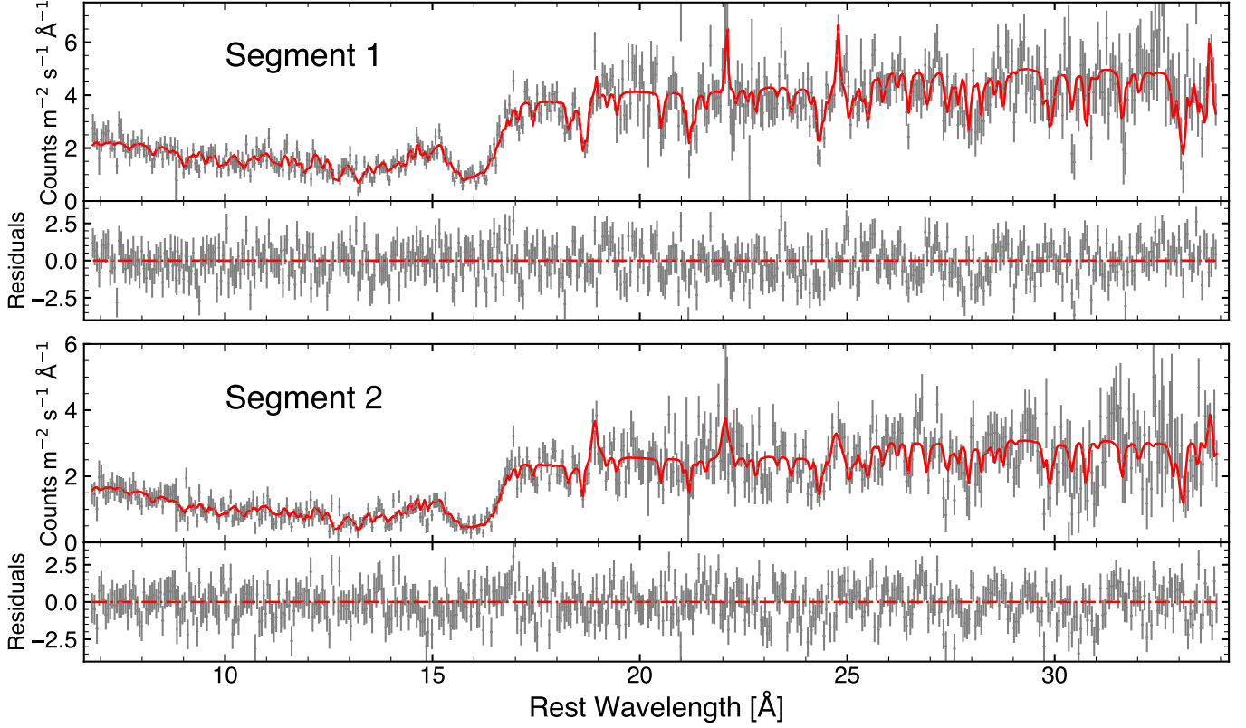
Figure 13. The RGS spectra for Segment 1 (top panel) and Segment 2 (bottom panel) with the best fitting model overlaid in red. The residuals are calculated as “(model-data)/error”.
