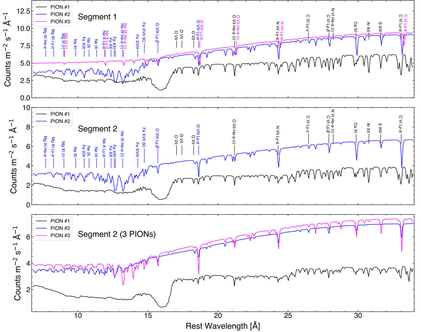
Figure 7. The contribution of each of the PION photoionization model components to the overall fit for Segment 1 ( t < 60 ks, top panel), and Segment 2 ( t > 60 ks, middle panel). The bottom panel shows the scenario where a statistically significant, but redundant PION component is added to the fit of Segment 2. The models are in the form of “(pow \times etau \times etau + bb + dbb + refl) \times pion” which we achieve by setting the covering fraction of the other PION components to zero. For both Segments 1 and 2, PION 1 (black) is the lowest ionization component, fitting largely the long wavelength lines and the iron UTA, while PION 2 (blue) is a higher ionization component, modeling largely the shorter wavelength lines. PION 3 (pink) accounts for the asymmetry in the line shapes of Segment 1 (see text for details).
