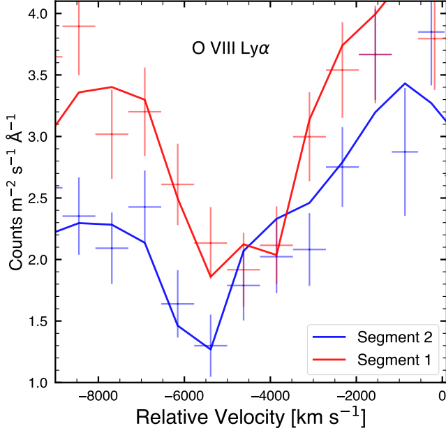
Figure 8. The O VIII Ly \alpha from Segment 1 ( t < 60 ks, red points) and Segment 2 ( t > 60 ks, blue points) with the best-fitting models. This is an example of the enhanced red wing present in Segment 1 and not Segment 2.
