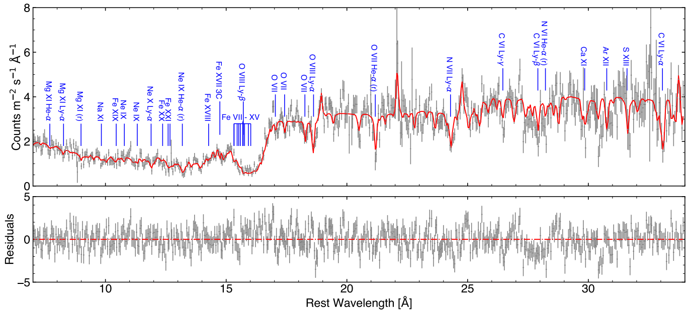
Figure 6. The time-averaged RGS spectrum with the best fitting model overlaid in red. A subset of the absorption lines are labeled at their blue-shifted wavelengths. The residuals are calculated as “(model-data)/error”.
