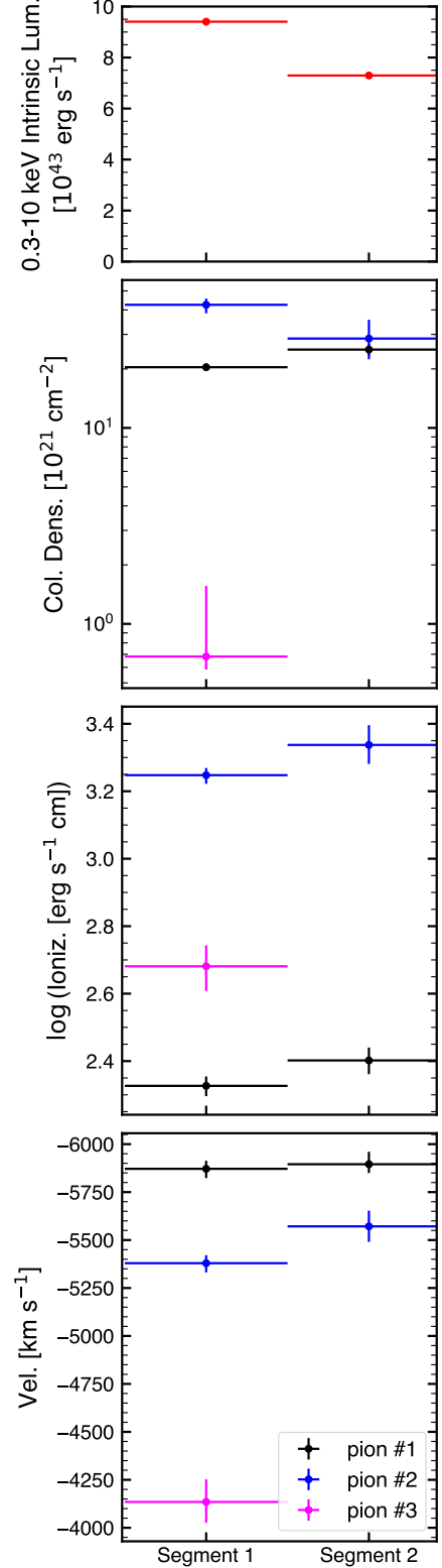
Figure 10. The evolution of key obscurer parameters between the first and second half of the observation. The top panel shows the intrinsic luminosity (absorption corrected) between 0.3 and 10 keV. The rest of the panels show the best-fitting values of the column density, ionization, and outflow velocity for each segment (values from Table 2).
