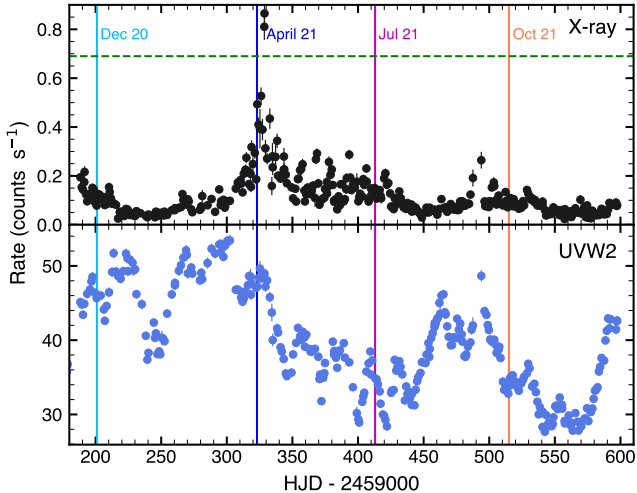
Figure 1. The AGN STORM 2 Swift XRT and UVW2 light curves from 2020 Dec to 2022 Feb (Cackett et al. 2023). Vertical lines indicate when the XMM-Newton and NuSTAR observations were conducted. The green horizontal line indicates the anticipated count rate based on the mean flux of an archival Swift campaign (Morales et al. 2019). During the AGN STORM 2 campaign, the source was largely obscured, with a mean Swift/XRT count rate below 0.2 \text{ counts s}^{-1} , except for a high flux state in 2021 Apr. Our second XMM-Newton and NuSTAR observation serendipitously took place during 2021 Apr.
