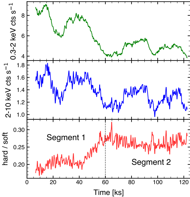
Figure 4. The XMM-Newton EPIC-pn soft band (0.3–2 keV; top panel) and hard band (2–10 keV; middle panel) light curves in 100 s bins along with the corresponding hardness ratio (hard/soft) for the 2021 Apr observation. The spectrum hardens significantly at \sim 60 ks, and the dotted black line delineates the division into two segments for the time-resolved analysis.
