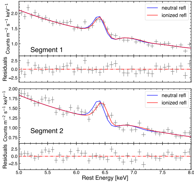
Figure 9. The region around the Fe K alpha emission line from the EPIC-pn instrument data. We overlay the best fit model in red. There are no strong absorption features in this energy band, but we find that the data prefer a mildly ionized reflection model over a neutral reflection model (blue), particularly in Segment 2 when the spectrum is harder (see Table 2 for the parameter values).
