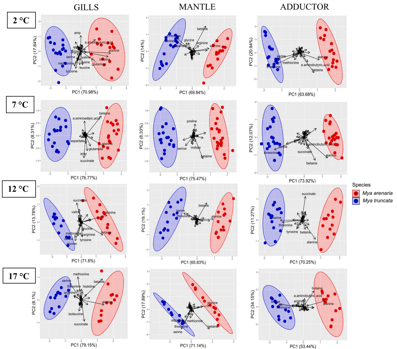
Fig. 2. Principal component analyses (PCA) plots displaying the PC1 and PC2 of the targeted metabolome (42 metabolites) comparing the gills, mantle, and muscle tissues of M. arenaria and M. truncata at all four common temperatures (2, 7, 12, and 17 °C). Points represent individual clams.
