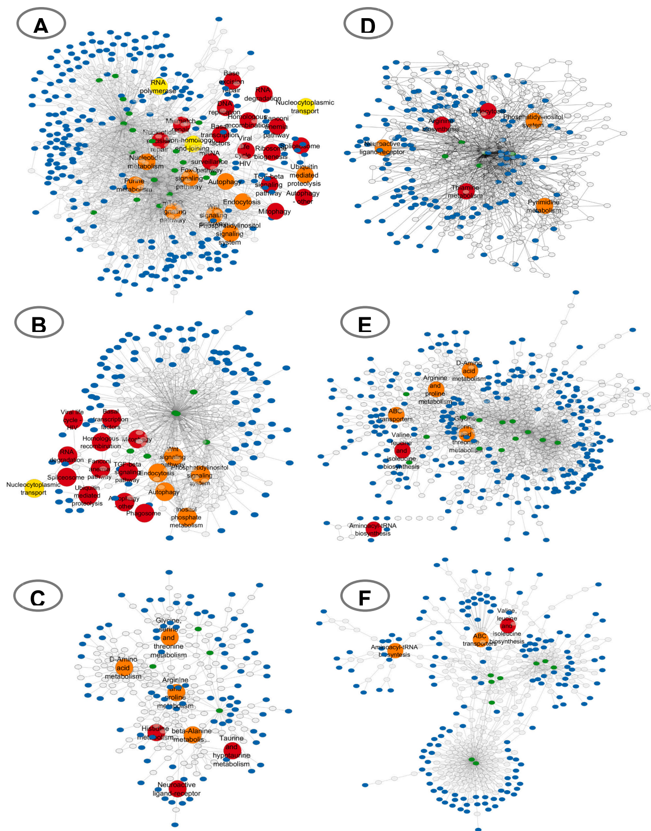
Fig. 4. Pathway analyses results showing the significant pathways expressed at the upper temperature treatment (relative to 7 °C) in the gills, mantle, and muscle tissues of M. arenaria (A, B, and C, respectively) and M. truncata (D, E, and F, respectively) based on a knowledge-based network and diffusion algorithm ( FELLA ). Nodes are either compounds, enzymes, reactions, modules or pathways. Terminal nodes are blue; most connected (> 10) nodes are green; most connected (>10) pathways are red; pathways are orange; and least connected (1) pathways are yellow. Pathways were labeled with text.
