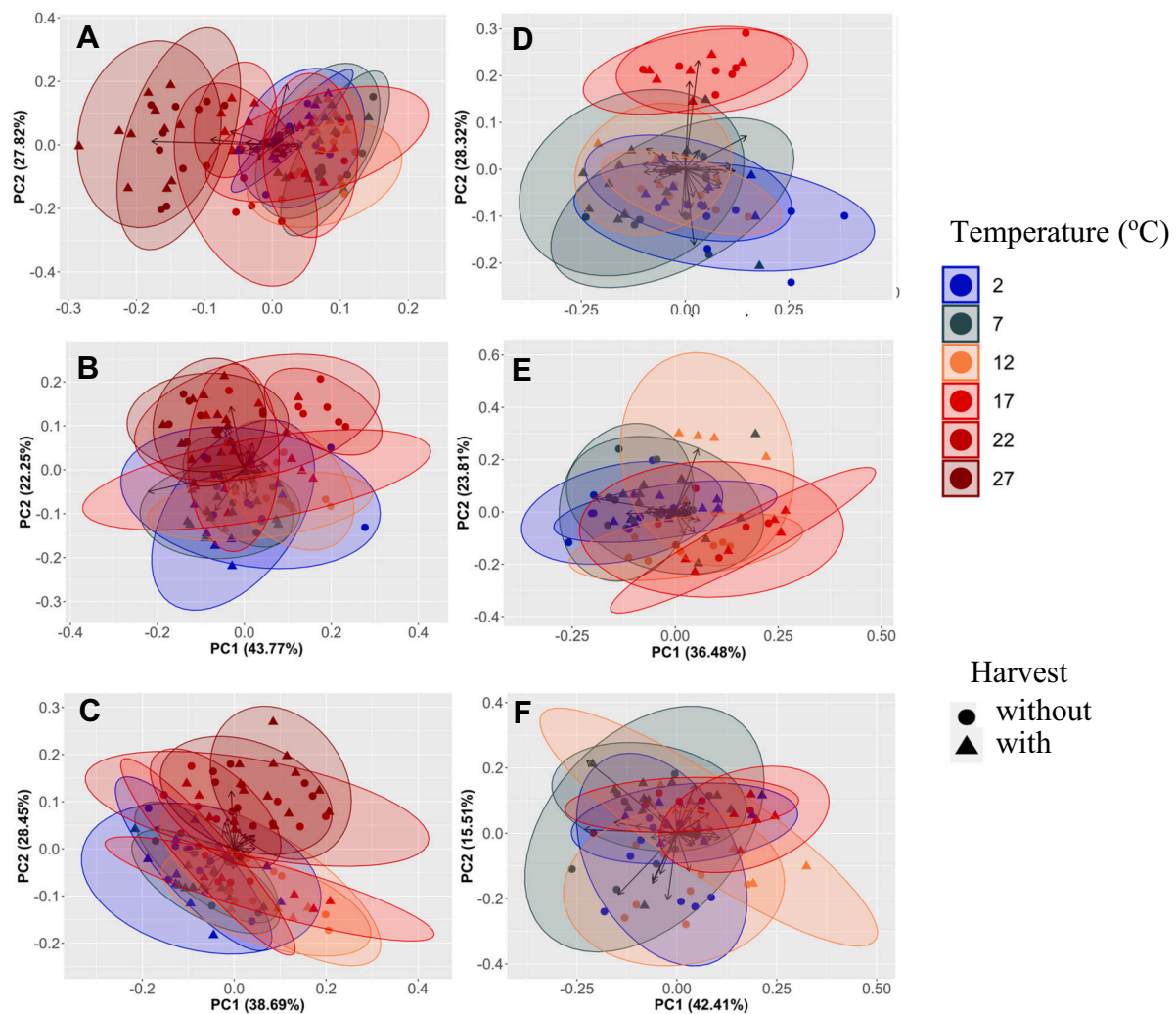
Fig. 3. PCA plots displaying the PC1 and PC2 of the targeted metabolome (42 metabolites) for different temperature treatments in the gills, mantle, and muscle tissues of M. arenaria (A, B, and C) and M. truncata (D, E, and F). Each plot displays the grouping variable temperature (2, 7, 12, 17, 22, and 27 °C, if available) and harvest (with, without). Points represent individual clams.
