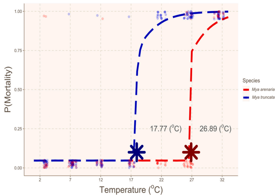
Fig. 1. Probability mortality curves predicted for temperatures ranging between 2 and 32 °C in Mya arenaria and Mya truncata . Curves and breakpoints (•) were estimated according to multiple change point (mcp) analysis ( N = 656 ). Points represent individual clams.
