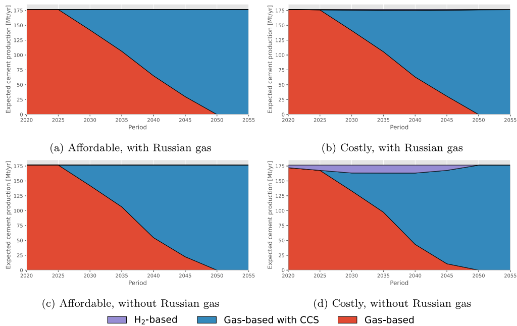
Fig. 5. Evolution of European cement clinker production.
